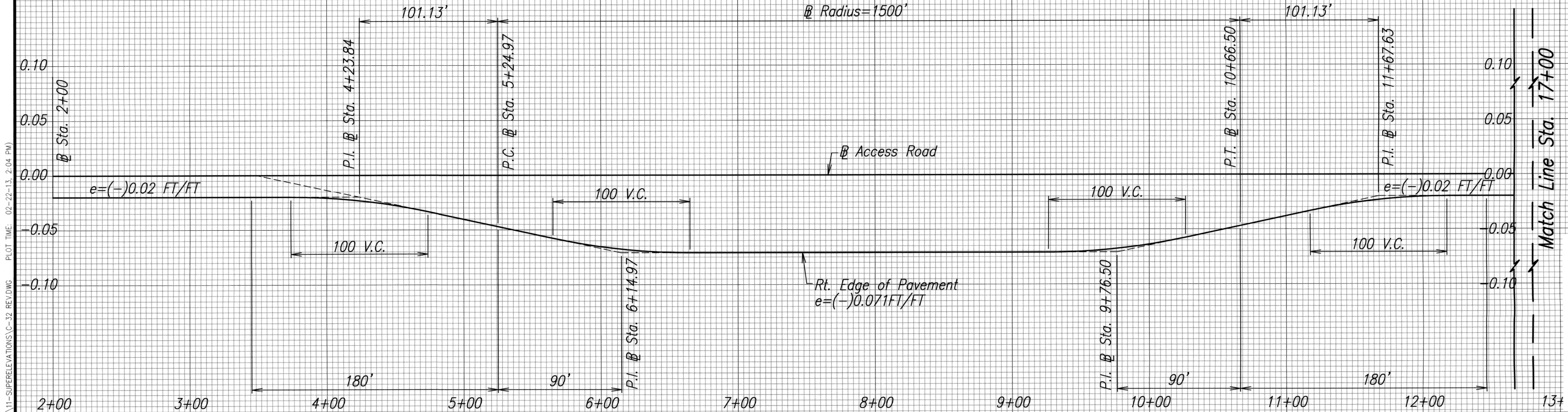
SUPERELEVATION DIAGRAM – MAIN ACCESS ROAD (OUTBOUND LANES) SCALE: HORIZ. 1"=40' VERT. 1"=0.05 FT/FT
