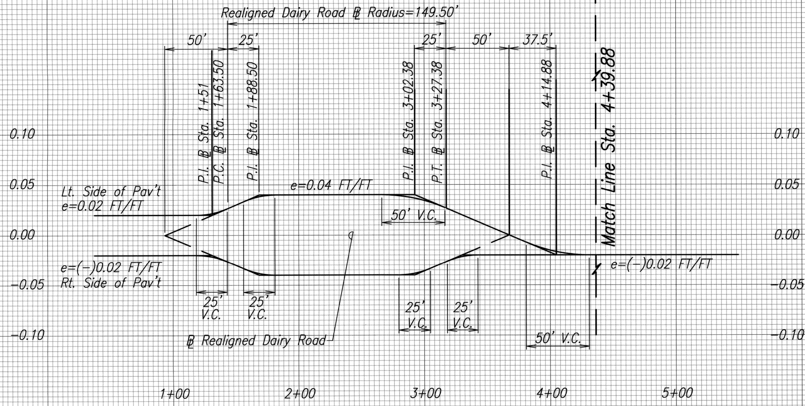
SUPERELEVATION DIAGRAM - REALIGNED DAIRY ROAD SCALE: HORIZ. 1"=40' VERT. 1"=0.05 FT/FT
