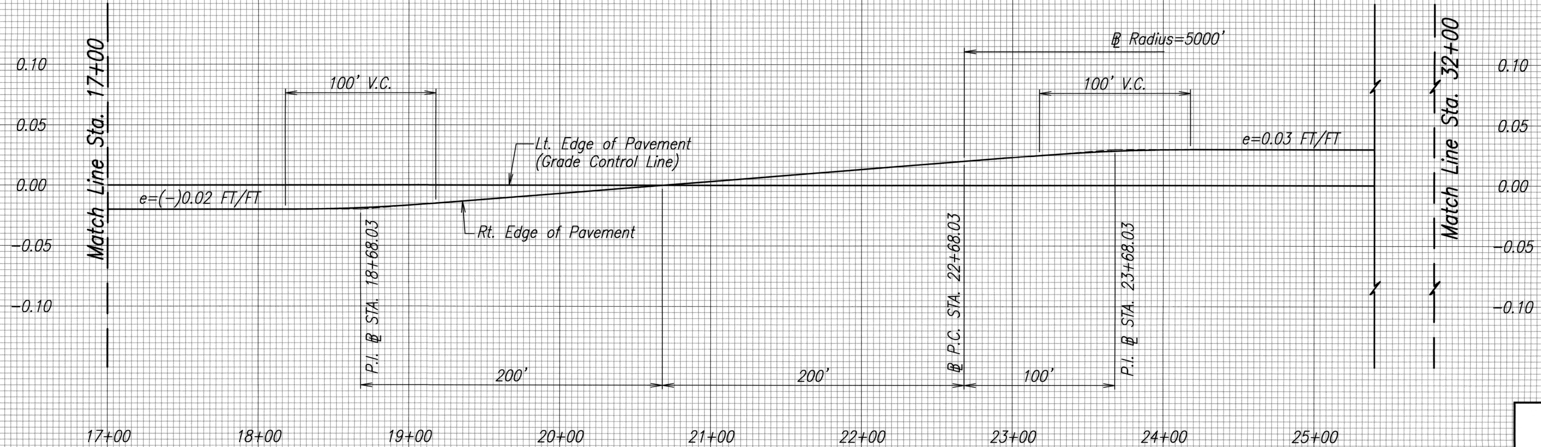
SUPERELEVATION DIAGRAM – MAIN ACCESS ROAD (INBOUND LANES) SCALE: HORIZ. 1"=40' VERT. 1"=0.05 FT/FT
