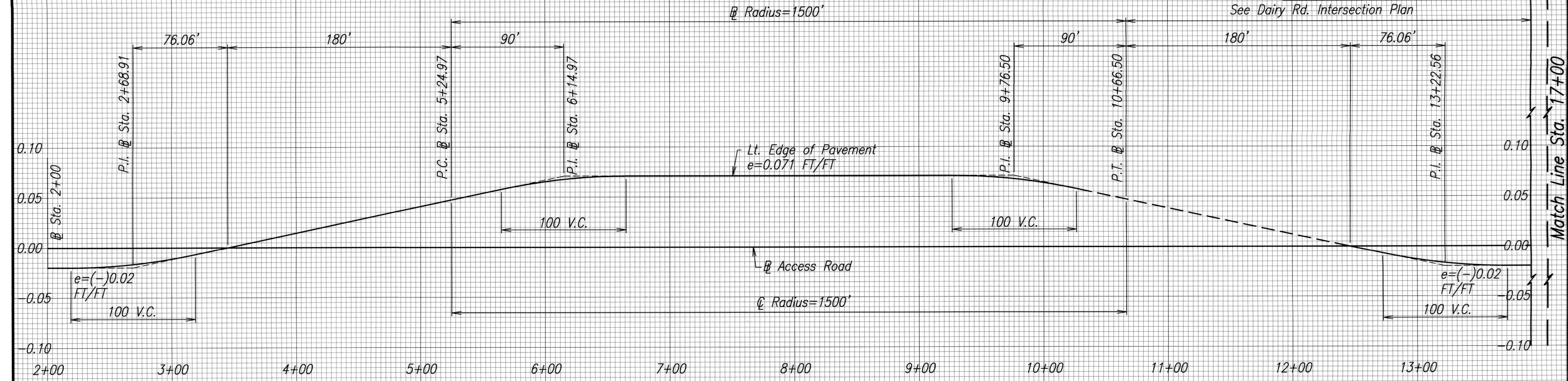
SUPERELEVATION DIAGRAM – MAIN ACCESS ROAD (OUTBOUND LANES) SCALE: HORIZ. 1"=40' VERT. 1"=0.05 FT/FT
