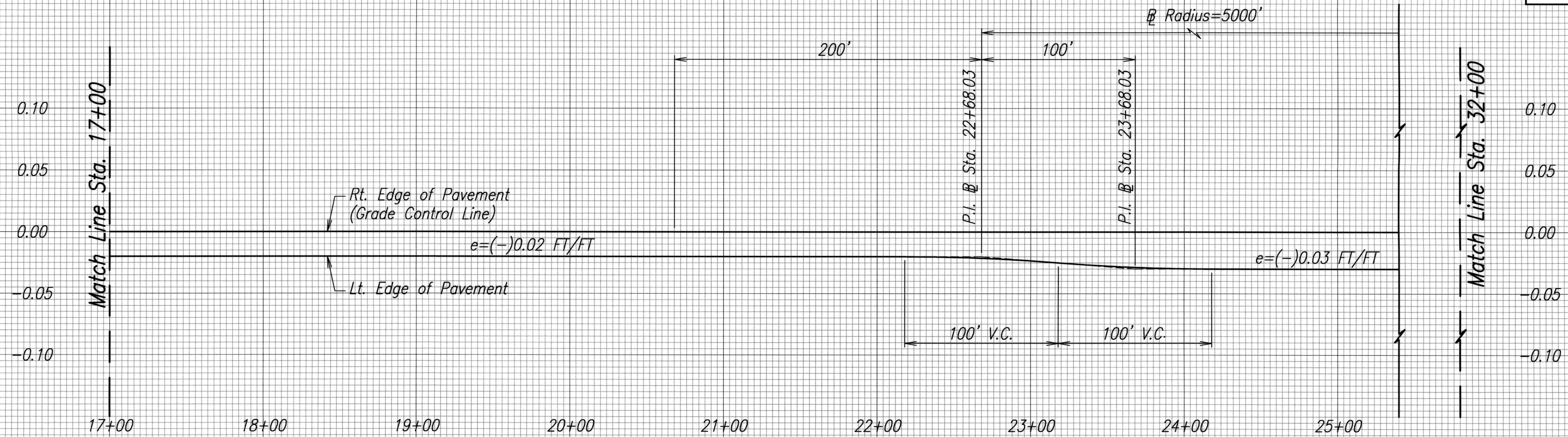
SUPERELEVATION DIAGRAM – MAIN ACCESS ROAD (OUTBOUND LANES) SCALE: HORIZ. 1"=40' VERT. 1"=0.05 FT/FT
