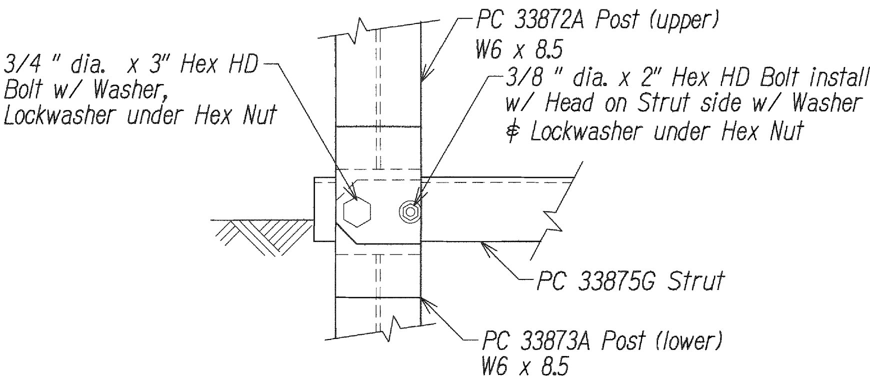
VIEW "H-H"
