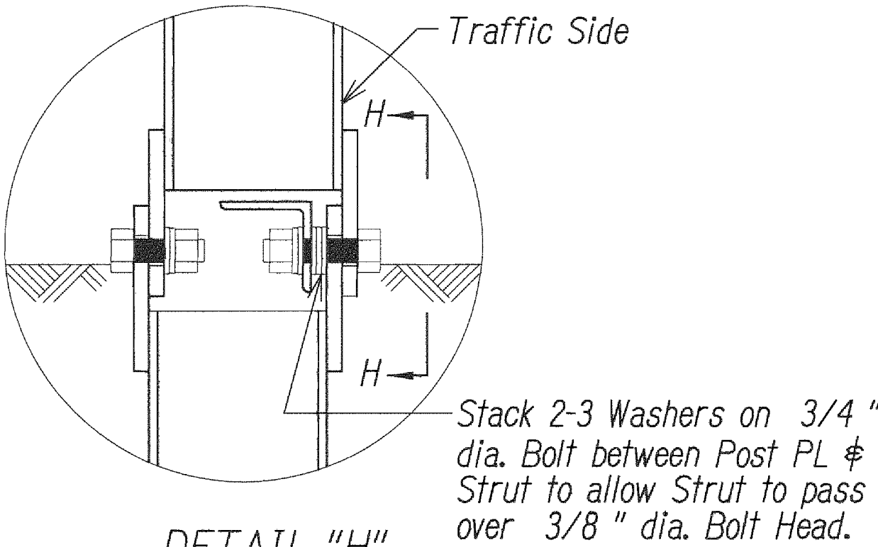
DETAIL "H" (POST #2)
