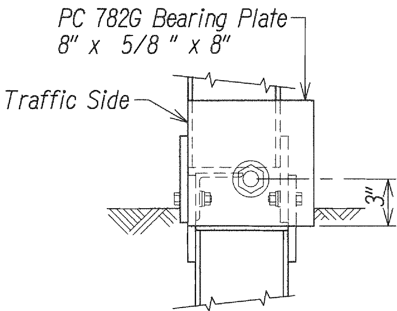
VIEW "K-K"
