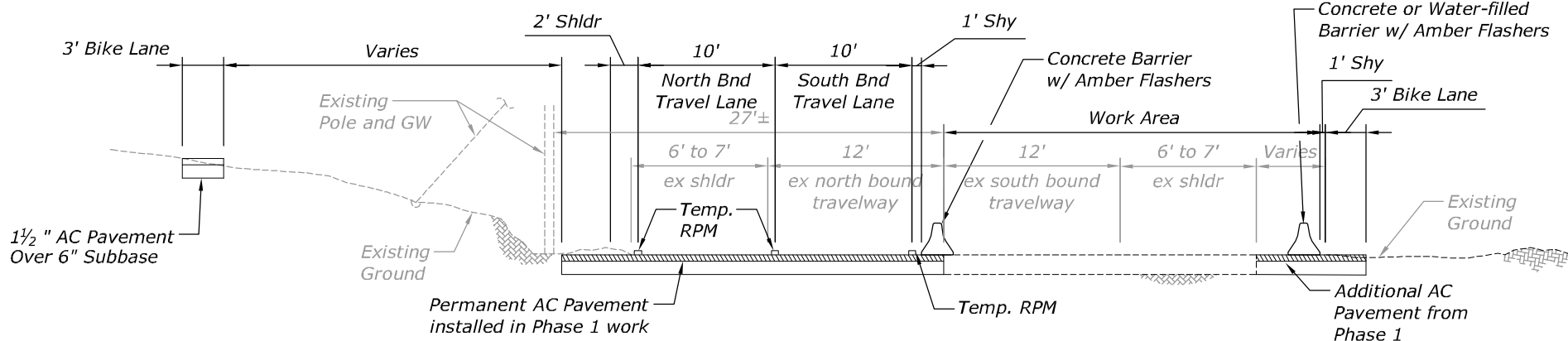
TYPICAL SECTION
