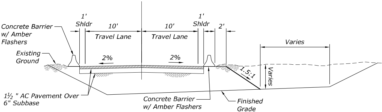
TYPICAL SECTION - CUT
