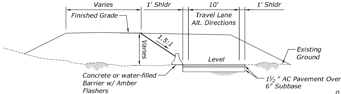
TYPICAL SECTION - FILL (ALONG HOKIOKIO)
