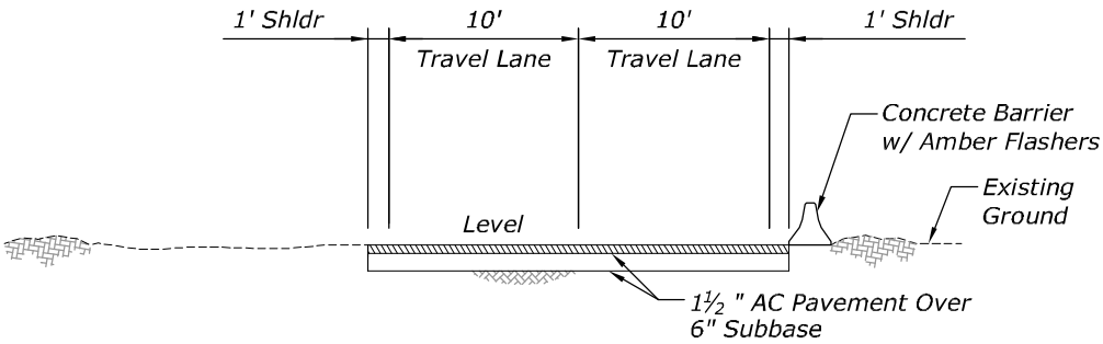
TYPICAL SECTION (ALONG LAHAINA BYPASS)
