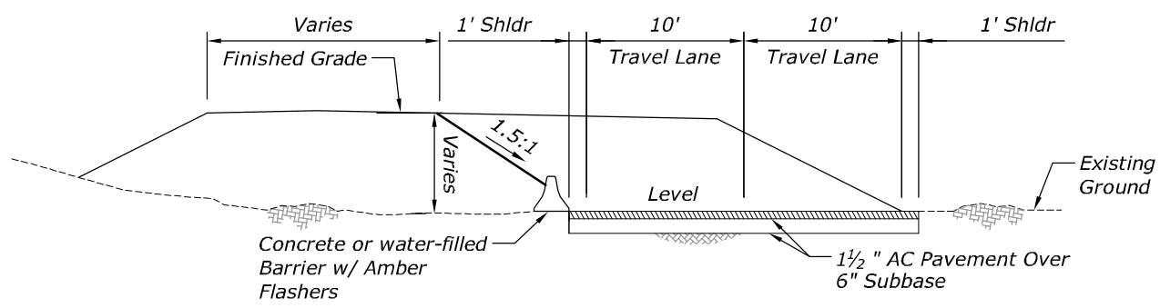
TYPICAL SECTION - FILL (ALONG LAHAINA BYPASS)
