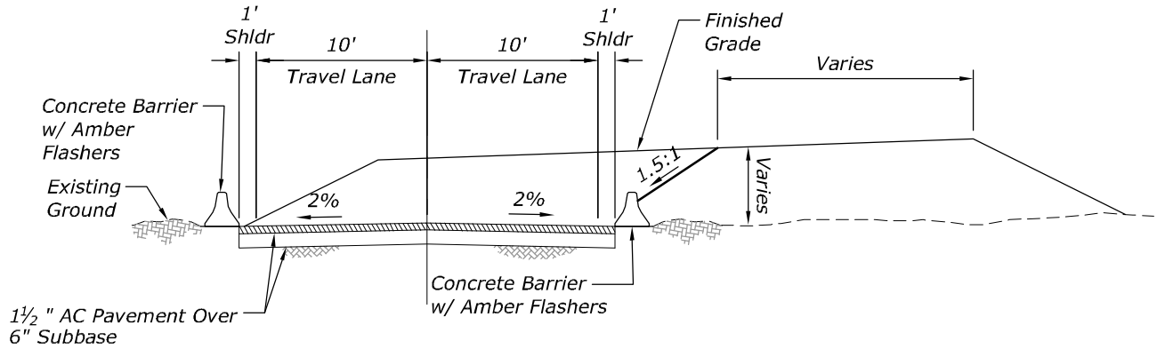
TYPICAL SECTION - FILL
