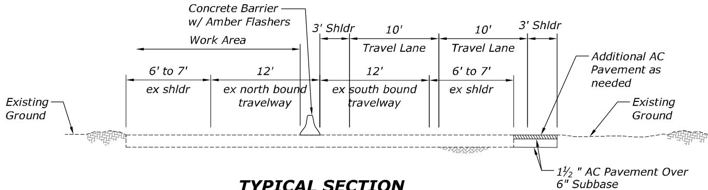
TYPICAL SECTION (HONOAPIILANI HIGHWAY)
