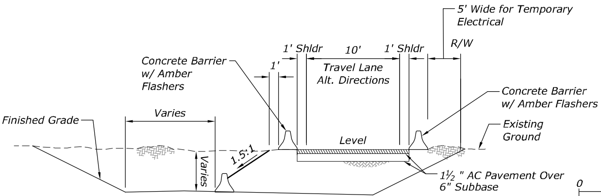
TYPICAL SECTION - CUT
