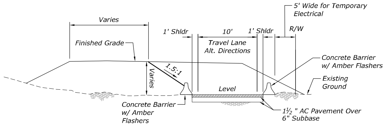
TYPICAL SECTION - FILL
