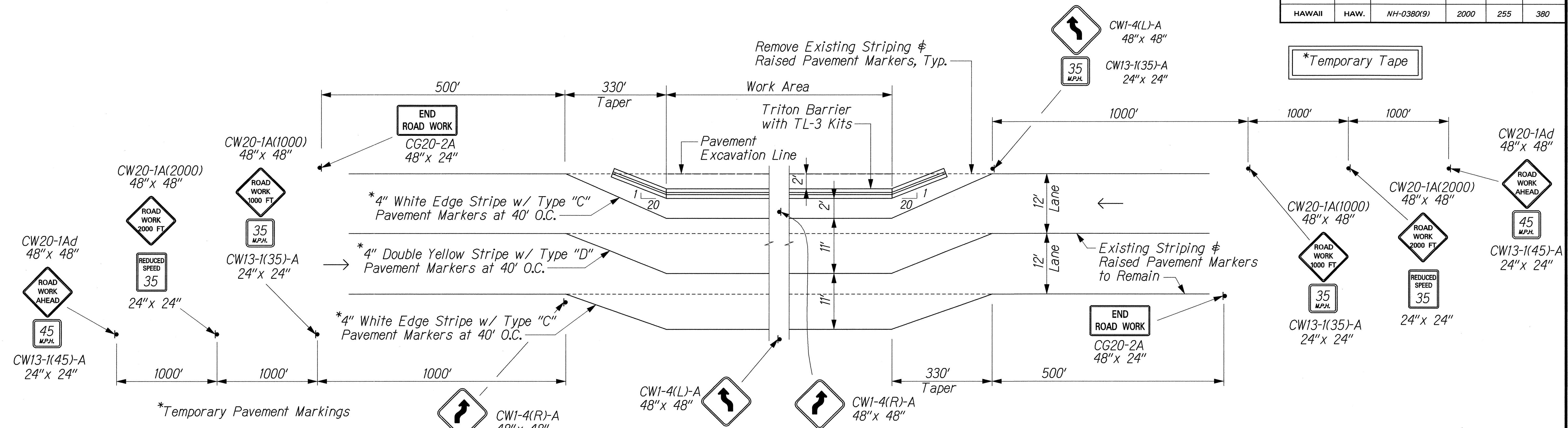
TEMPORARY STRIPING PLAN @ LANE SHIFT Not to Scale
