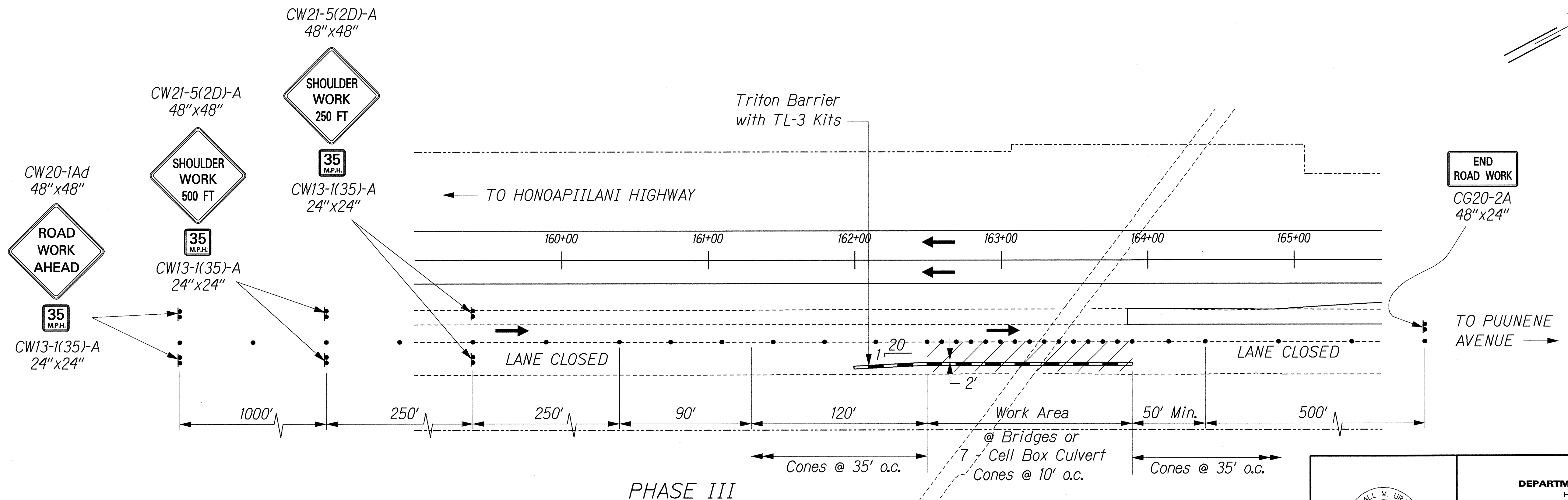
TYPICAL TRAFFIC CONTROL AT BRIDGES AND 7 CELL BOX CULVERT
