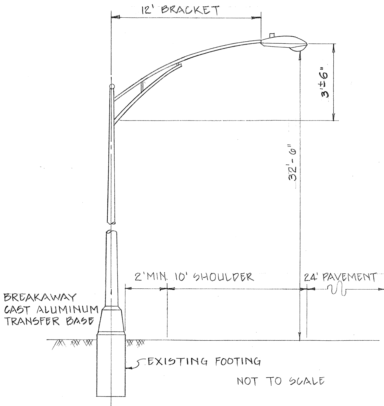
TYPICAL STREET LIGHT STANDARD
