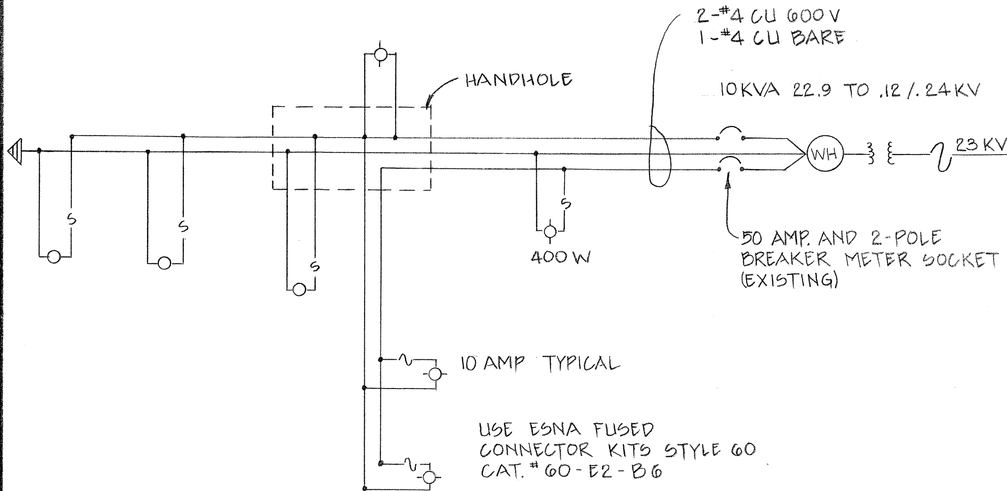
ONE LINE DIAGRAM ST. LIGHTING HONOAPIILANI & NEW HIGHWAY INTERSECTION 7-400 WATT
