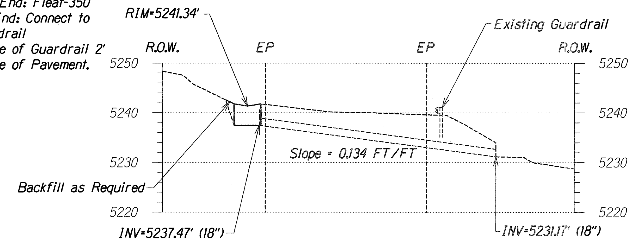
Profile CC-CC Scale: 1"=10'-0"
