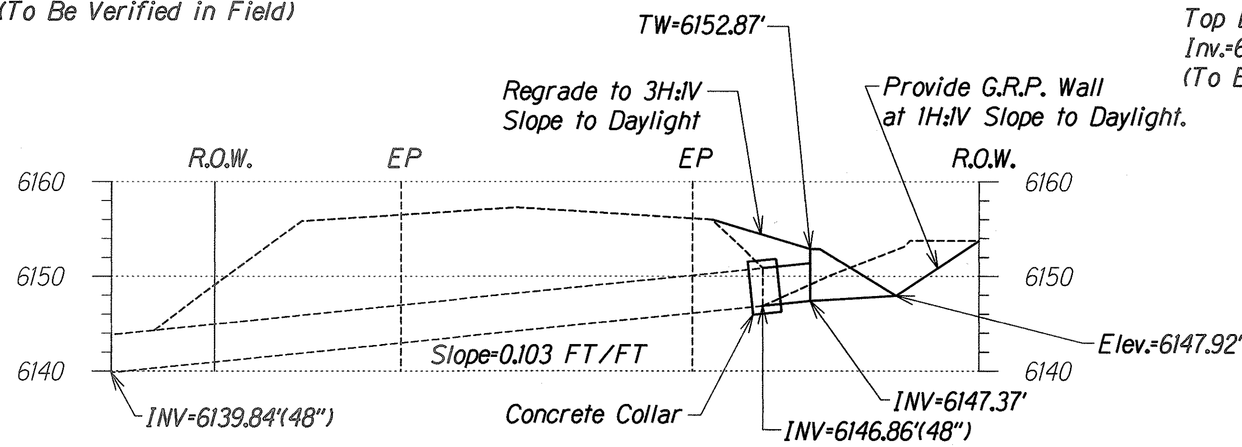
Profile QQ-QQ Scale: 1"=10'-0"
