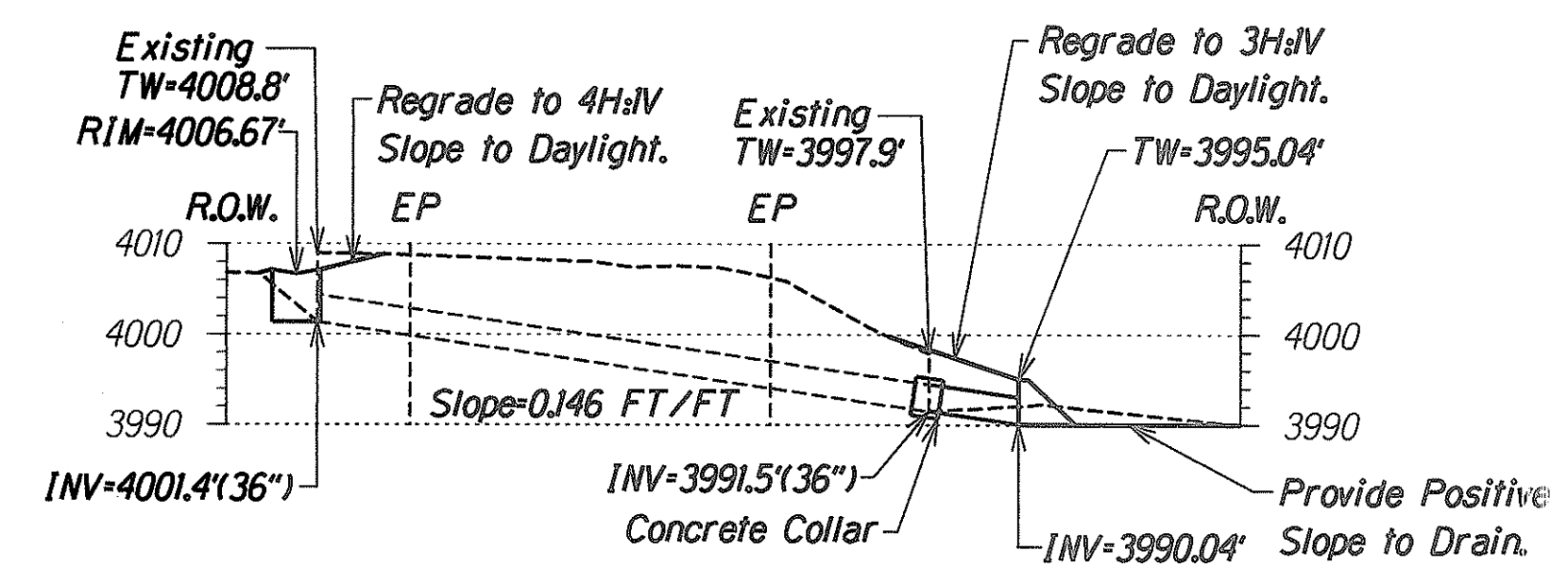
Profile IM-IM Scale: 1"=20'-0"
