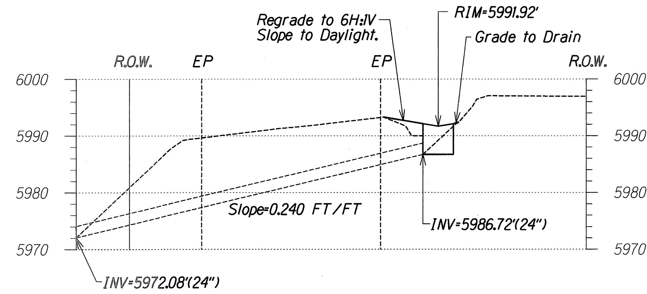
Profile KK-KK Scale: 1"=10'-0"
