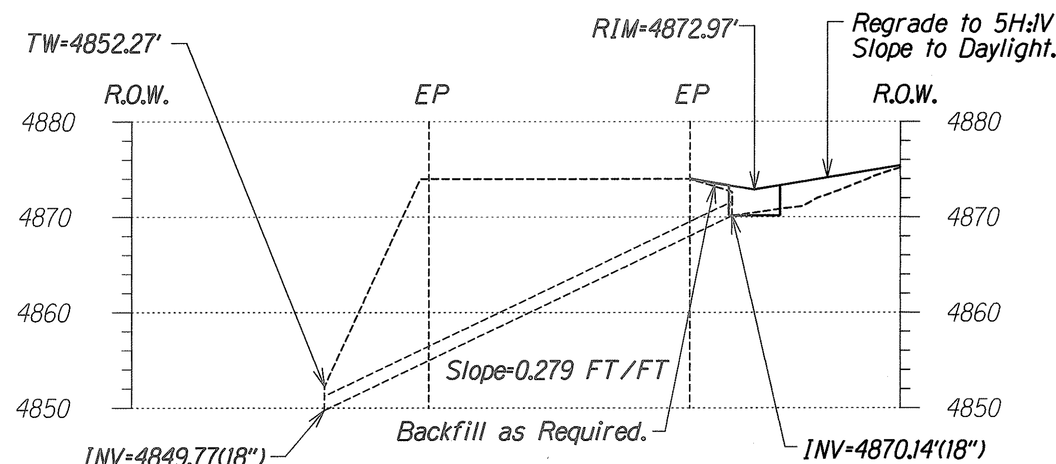
Profile VA-VA Scale: 1"=10'-0"
