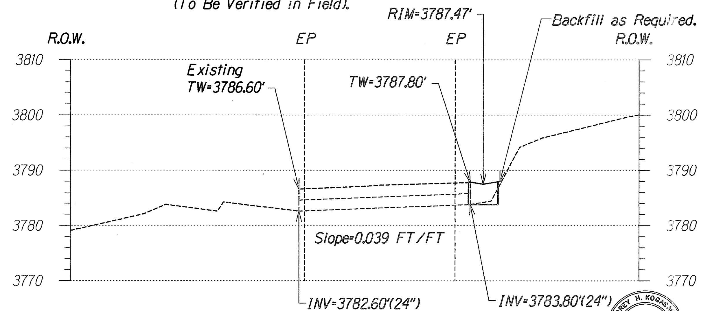
Profile IB-IB Scale: 1"=10'-0"
