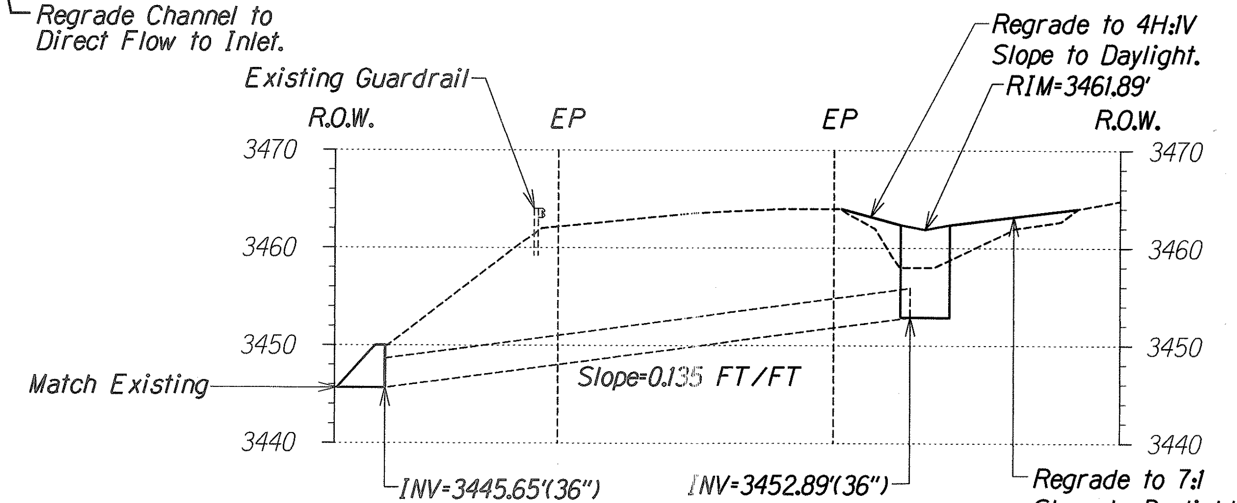
Profile C-C Scale: 1"=10'-0"
