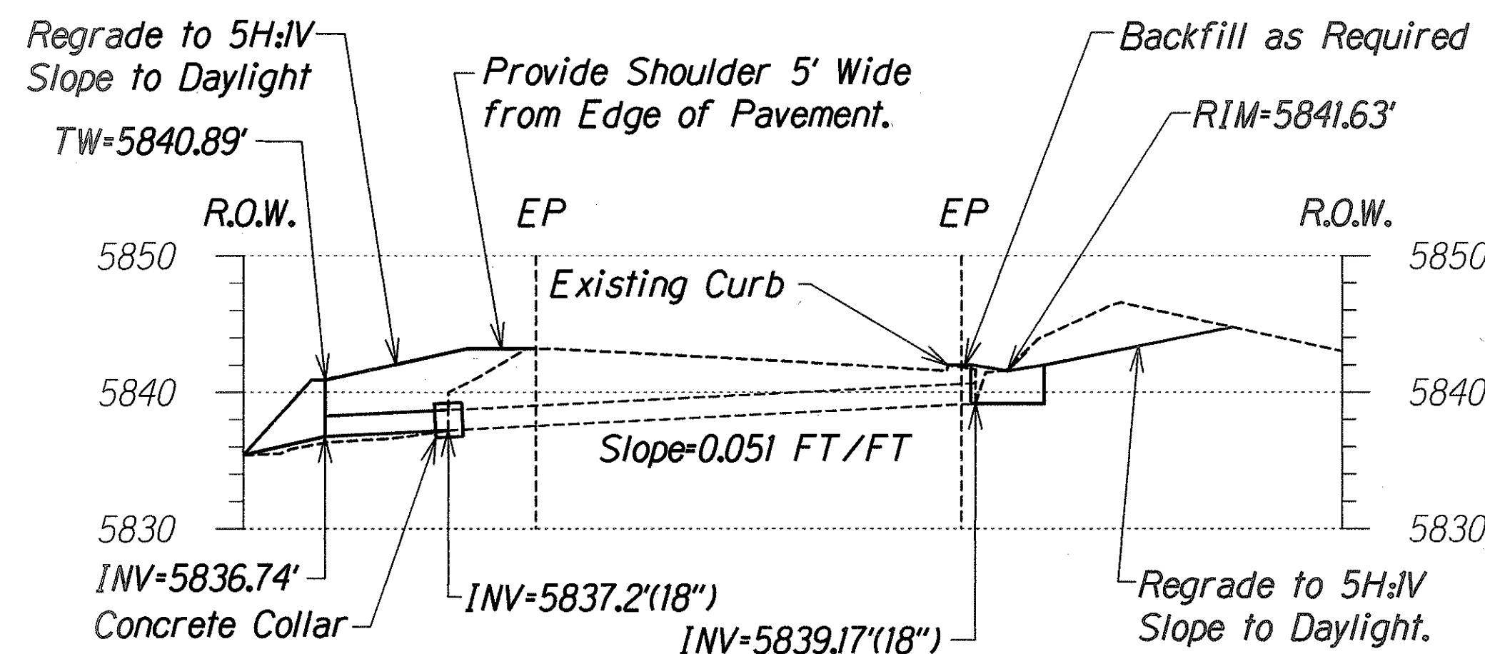
Profile GG-GG Scale: 1"=10'-0"
