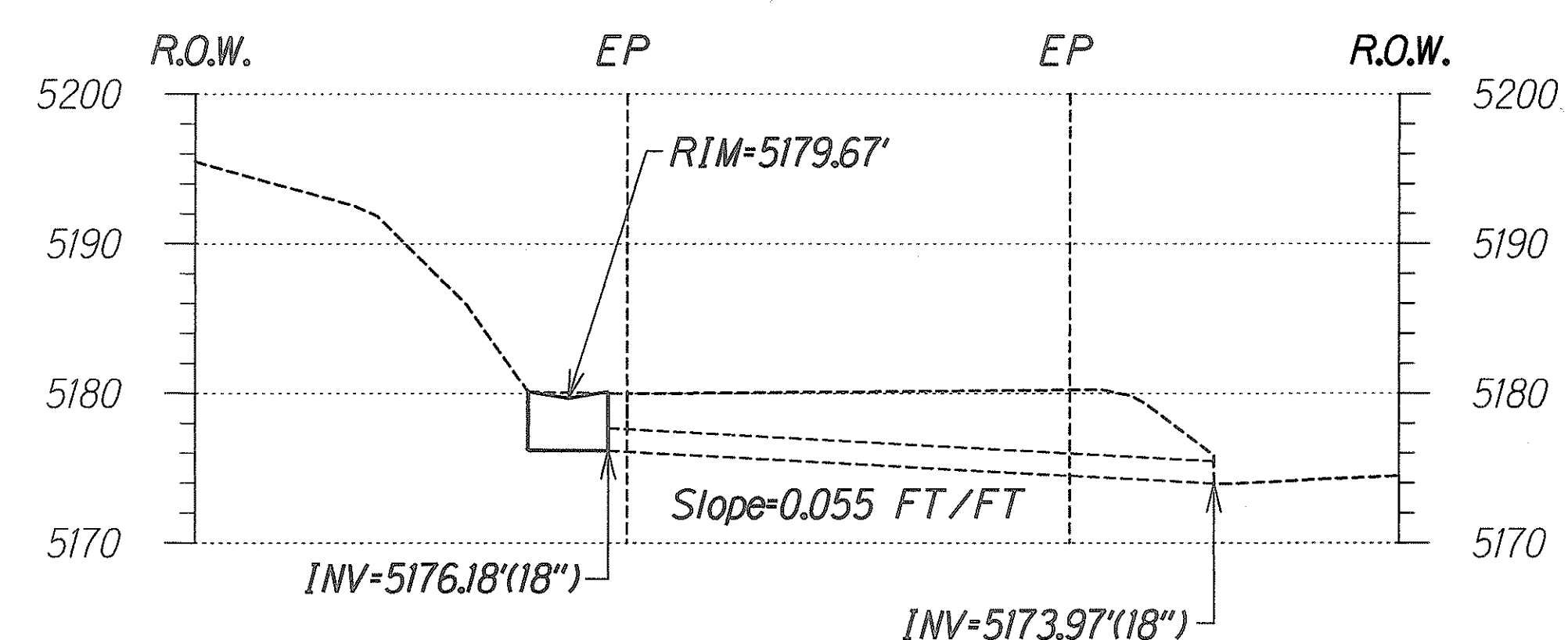
Profile AA-AA Scale: 1"=10'-0"
