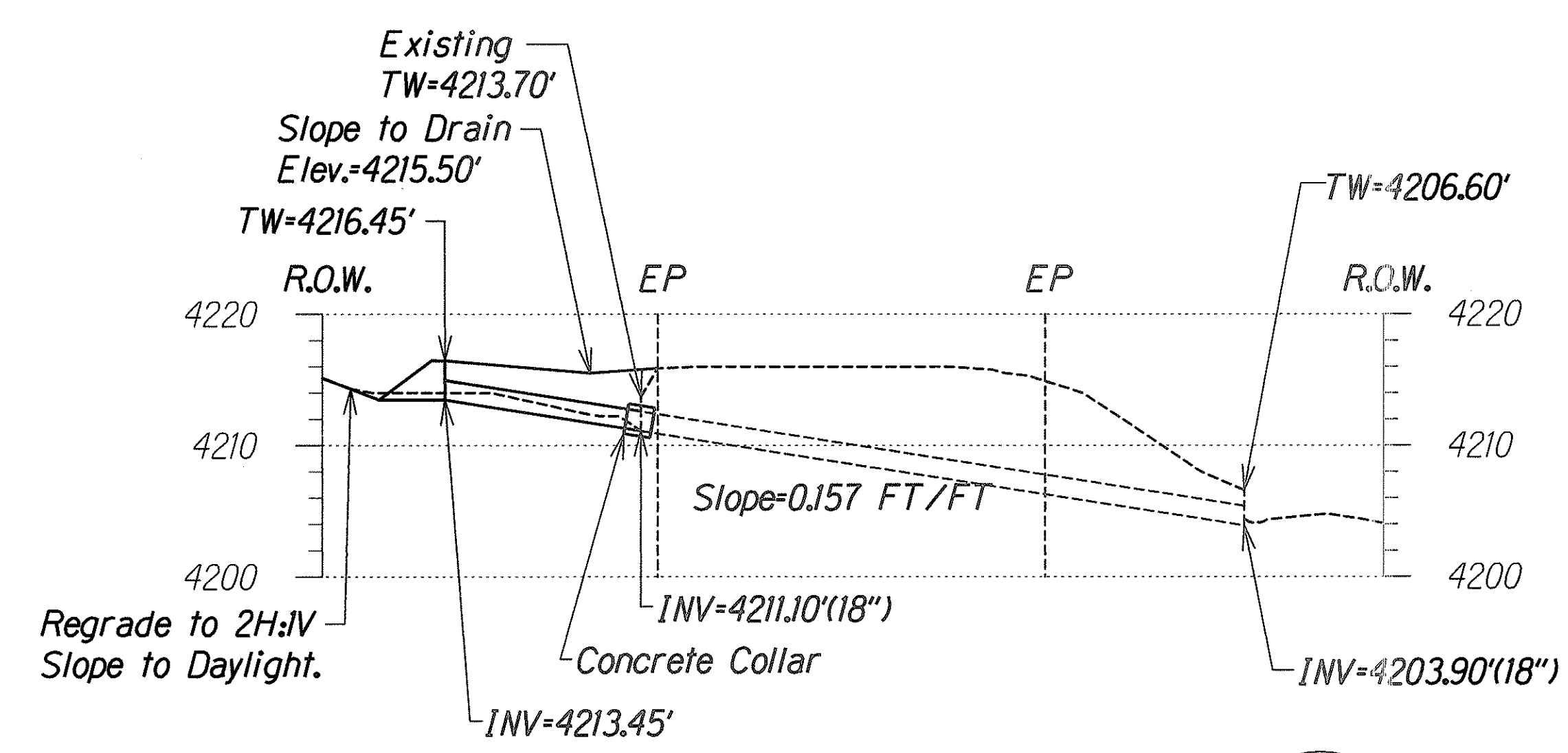
Profile M-M Scale: 1"=10'-0"
