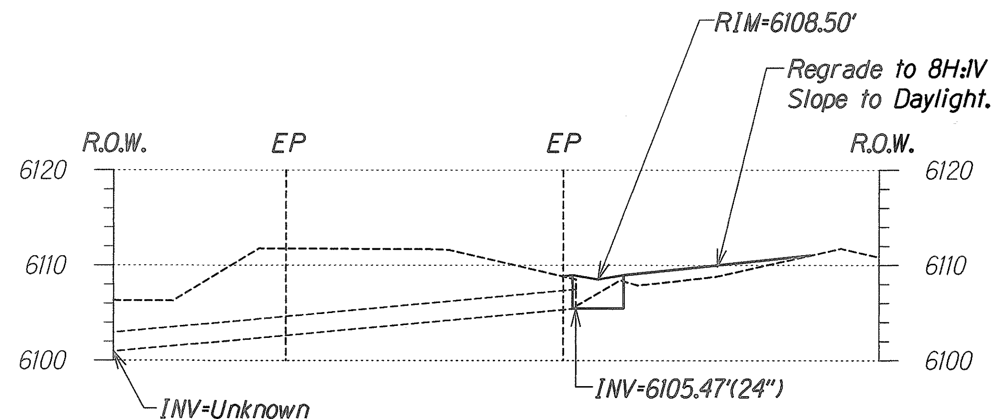
Profile 00A-00A Scale: 1"=10'-0"
