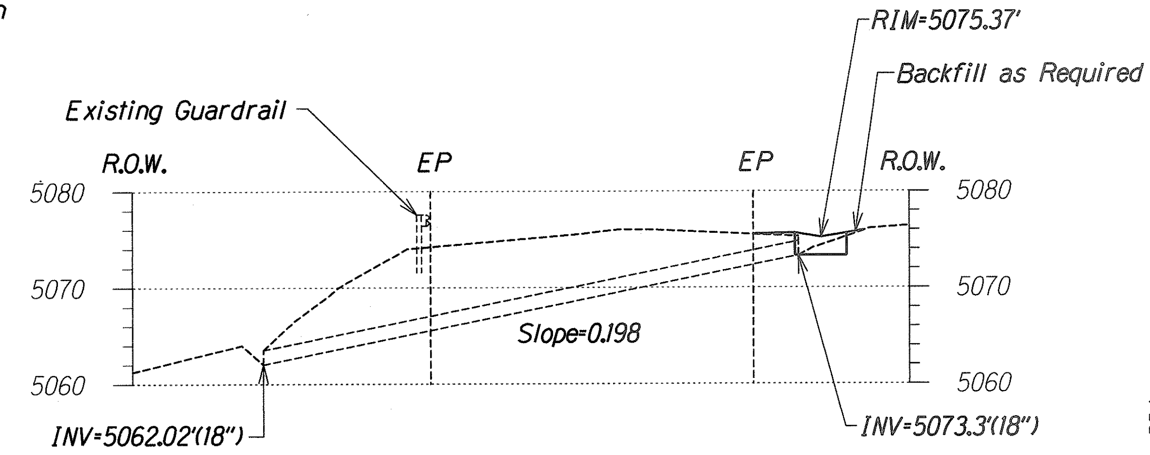
Profile W-W Scale: 1"=10'-0"
