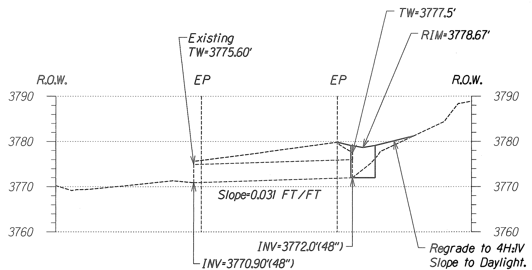
Profile IA-IA Scale: 1"=10'-0"
