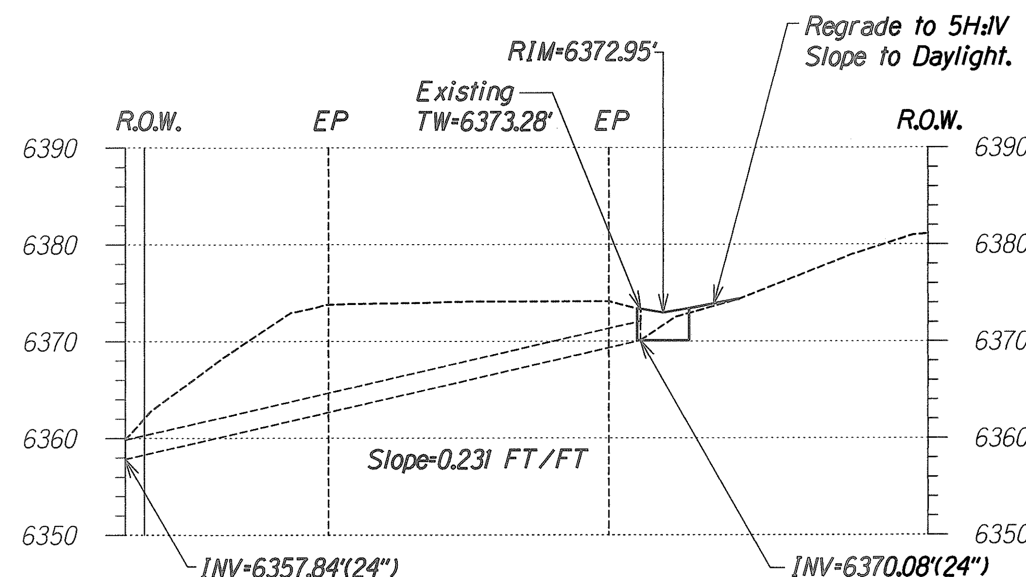
Profile WW-WW Scale: 1"=10'-0"
