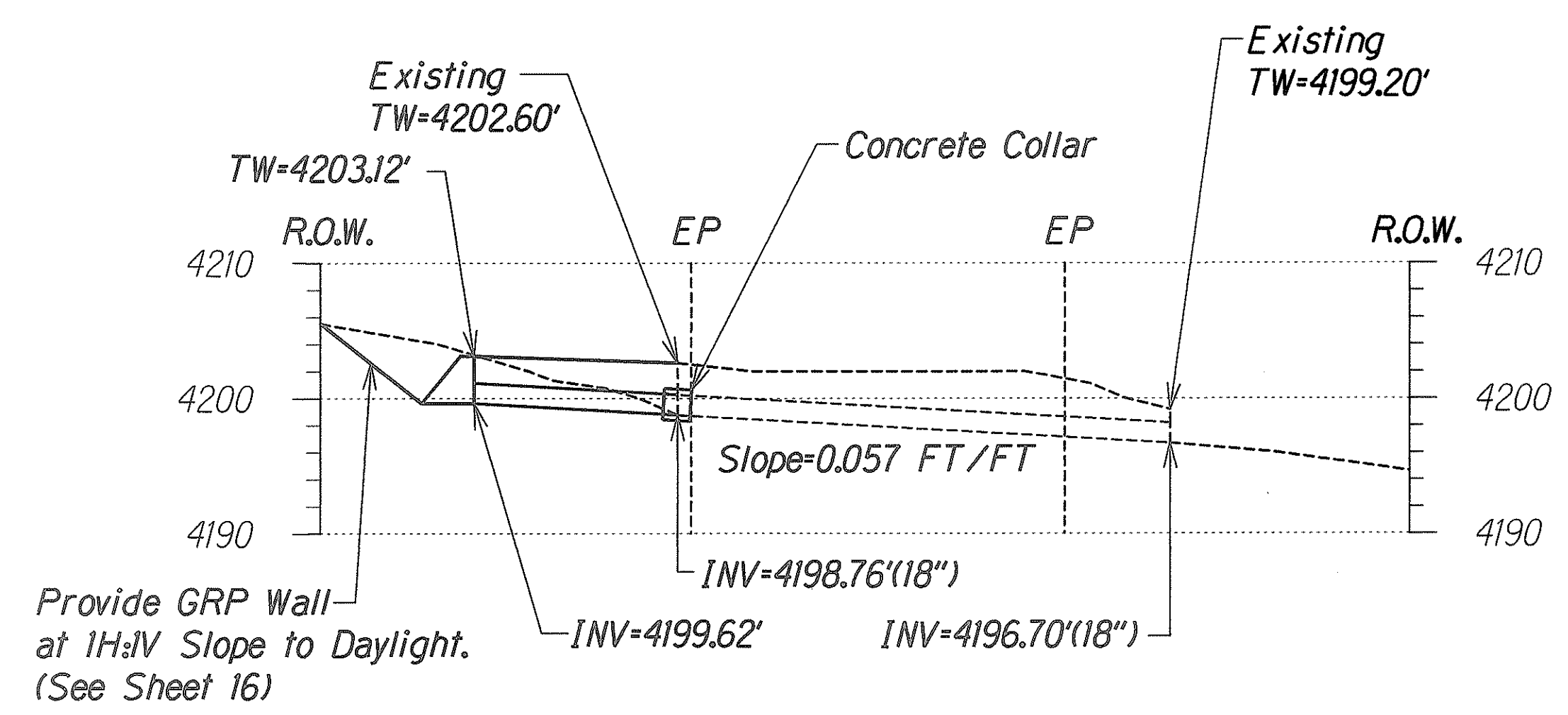
Profile L-L Scale: 1"=10'-0"
