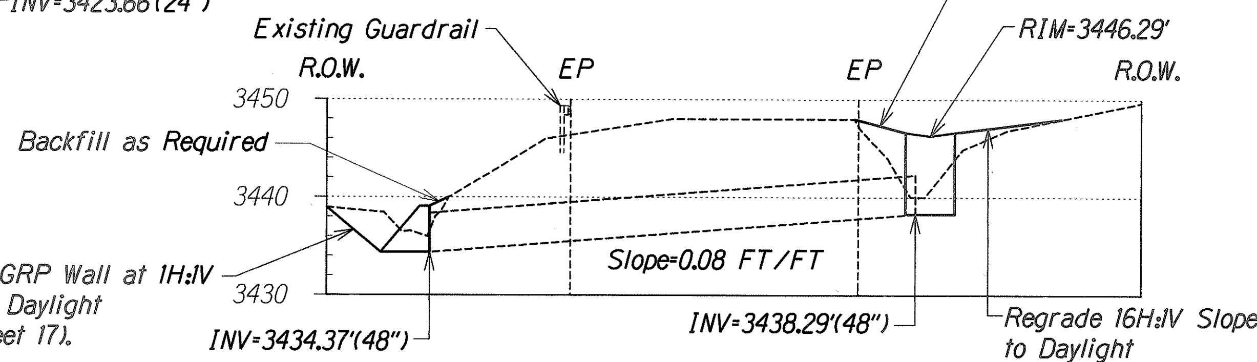
Profile B-B Scale: 1"=10'-0"
