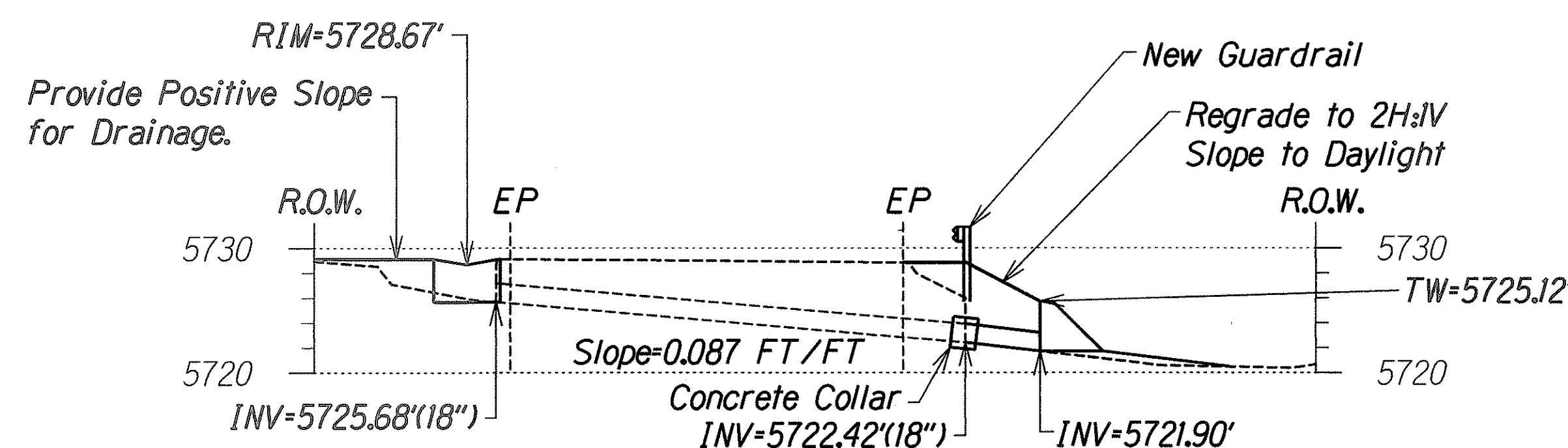
Profile EE-EE Scale: 1"=10'-0"
