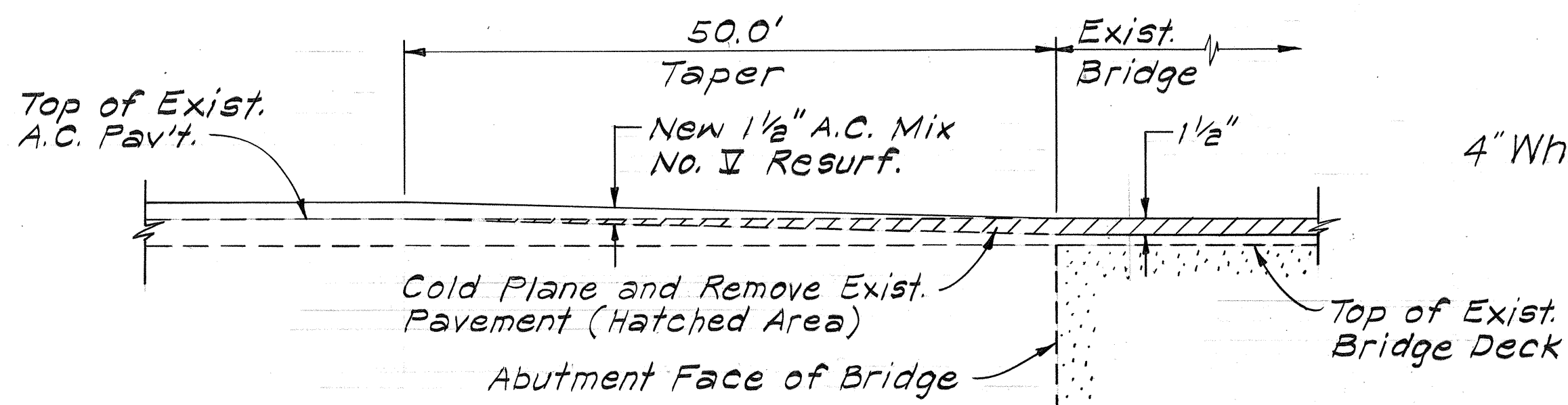
DETAIL AT WAIKALE BRIDGE Not to Scale
