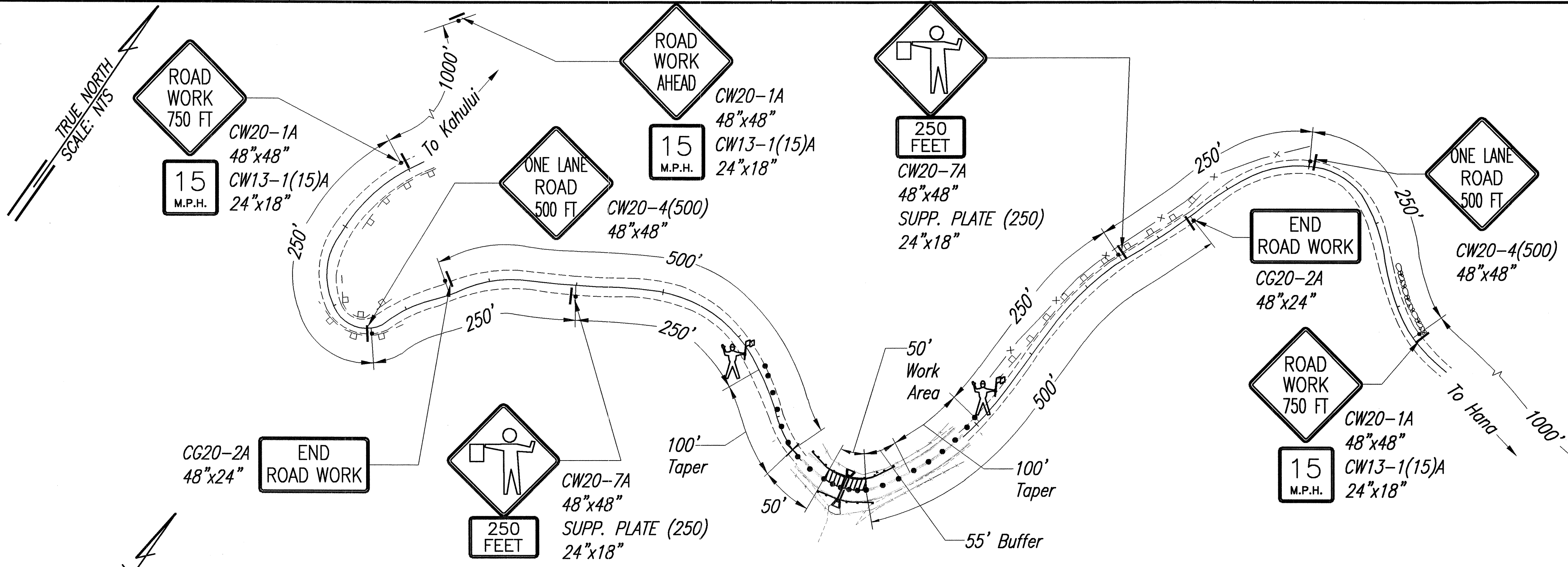
Site 1 Traffic Control Plan - 1 Scale: NTS
