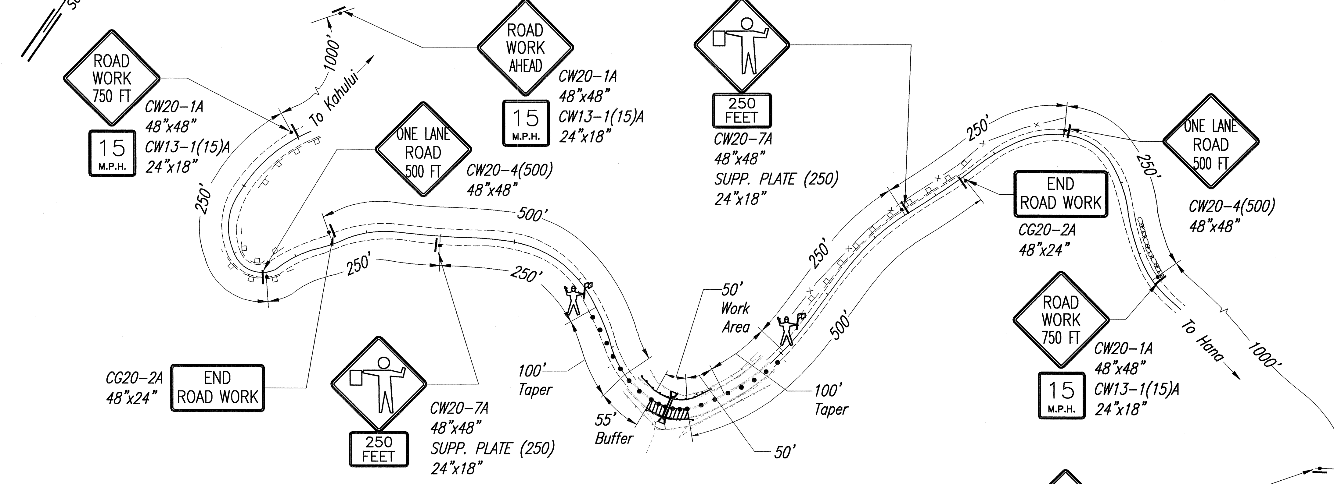
Site 1 Traffic Control Plan - 2 Scale: NTS
