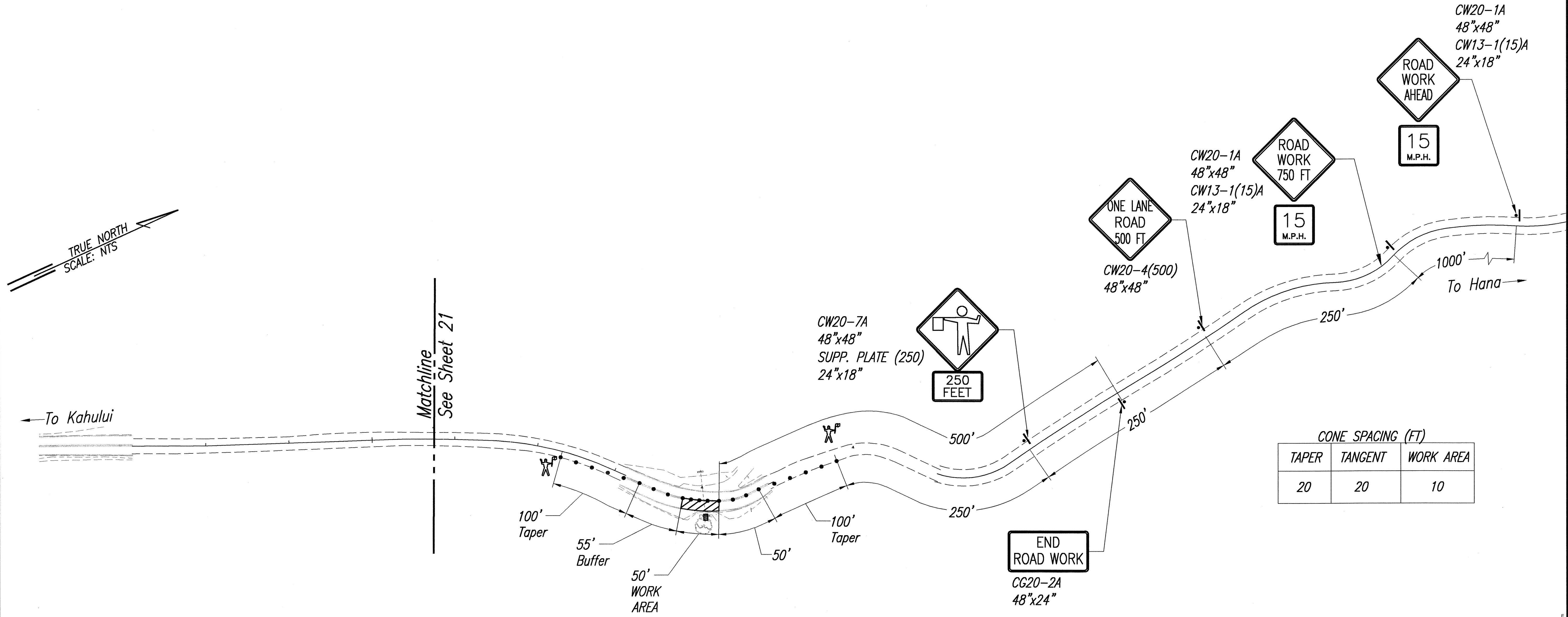
Site 5 Traffic Control Plan Scale: NTS
