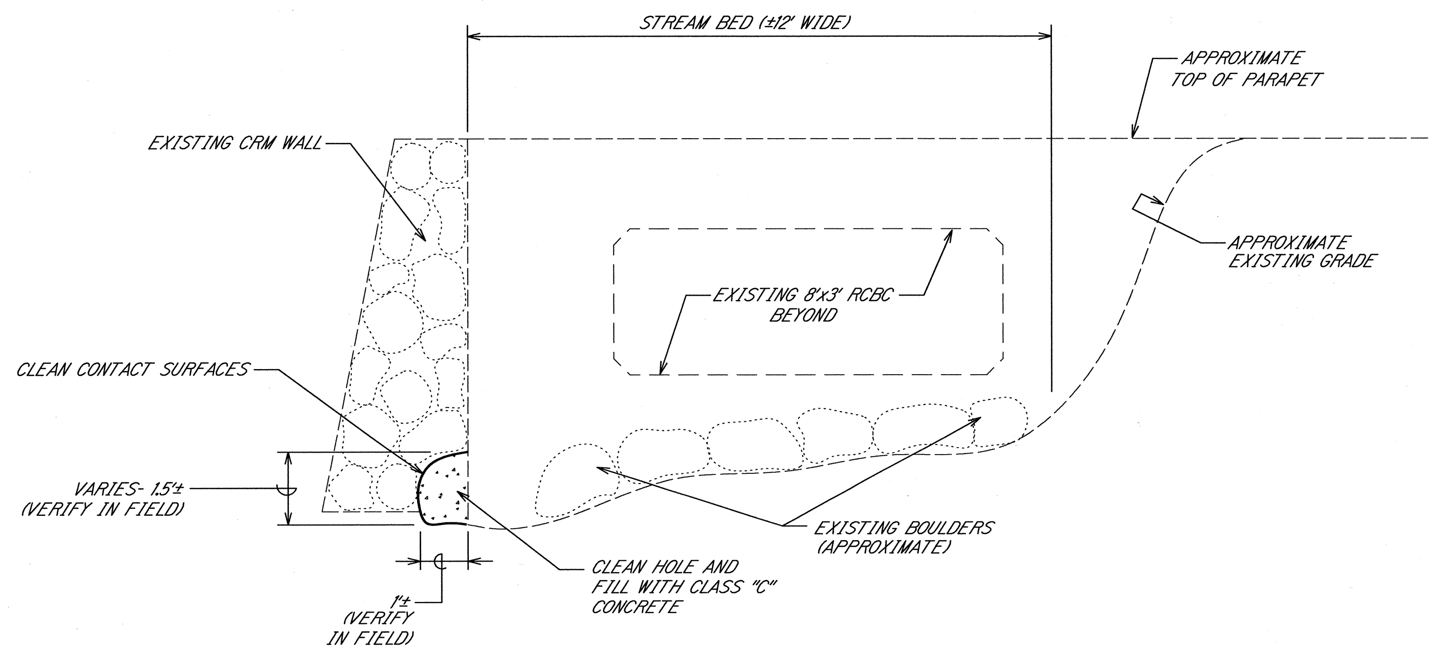
TYPICAL SECTION - REPAIR OF UNDERMINED/BROKEN CRM BASE
