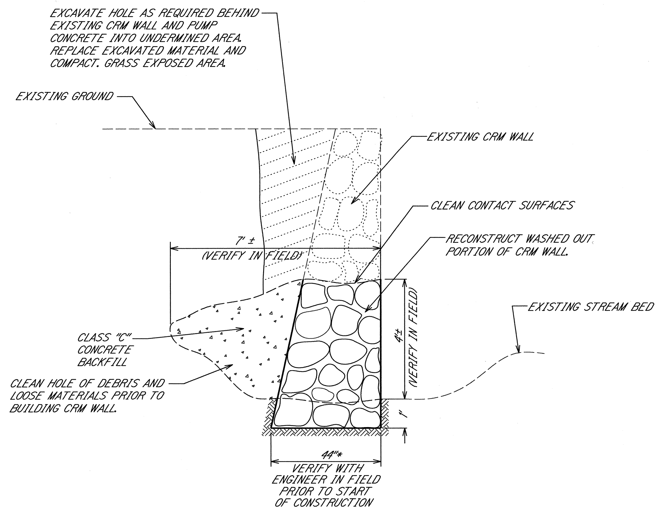
TYPICAL SECTION - REPAIR OF WASHED OUT CRM WALL
