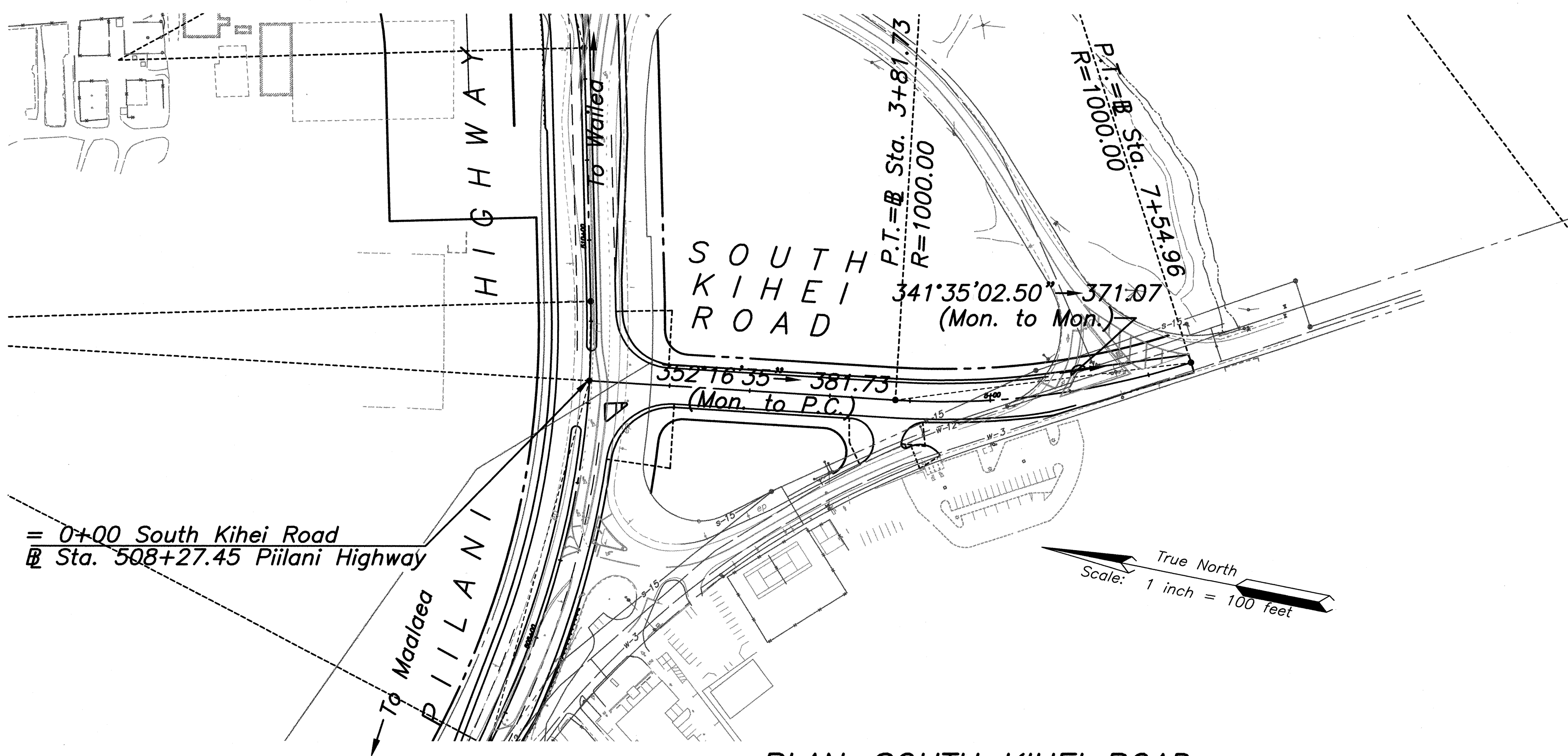
PLAN-SOUTH KIHAI ROAD
