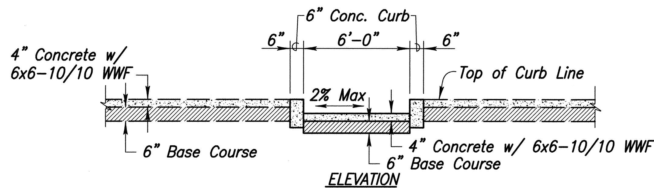
CURB ISLAND DETAIL Scale: 1"=10'
