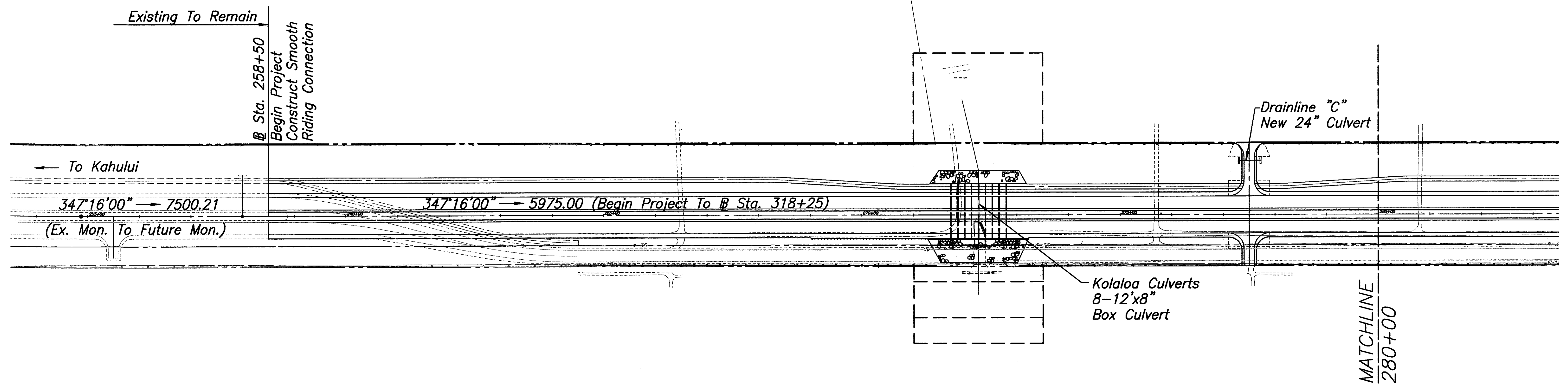
PLAN-MOKULELE HIGHWAY Scale: 1"=100'
