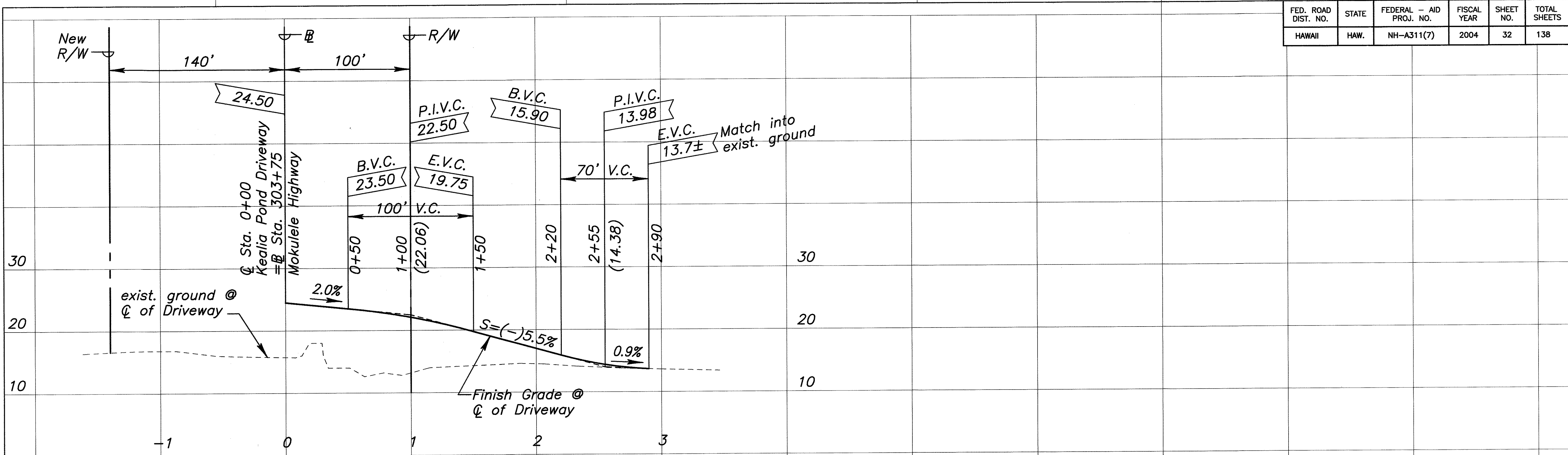
PROFILE-KEALIA POND DRIVEWAY @ STA. 303+75
