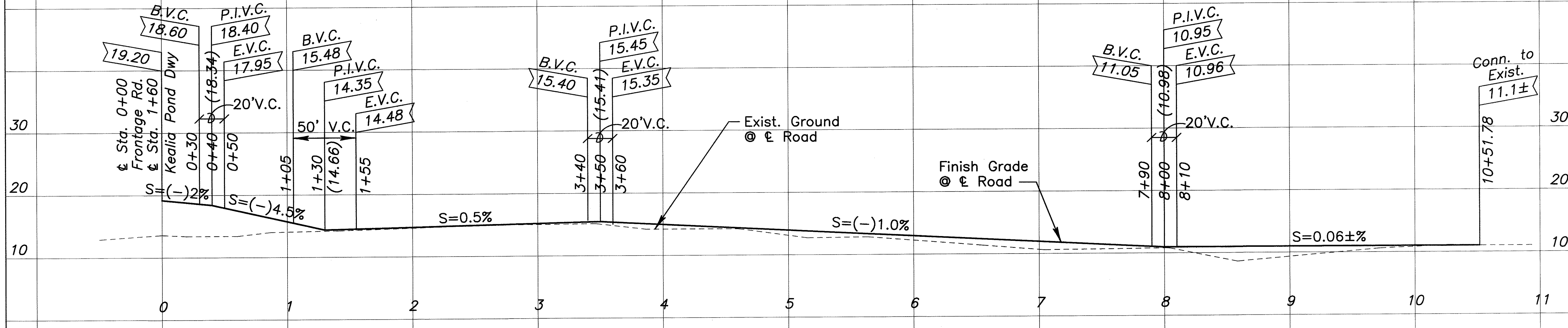
PROFILE-KEALIA POND DRIVEWAY @ STA. 303+75
