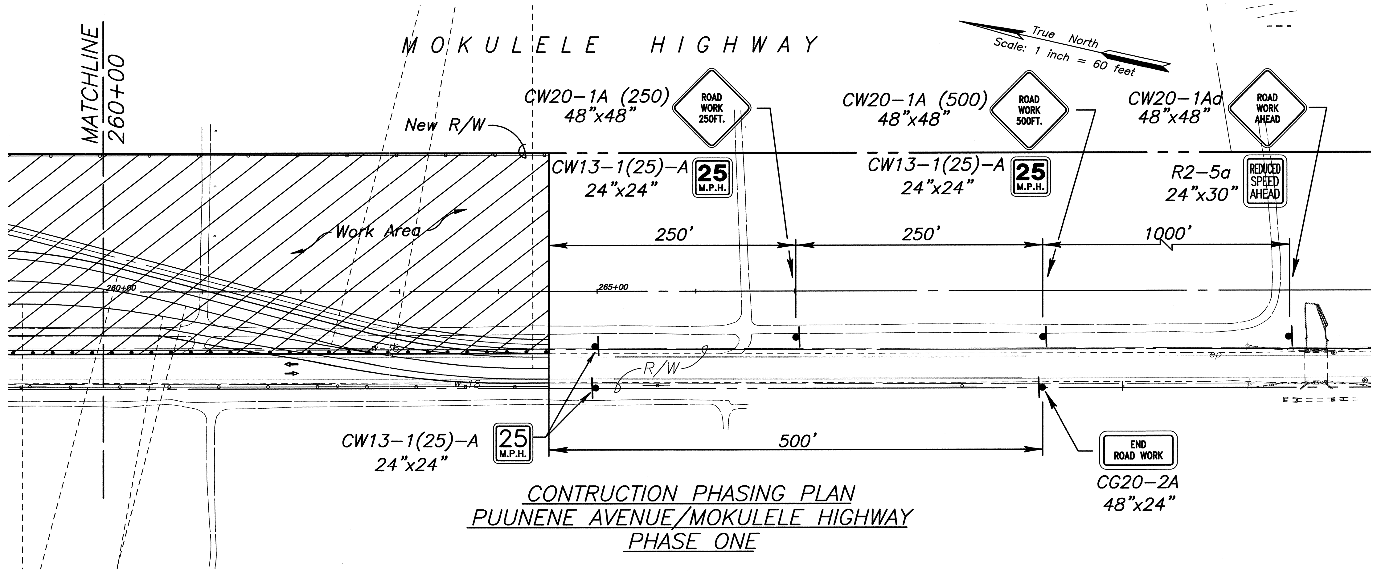
CONSTRUCTION PHASING PLAN PUUNENE AVENUE/MOKULELE HIGHWAY PHASE ONE
