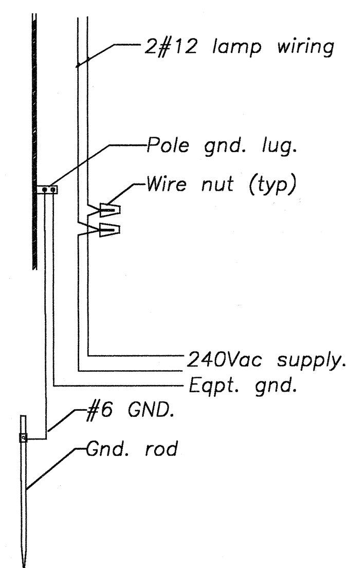
STREET LIGHT WIRING DETAIL NTS
