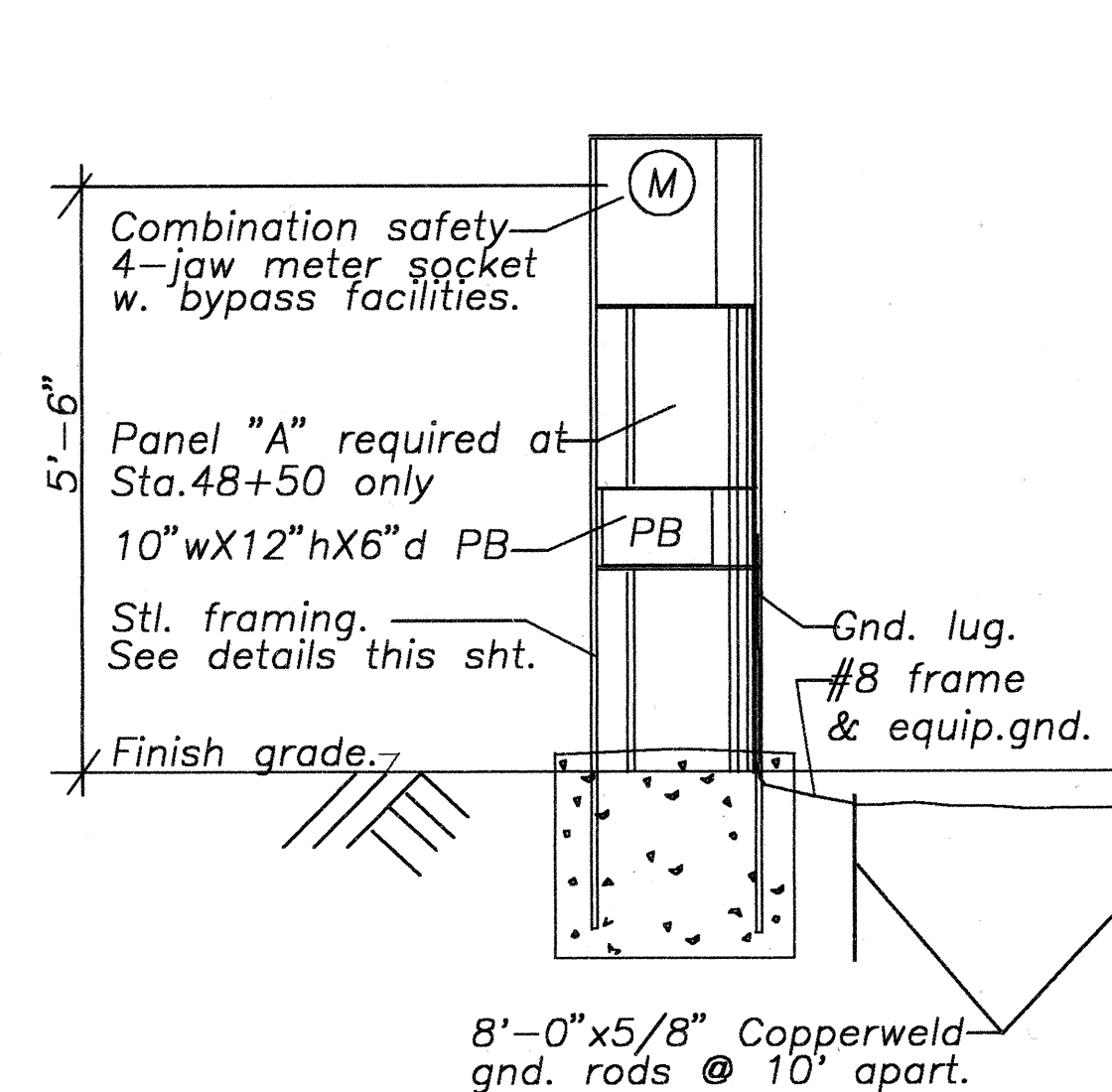
SERVICE EQUIPMENT ELEVATION NTS
