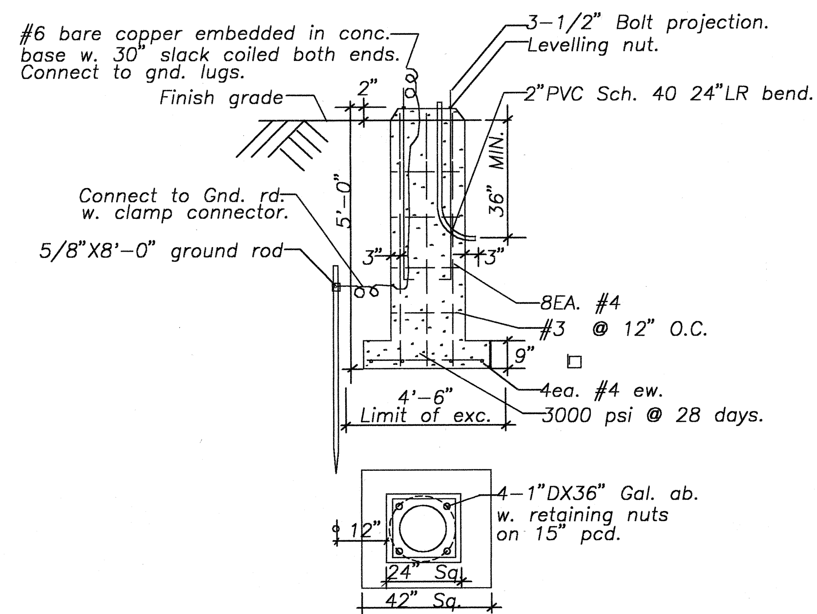
TRAFFIC CONTROL SERVICE EQUIPMENT DETAIL NTS
