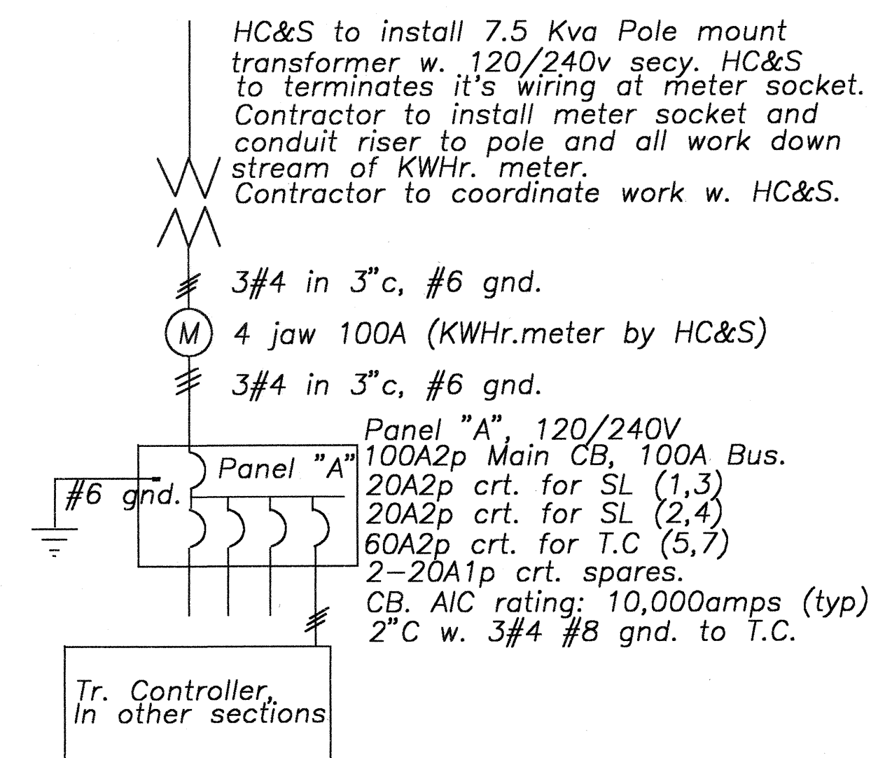
SINGLE LINE DIAGRAM Sta.48+50 NTS
