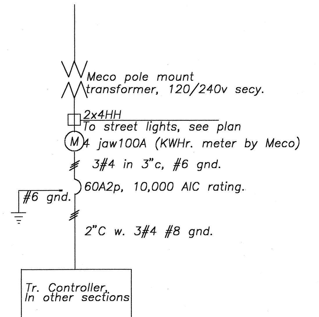
SINGLE LINE DIAGRAM HANSEN ROAD NTS
