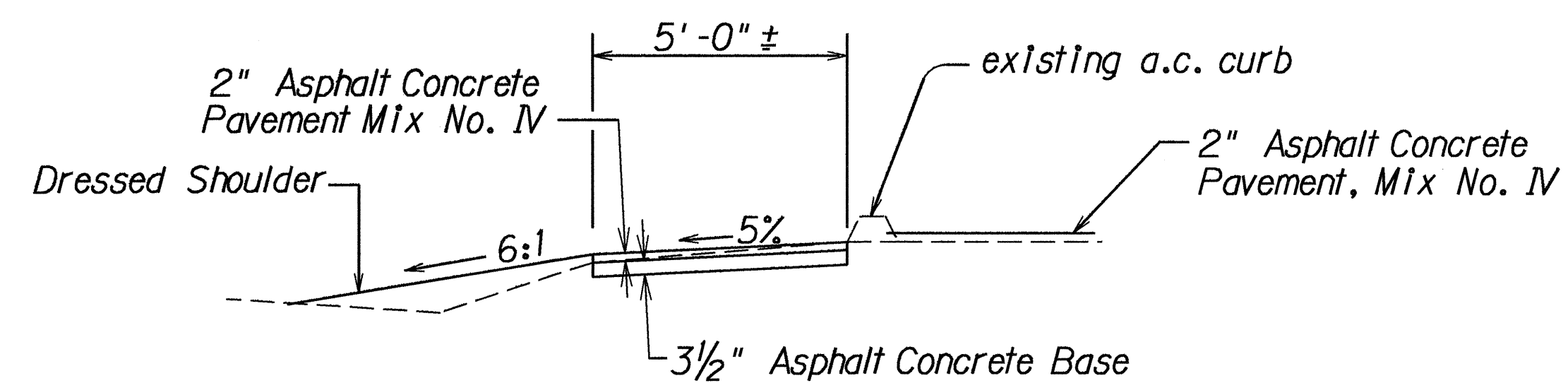
SECTION "A" STA. 96+40± LT. - STA. 97+85± LT. Not To Scale
