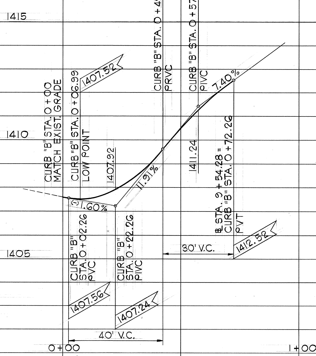
PROFILE ~ CURB "B"
