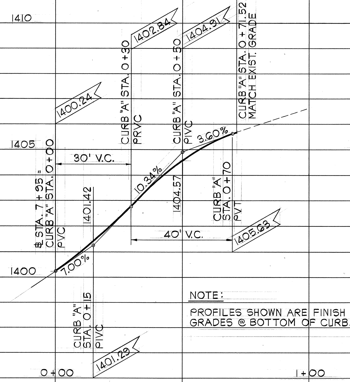
PROFILE ~ CURB "A"
