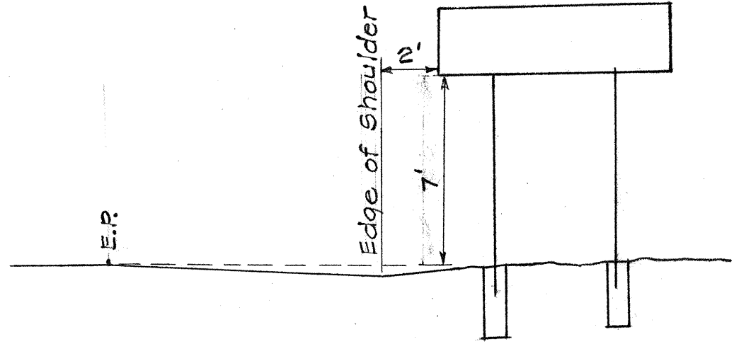
TYPICAL DESTINATION SIGN LOCATION Not to Scale
