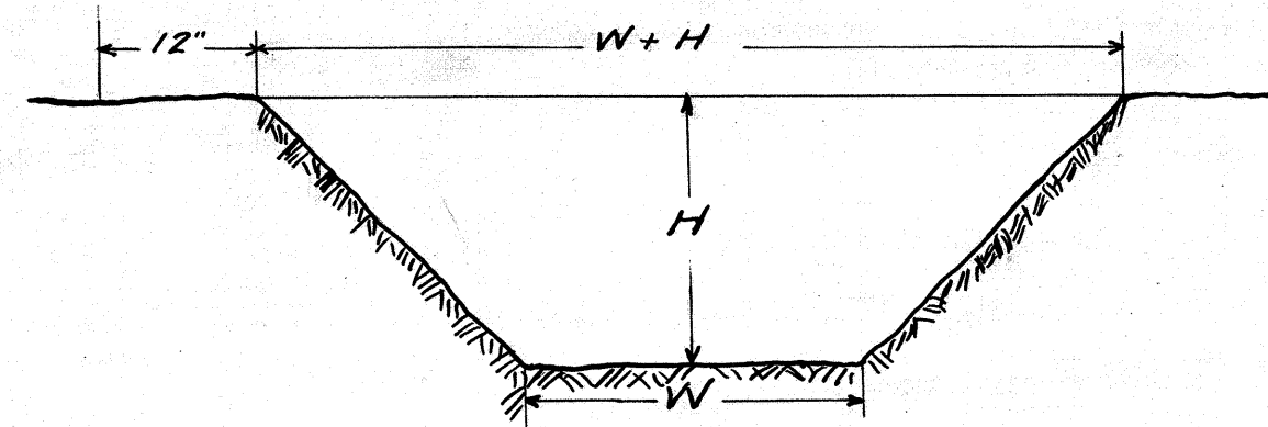
STANDARD SECTION OF OUTLET DITCH.
