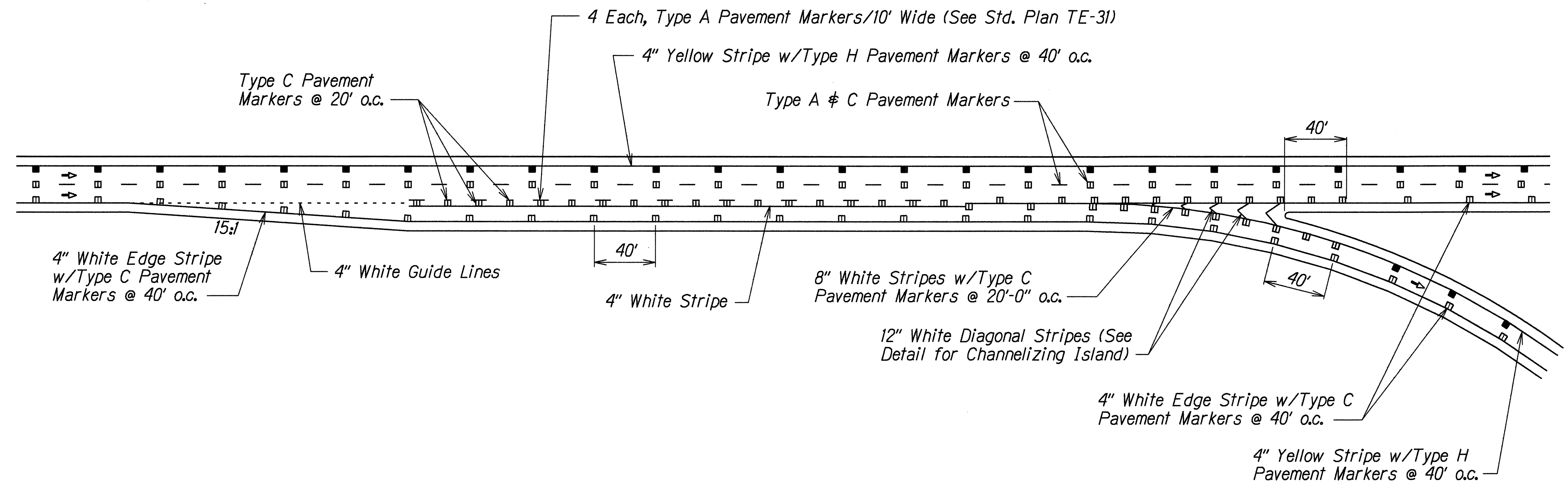
TYPICAL INTERSECTION PARALLEL DECELERATION LANE PAVEMENT MARKINGS Not To Scale
