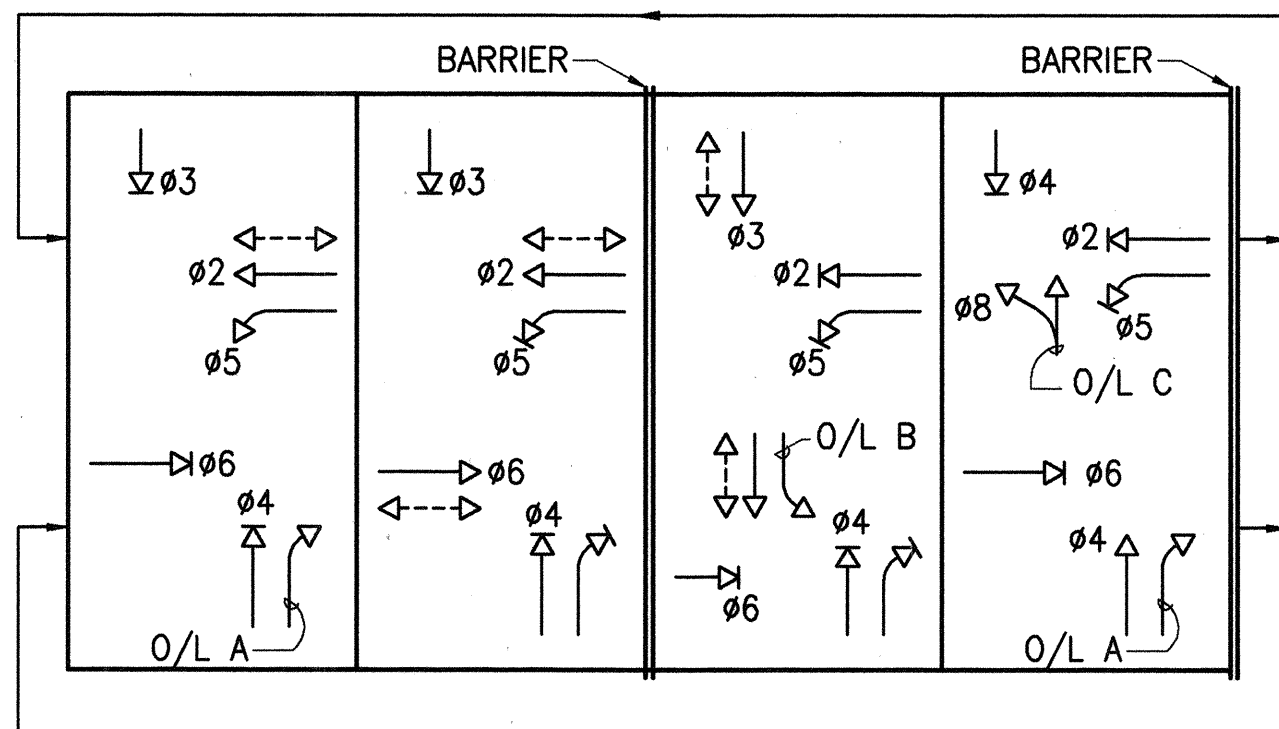
PHASE ASSIGNMENT DIAGRAM
