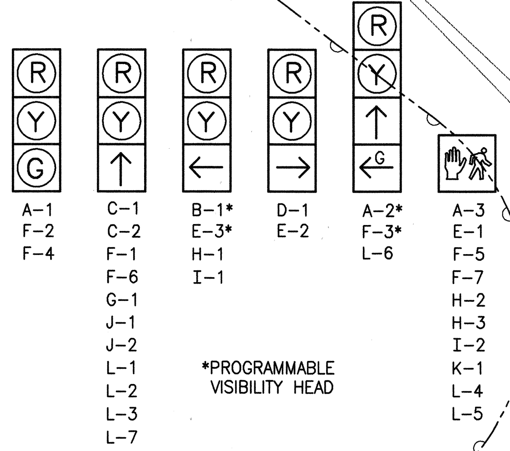
SIGNAL INDICATIONS
