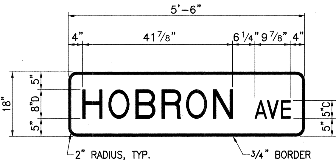
STREET NAME SIGN DETAIL NOT TO SCALE
