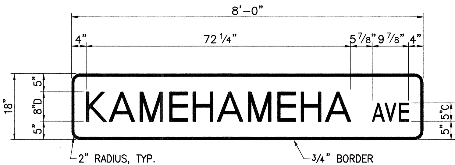
STREET NAME SIGN DETAIL NOT TO SCALE
