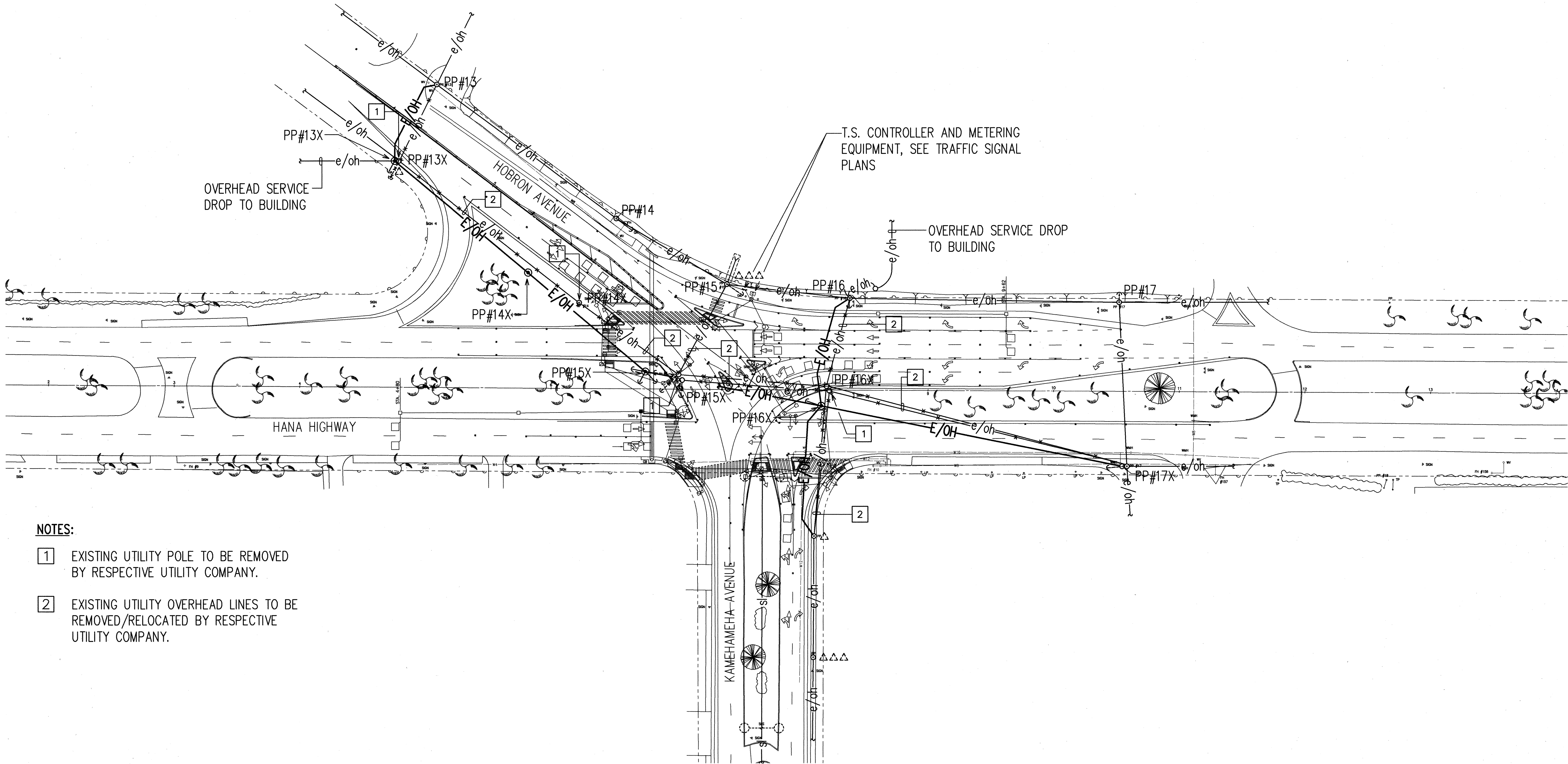
ELECTRICAL PLAN SCALE: 1"=40'
