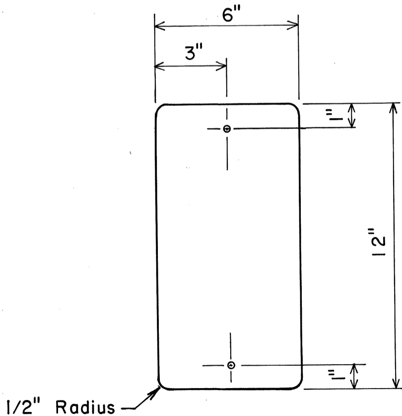
TYPE II OBJECT MARKER POST MOUNTED Not To Scale
