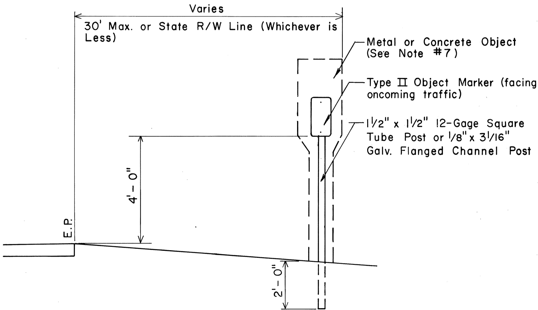
TYPE II POST MOUNTED OBJECT MARKER DETAIL Not To Scale
