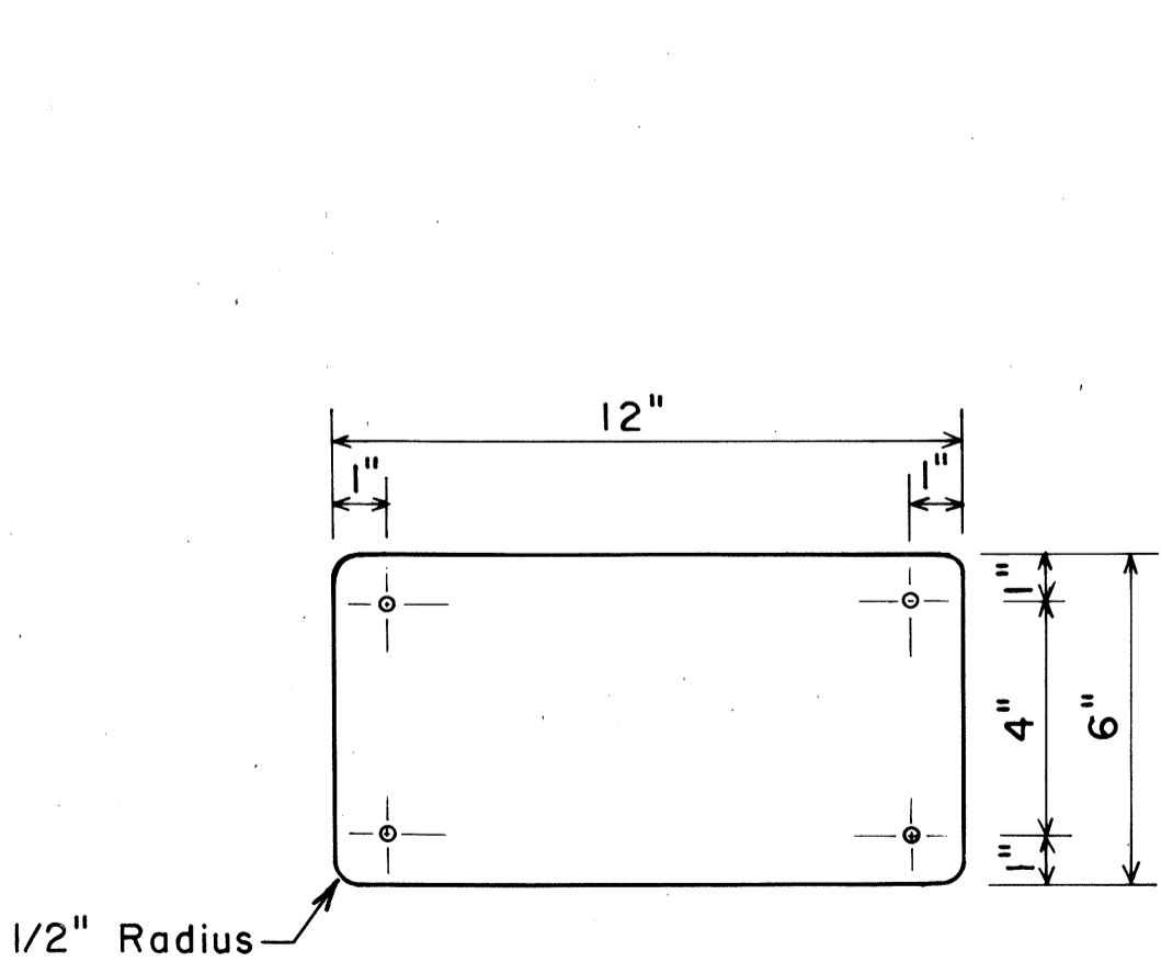
TYPE II OBJECT MARKER Not To Scale
