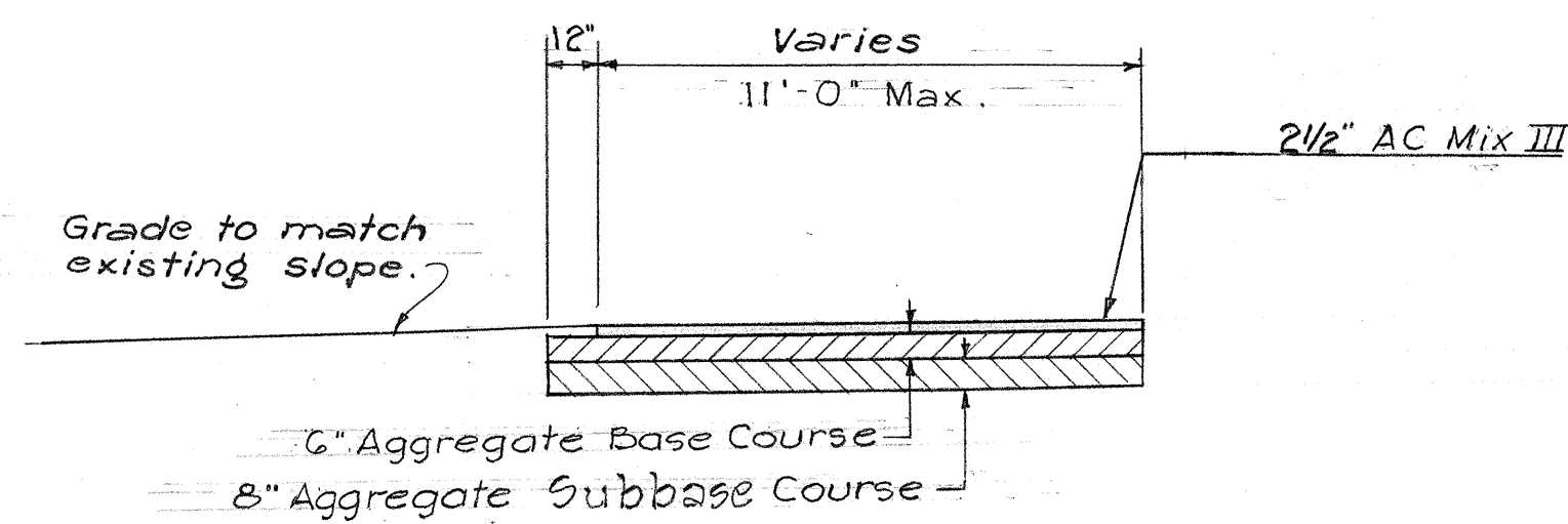
TYPICAL SECTION Scale 1/4" = 1'-0"
