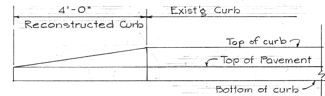
ELEVATION DETAIL OF RECONSTRUCTED CURB Not to scale
