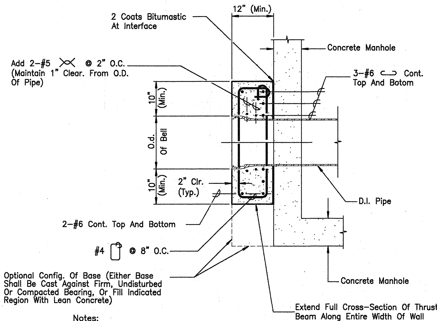
DETAIL - THRUST BEAM SCALE: 3/4" = 1'-0"
