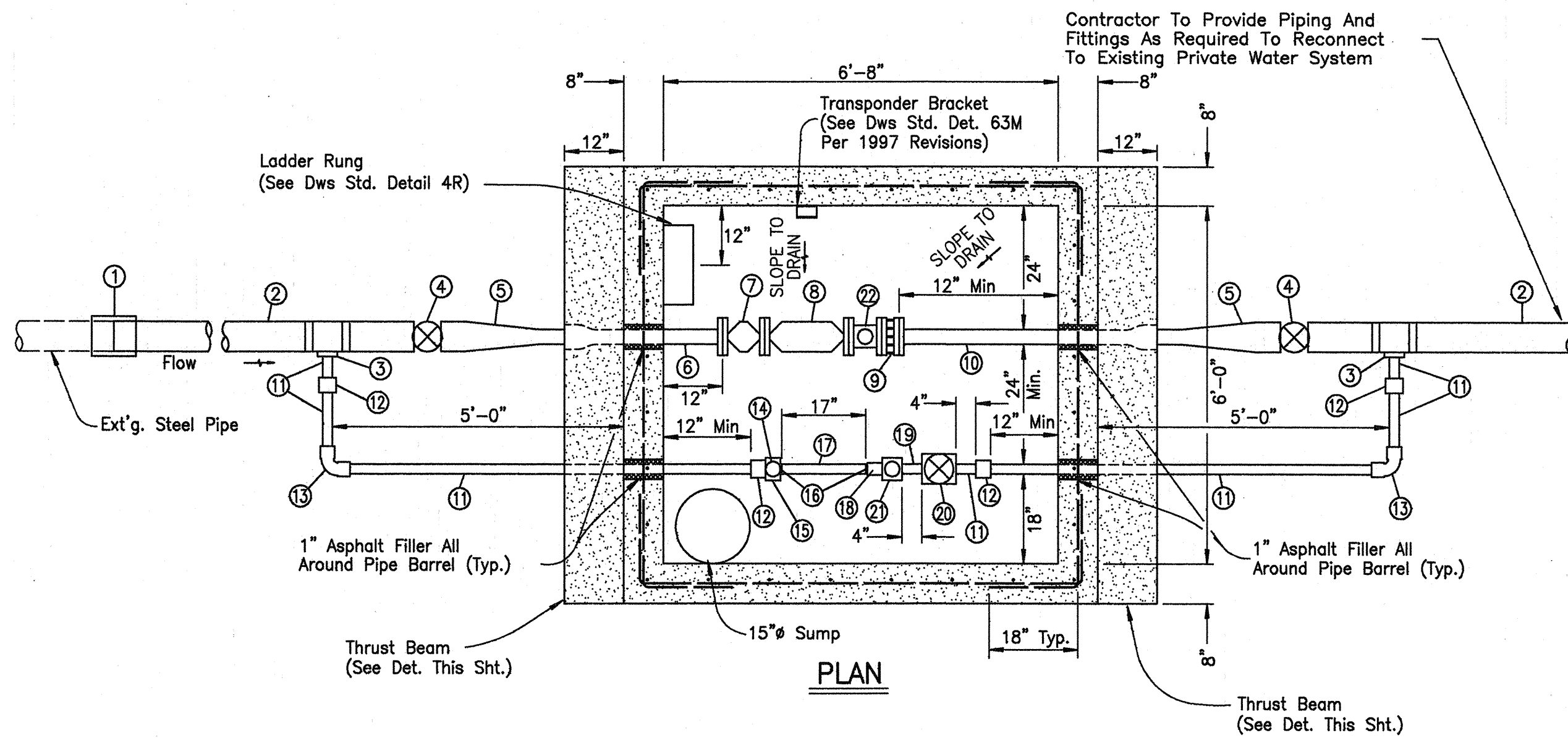
DETAILS - 3" WATER METER SCALE: 1/2" = 1'-0"
