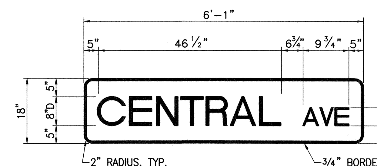
STREET NAME SIGN DETAIL NOT TO SCALE
