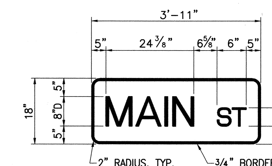
STREET NAME SIGN DETAIL NOT TO SCALE
