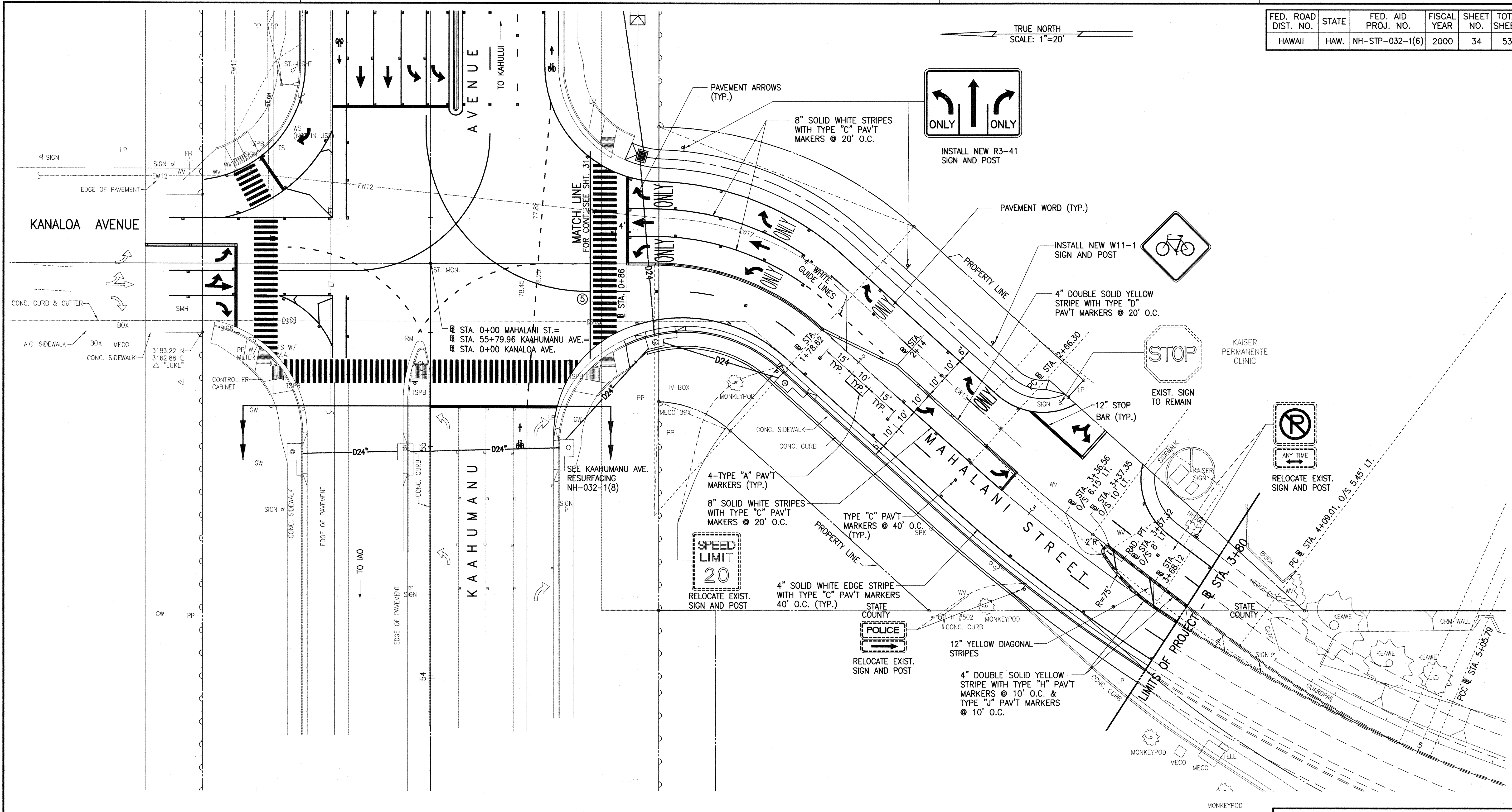
SIGN AND STRIPING PLAN SCALE: 1"=20'
