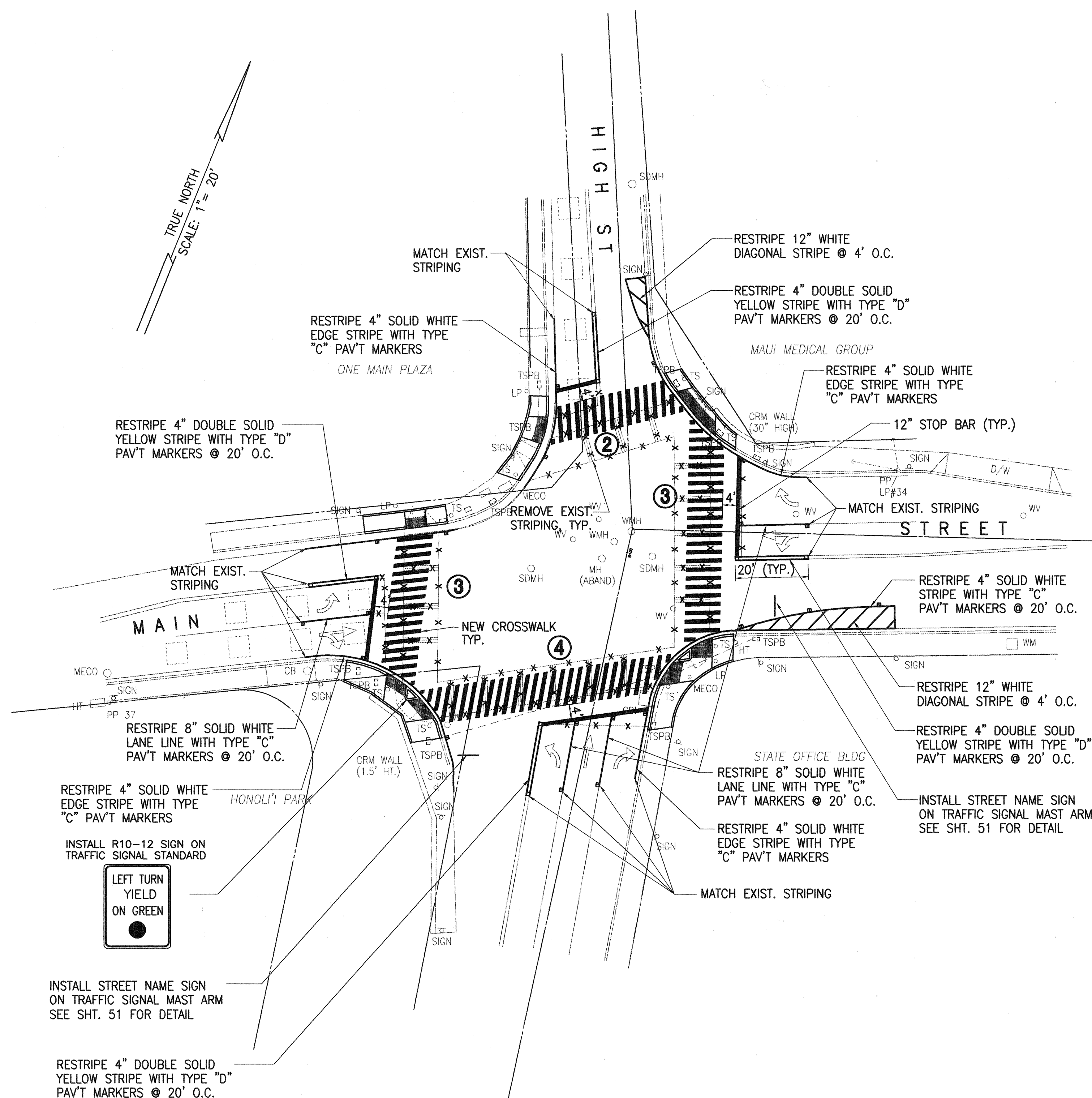
STRIPING PLAN SCALE: 1"=20'
