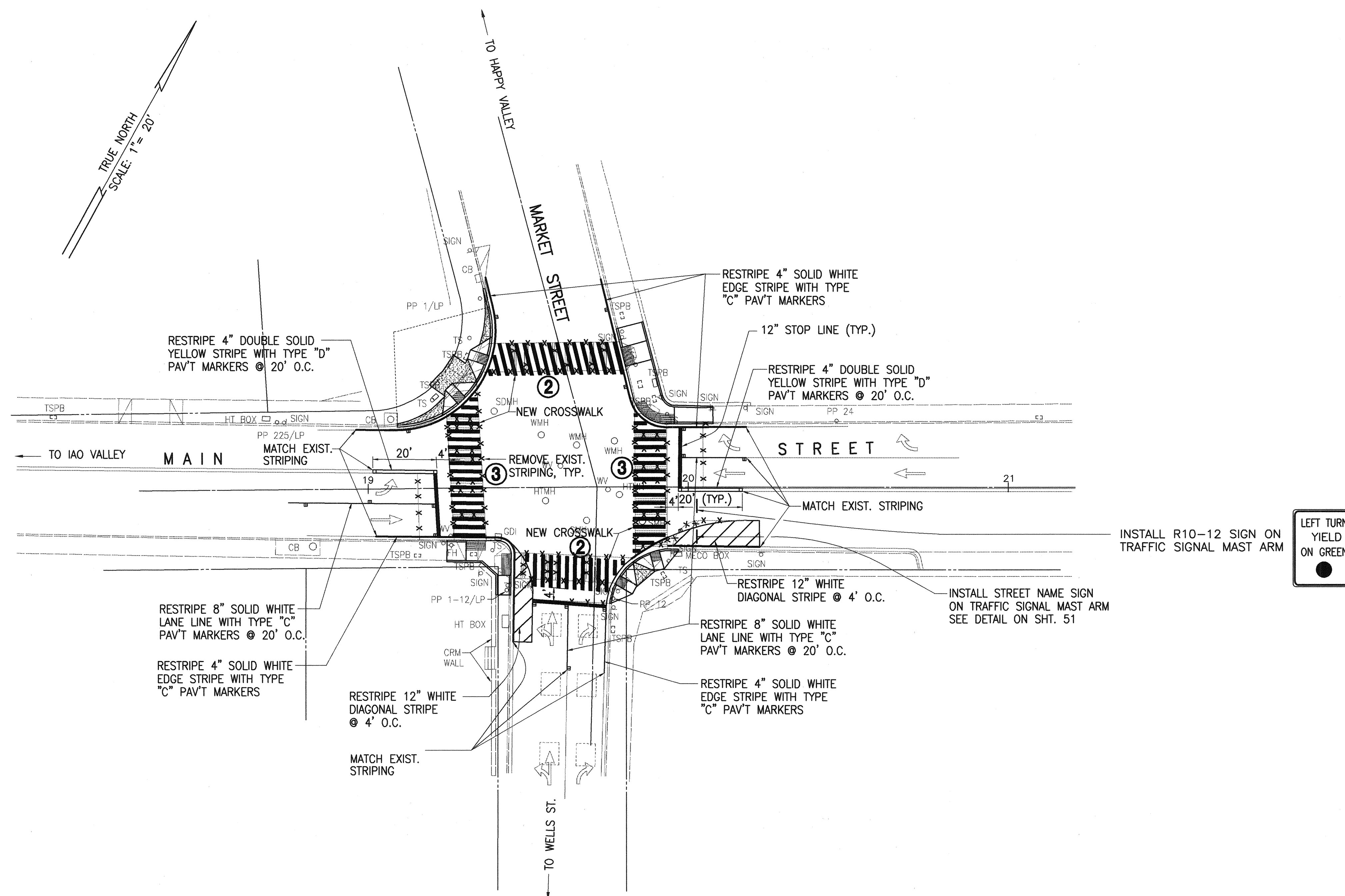
STRIPING PLAN SCALE: 1"=20'
