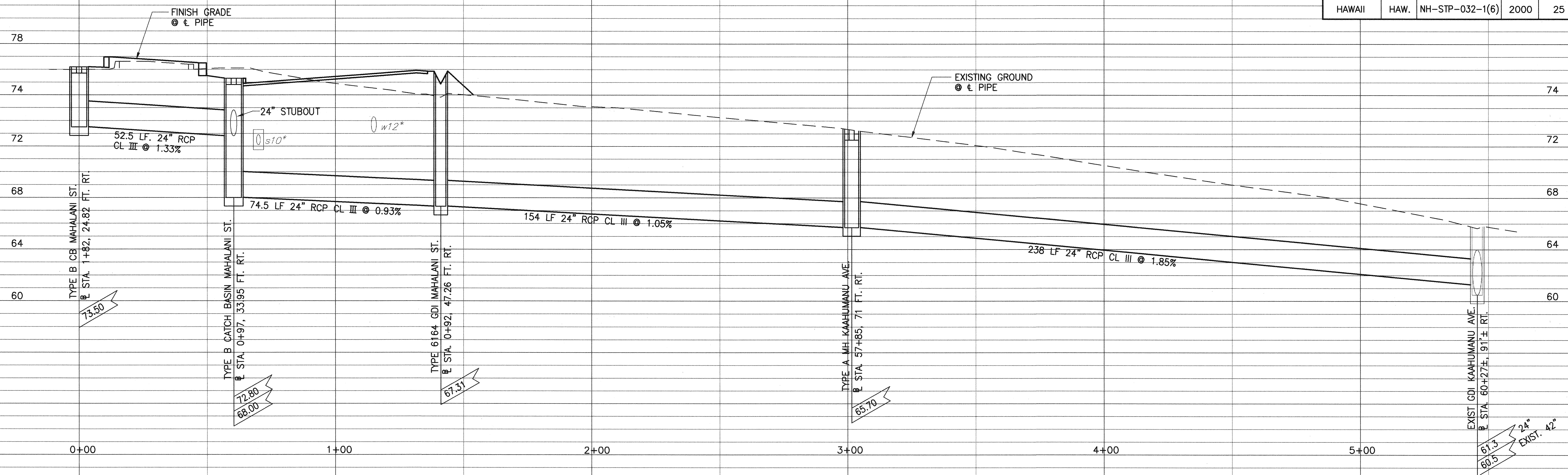
PROFILE - DRAIN LINE "A" SCALE: HORIZ. 1"=20' VERT. 1"=4'
