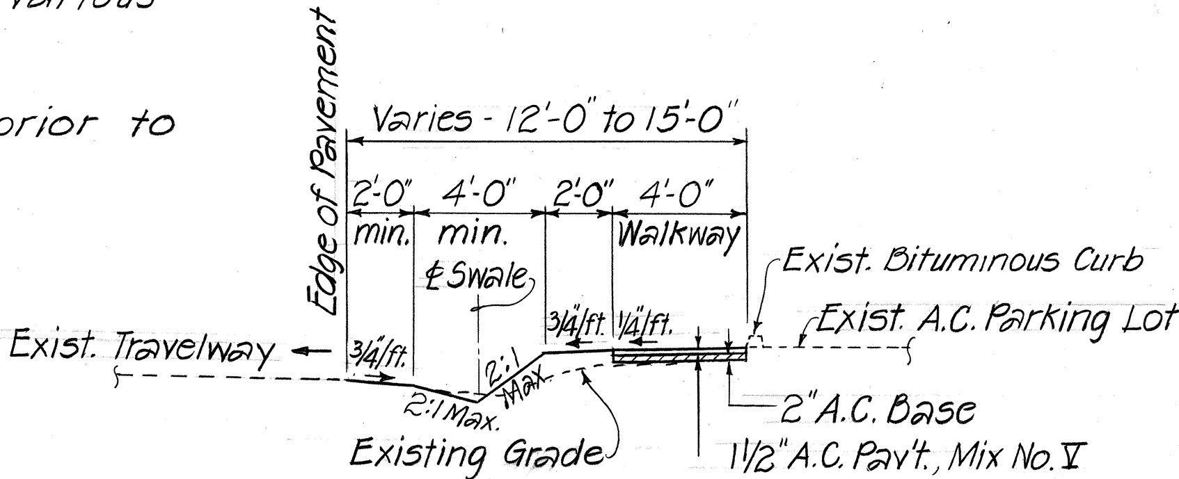
TYPICAL SECTION OF WALKWAY ALONG KAHULUI BEACH ROAD Scale: 1/4" = 1'-0"
