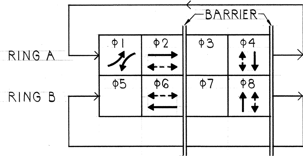
PHASE DIAGRAM
