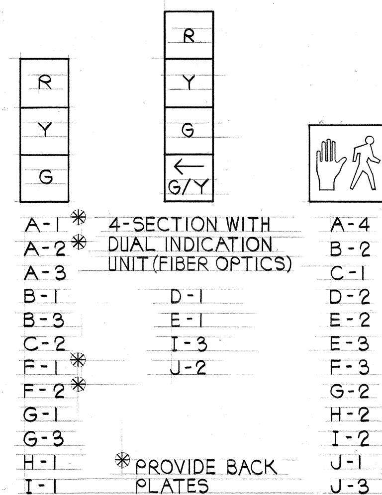
SIGNAL INDICATIONS
