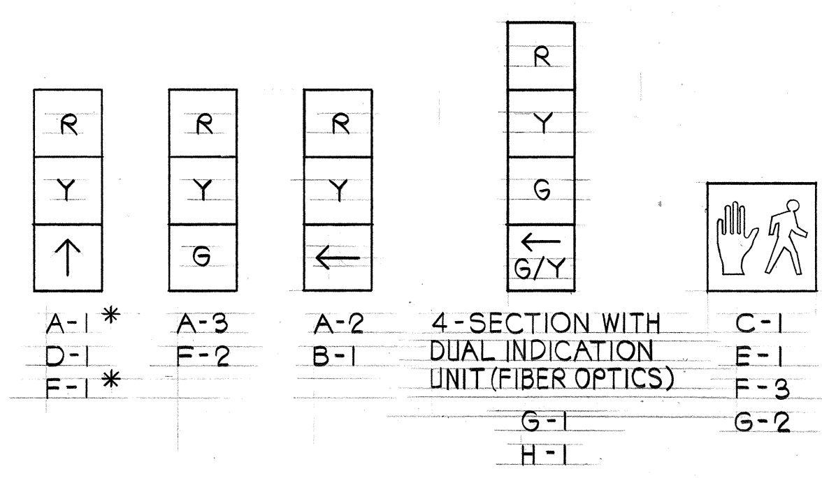
SIGNAL INDICATIONS
