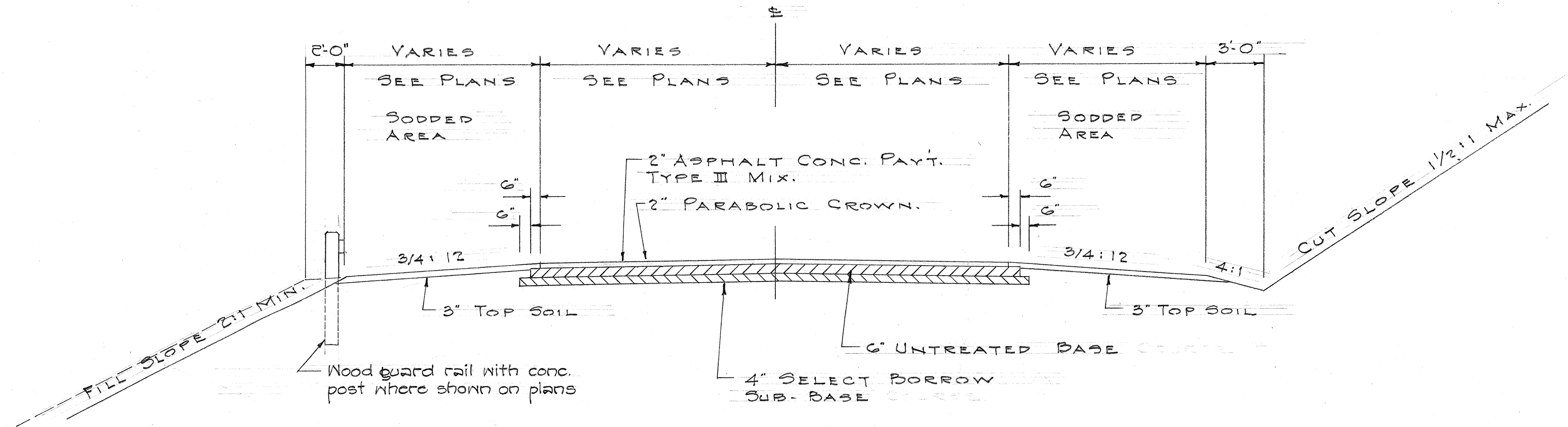
TYPICAL SECTIONS ON TANGENTS APPROACH ROADS SCALE: 1/4" = 1'-0"
