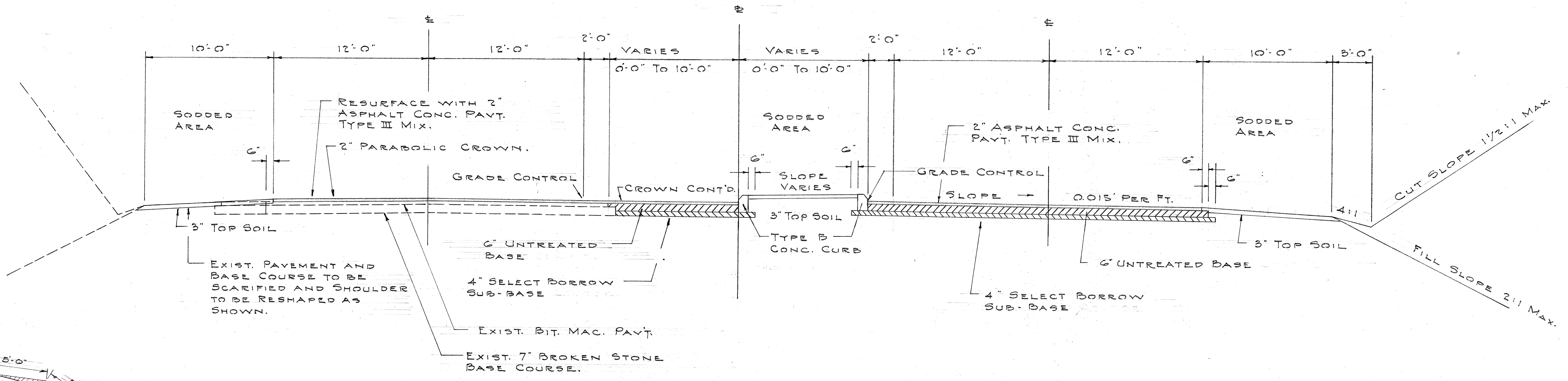
TYPICAL SECTION ON TANGENT NON-CONTINUOUS CURB SCALE: 1/4" = 1'-0"
