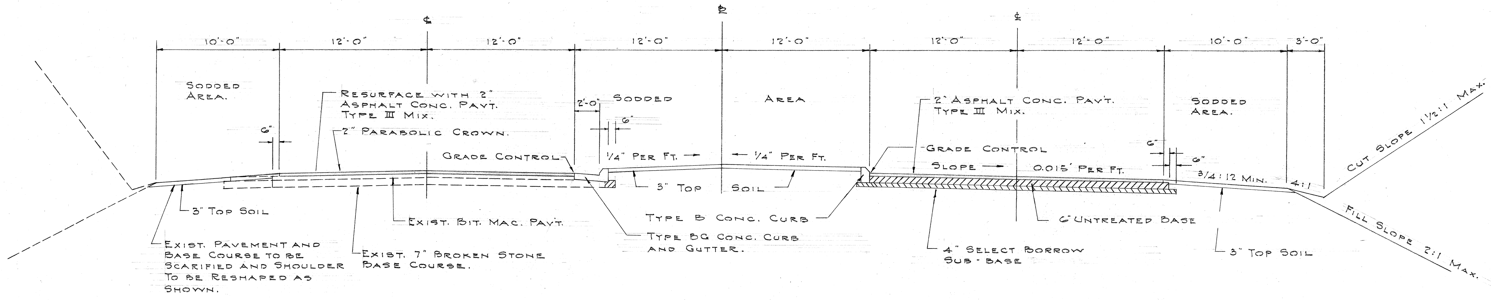
TYPICAL SECTION ON TANGENT CONTINUOUS CURB SCALE: 1/4" = 1'-0"
