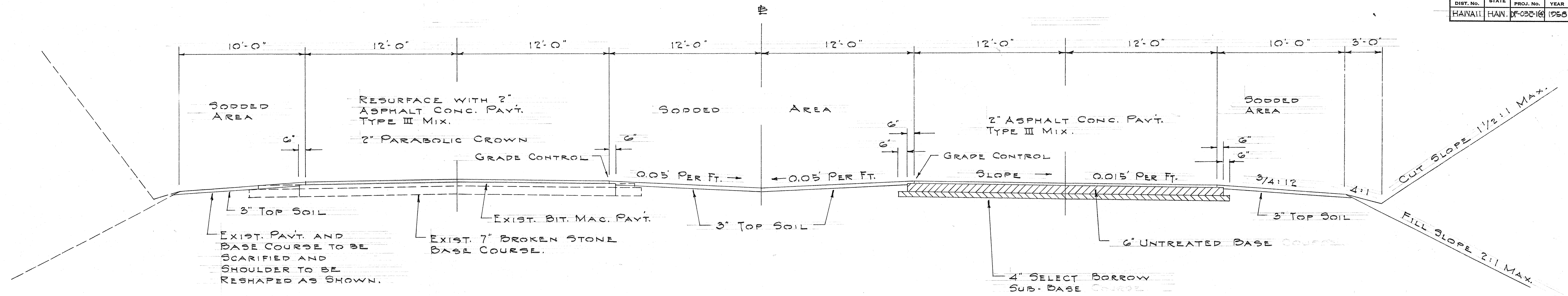
TYPICAL SECTION ON TANGENT WITHOUT CURB SCALE: 1/4" = 1'-0"
