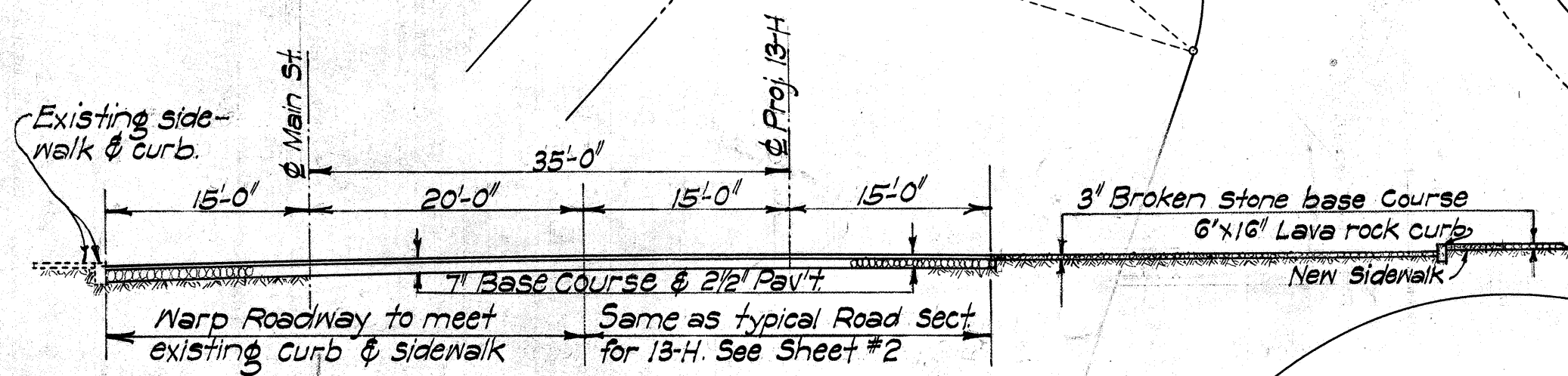
SECT. A-A Scale 3/32"=1'-0"
