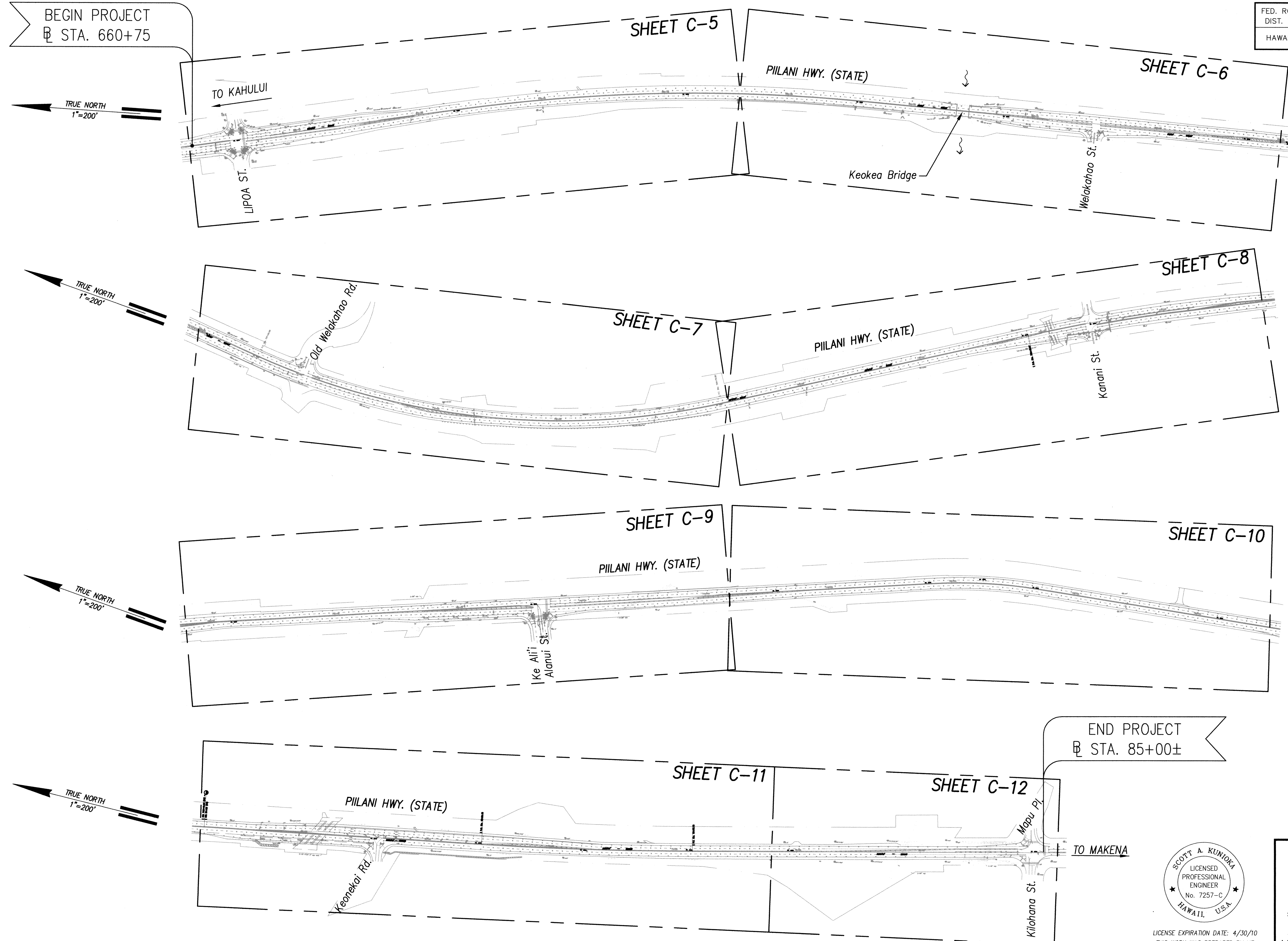
GENERAL PLAN SCALE: 1" = 200'
