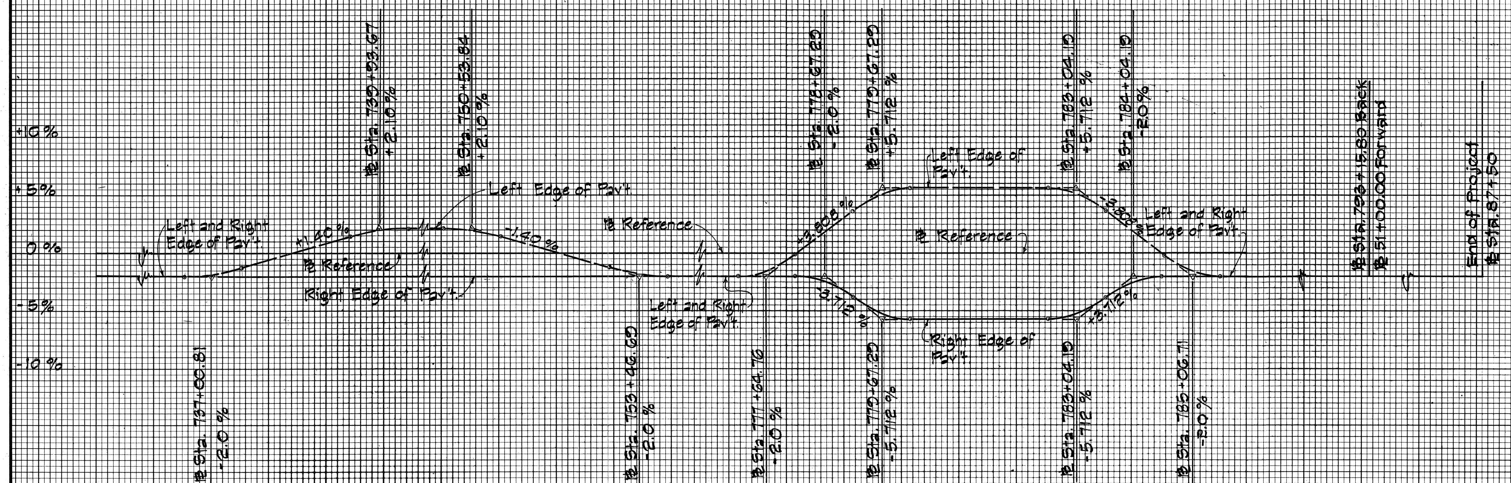
SUPERELEVATION FOR LEFT AND RIGHT EDGE OF PAVEMENT
