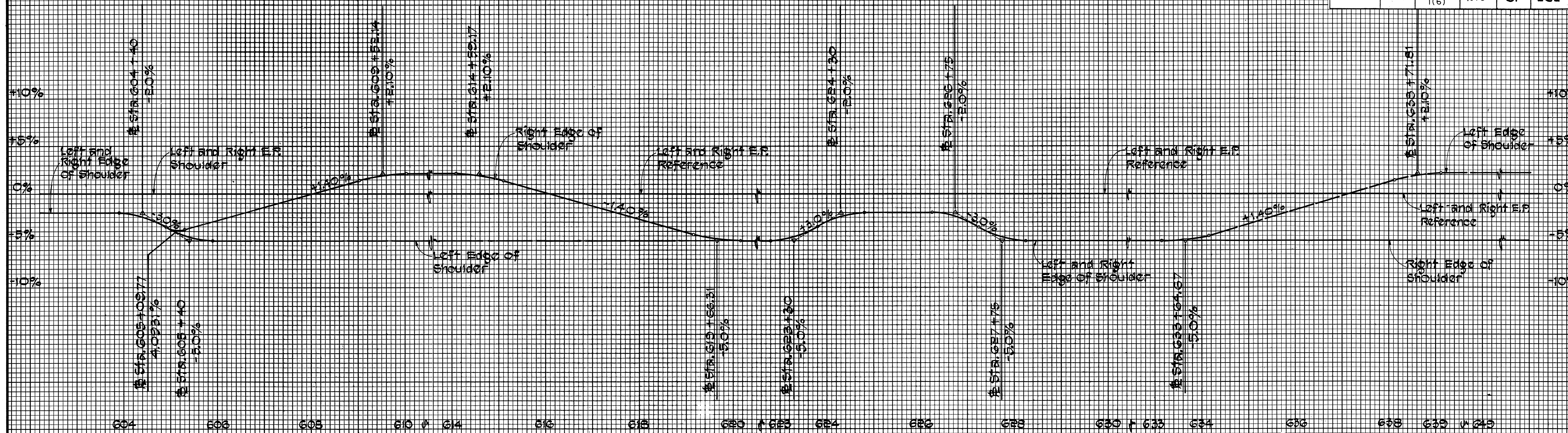
SUPERELEVATION FOR LEFT AND RIGHT EDGE OF SHOULDER
