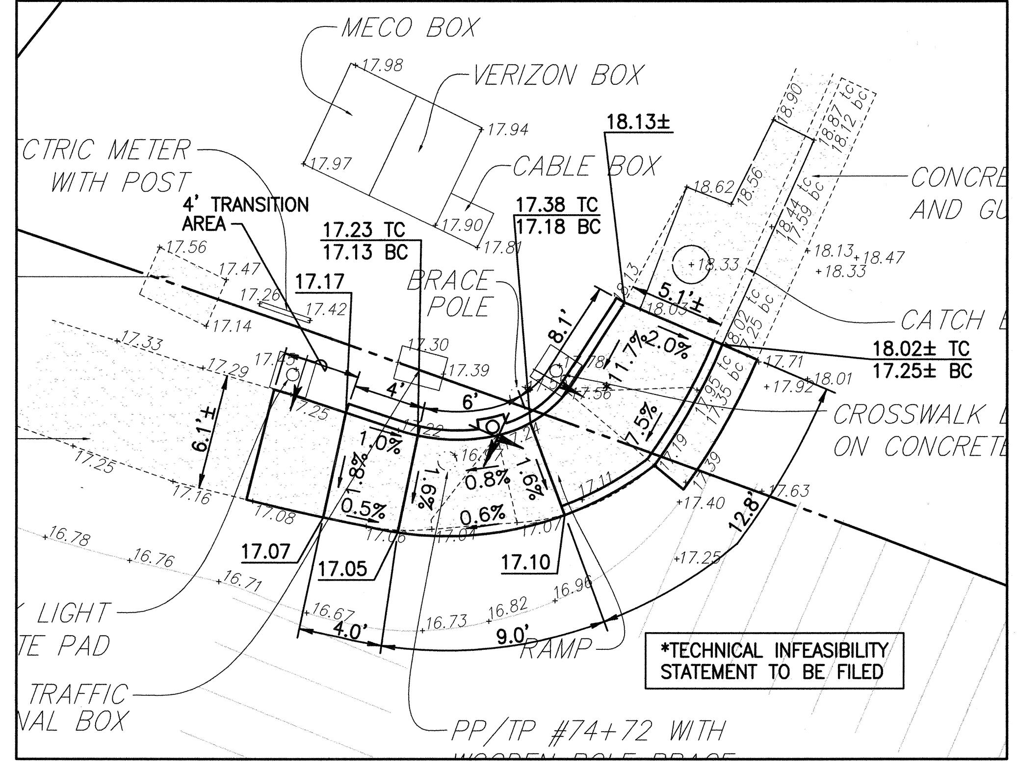
CURB RAMP NO. 40304-2 DETAILS SCALE: 1"= 5'
