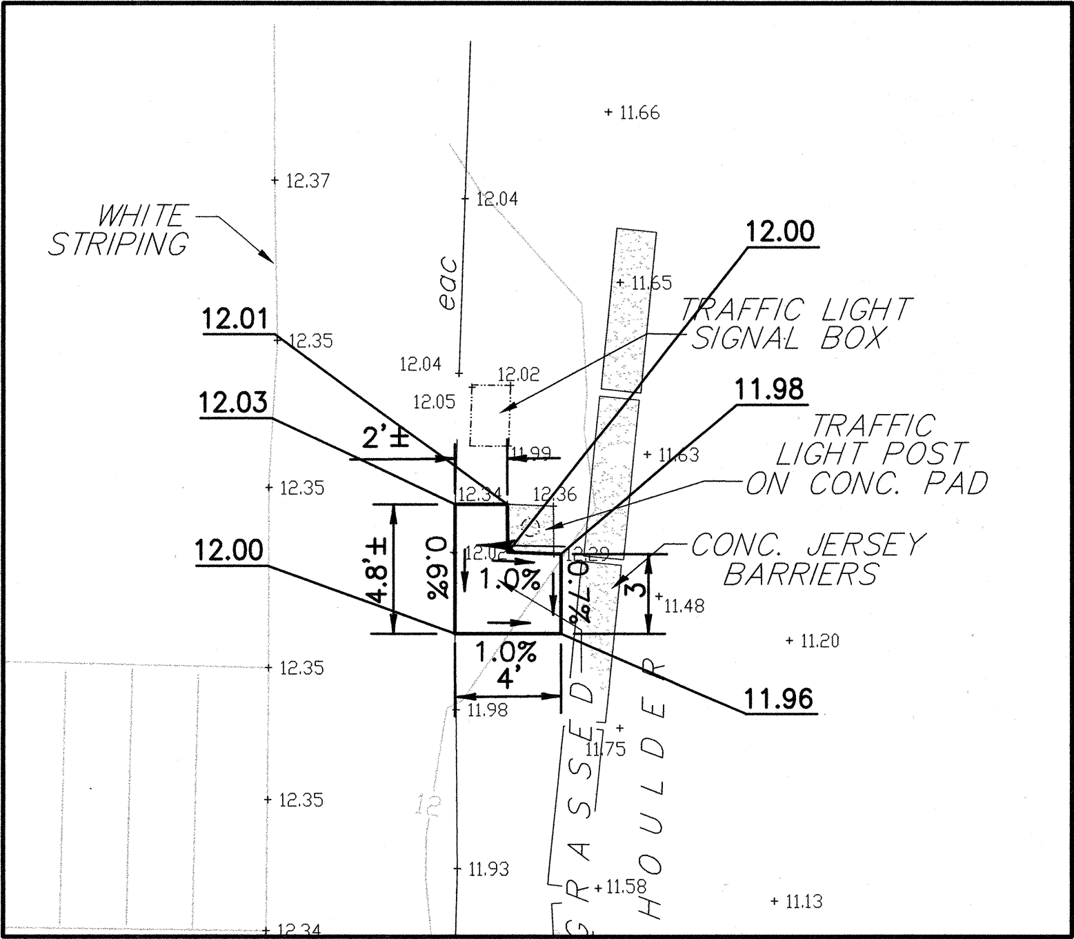
A.C. SIDEWALK NO. 32304-5 DETAILS SCALE: 1"= 5'
