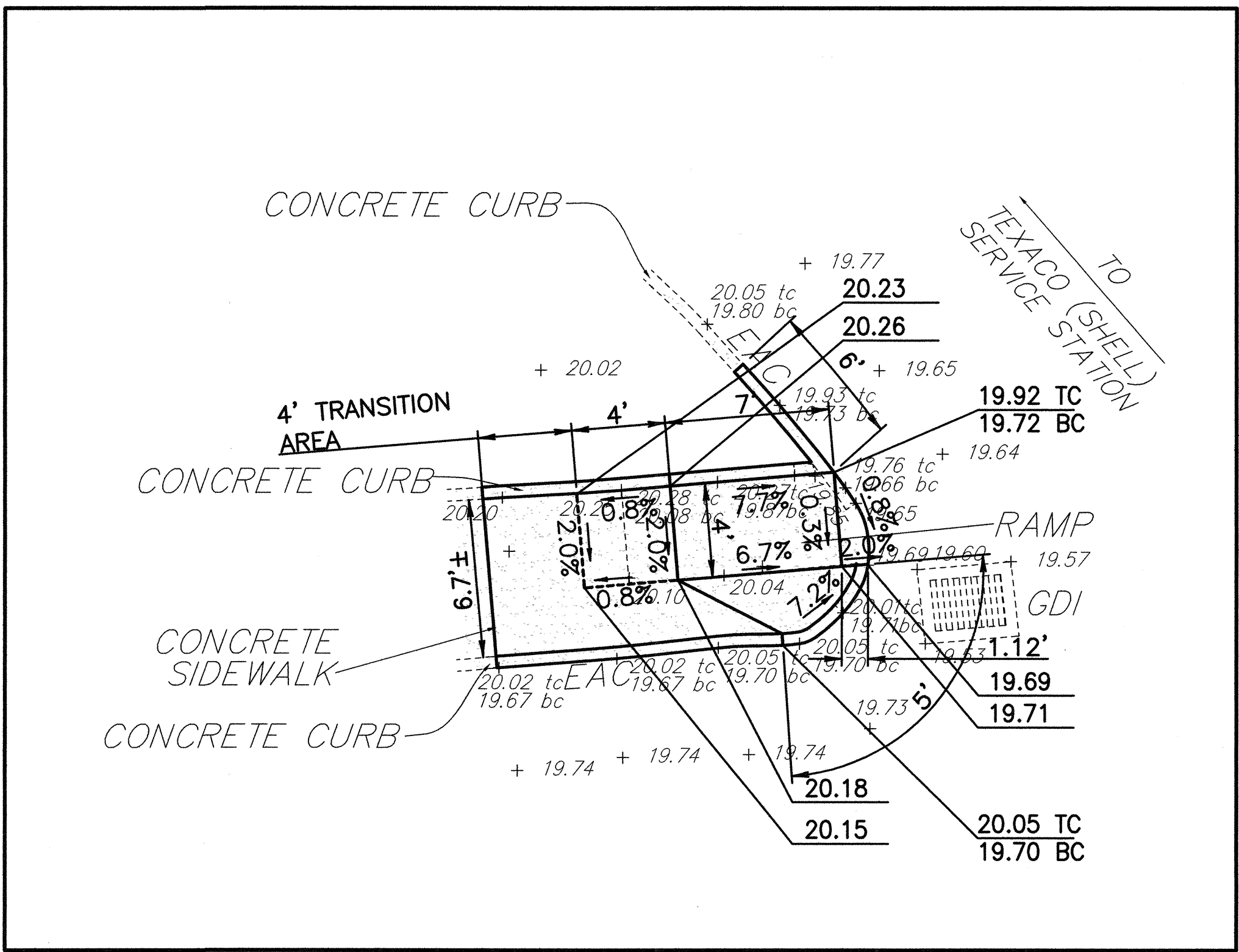
CURB RAMP NO. 61204-1 DETAILS SCALE: 1" = 5'
