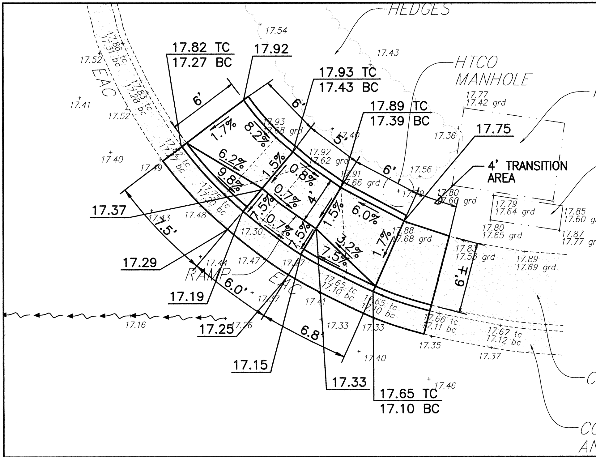
CURB RAMP NO. 20304-2 DETAILS SCALE: 1"= 5'
