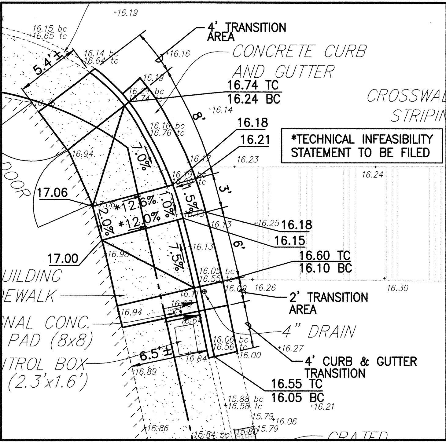
CURB RAMP NO. 50204-3 DETAILS SCALE: 1"= 5'
