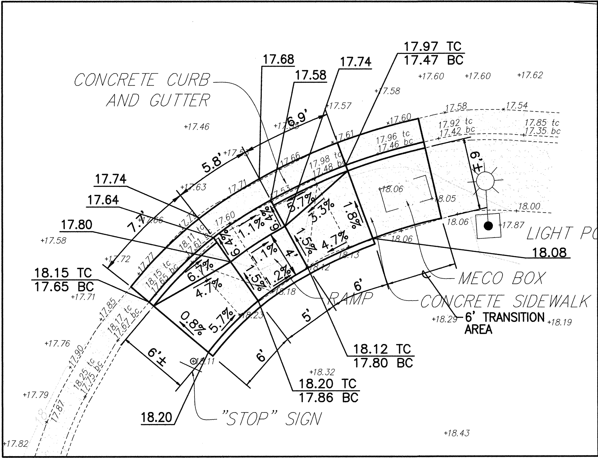
CURB RAMP NO. 20304-3 DETAILS SCALE: 1"= 5'
