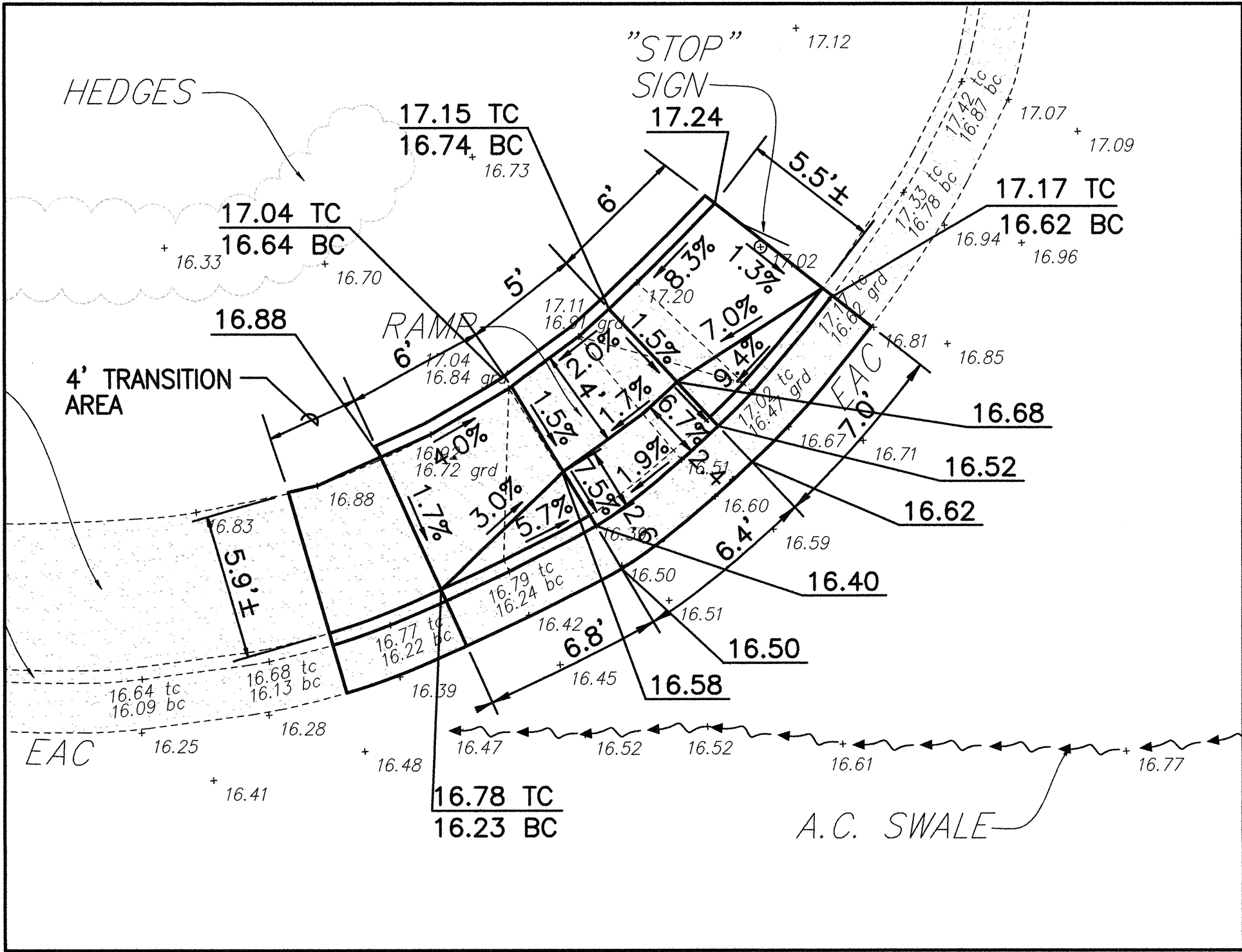
CURB RAMP NO. 20304-1 DETAILS SCALE: 1"= 5'
