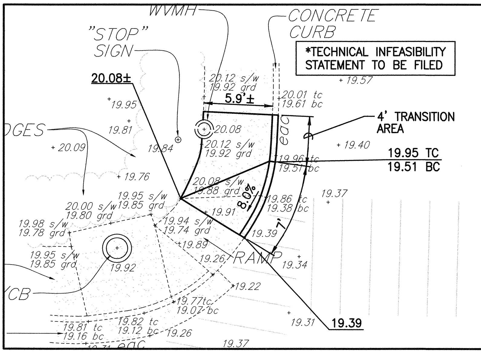
CURB RAMP NO. 62104-1 DETAILS SCALE: 1"= 5'
