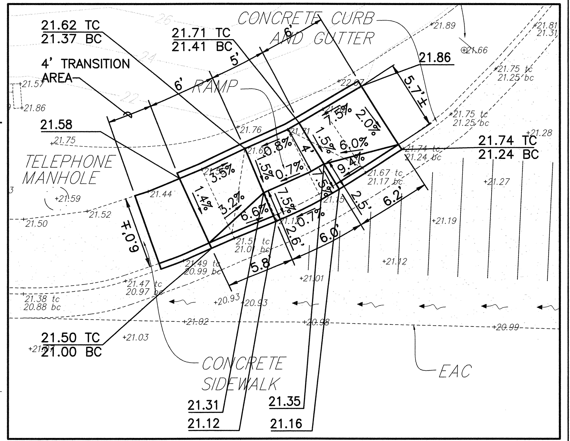
CURB RAMP NO. 20404-1 DETAILS SCALE: 1"= 5'
