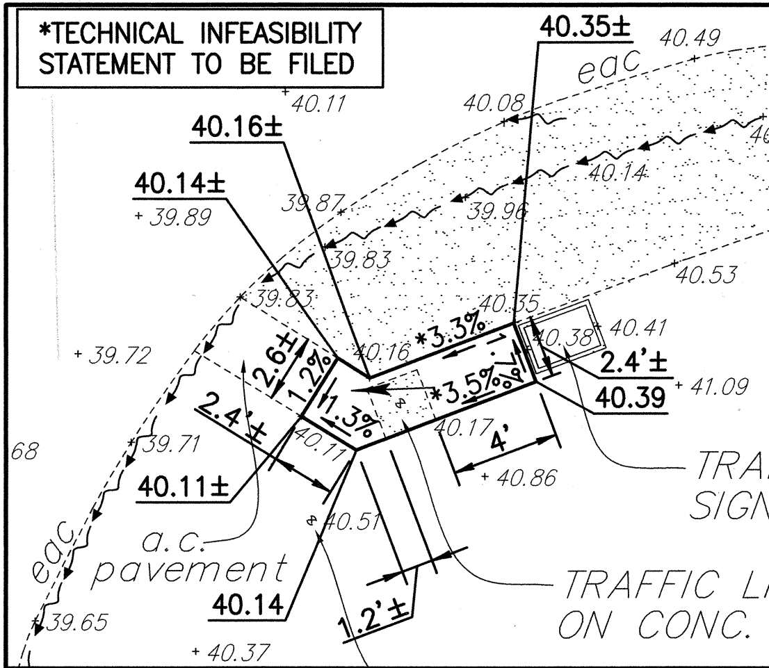
SIDEWALK NO. 40904-3 DETAILS SCALE: 1"= 5'
