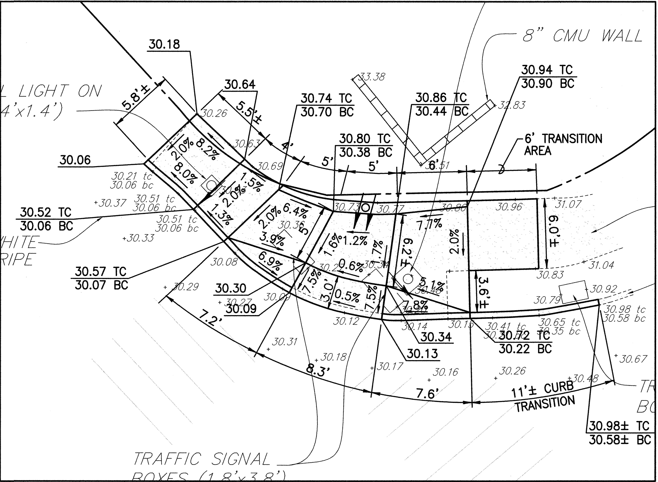
CURB RAMP NO. 32704-1 DETAILS
