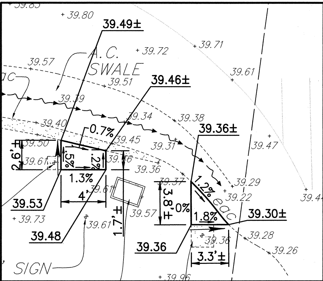
SIDEWALK NO. 40904-4 DETAILS SCALE: 1"= 5'
