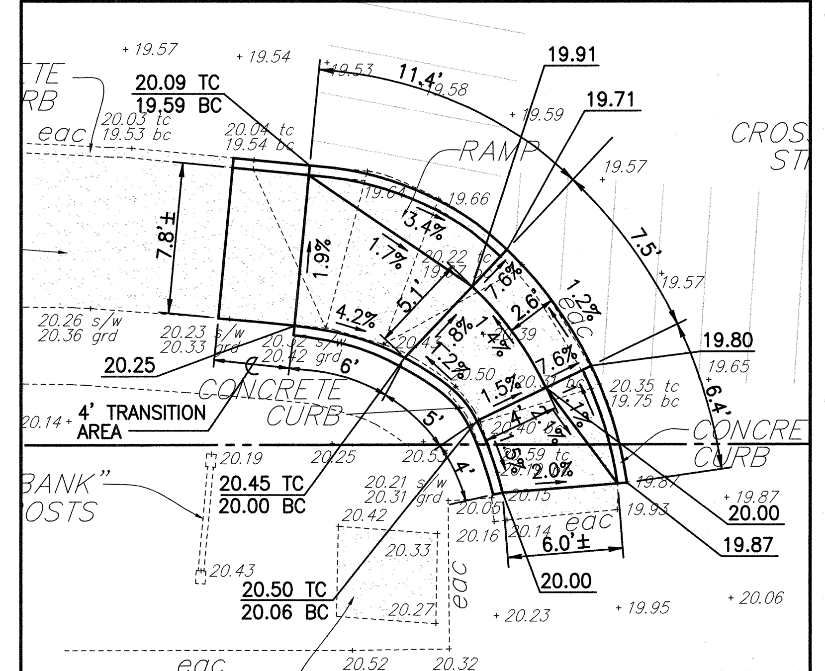
CURB RAMP NO. 62104-4.5 DETAILS SCALE: 1"= 5'
