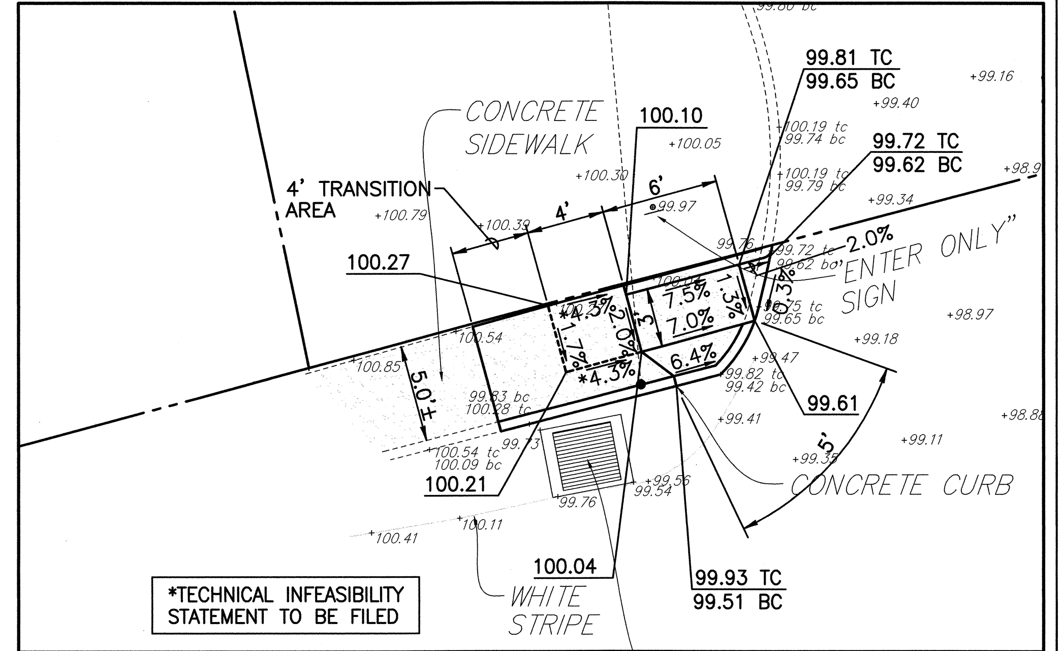
CURB RAMP NO. 10604-1 DETAILS
