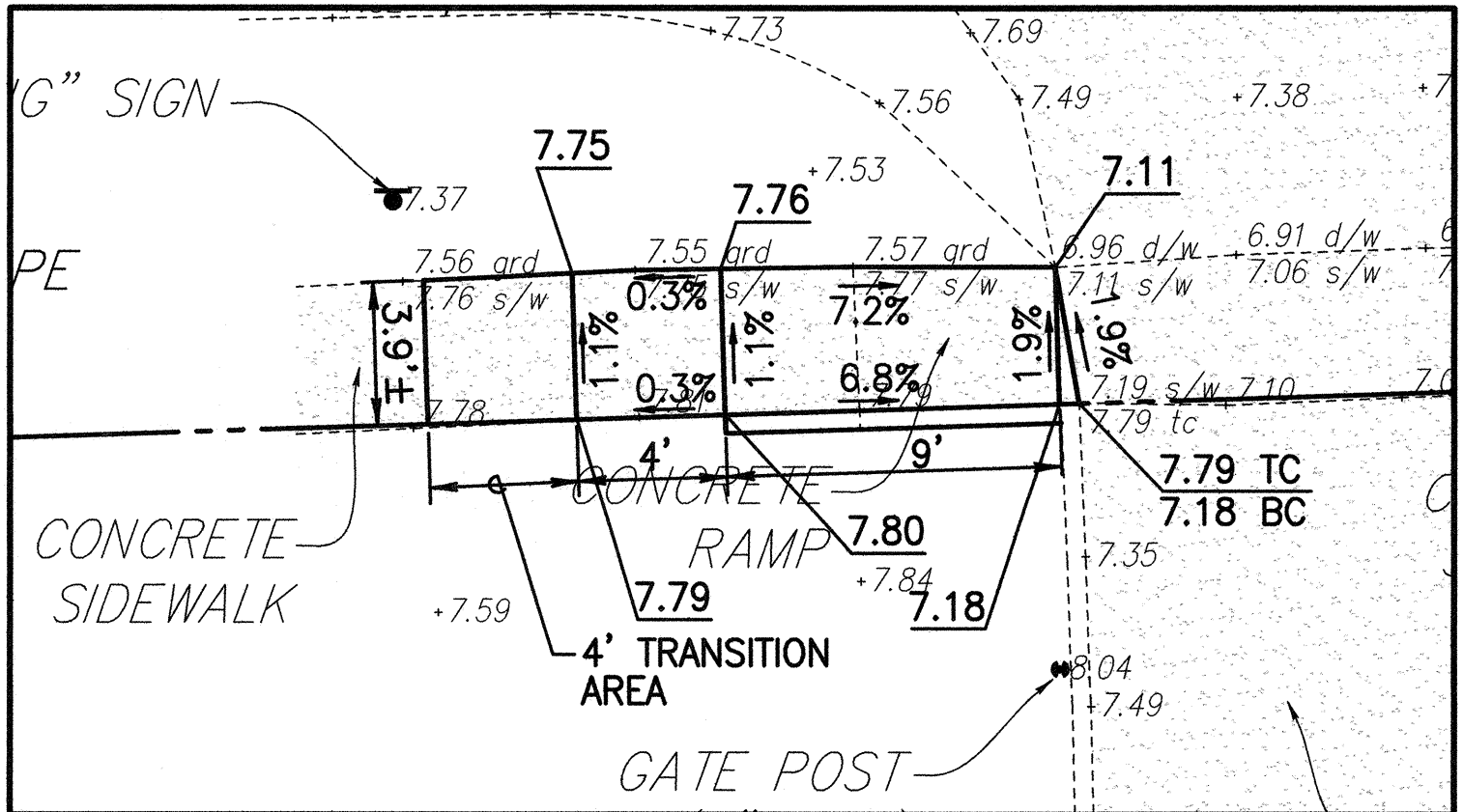
CURB RAMP NO. 30404-1 DETAILS SCALE: 1"= 5'
