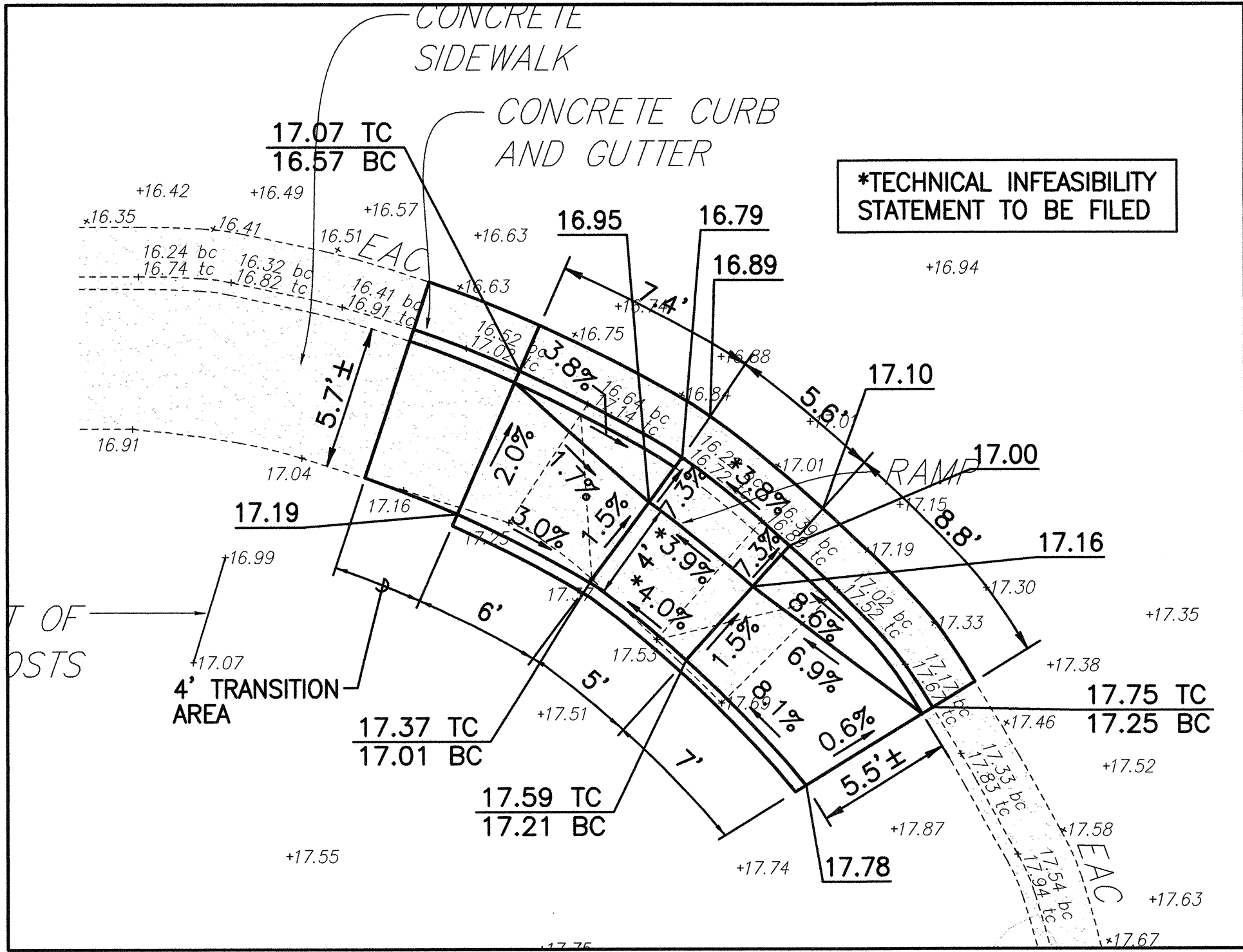
CURB RAMP NO. 20304-4 DETAILS SCALE: 1"= 5'
