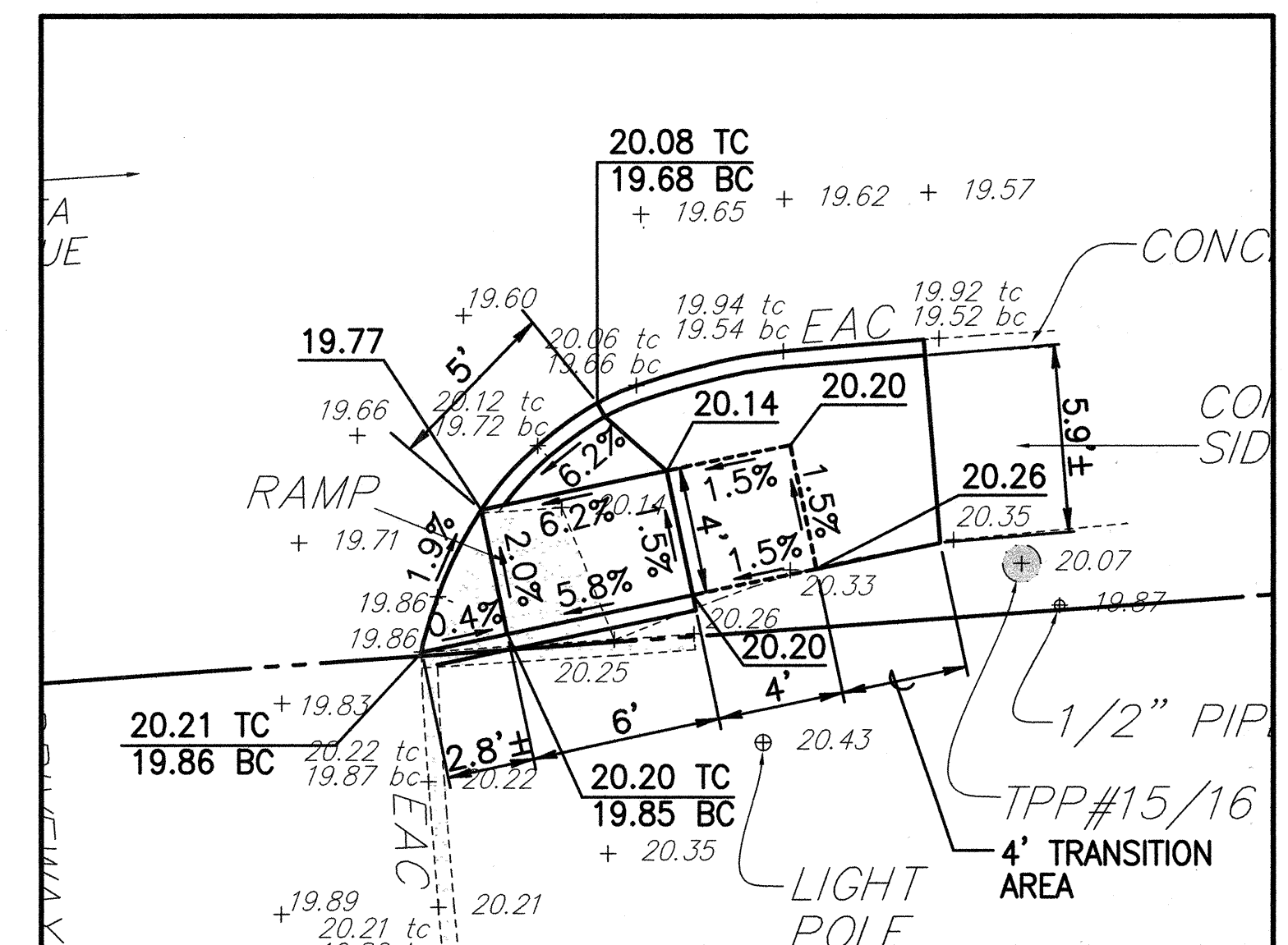
CURB RAMP NO. 61304-1 DETAILS SCALE: 1" = 5'
