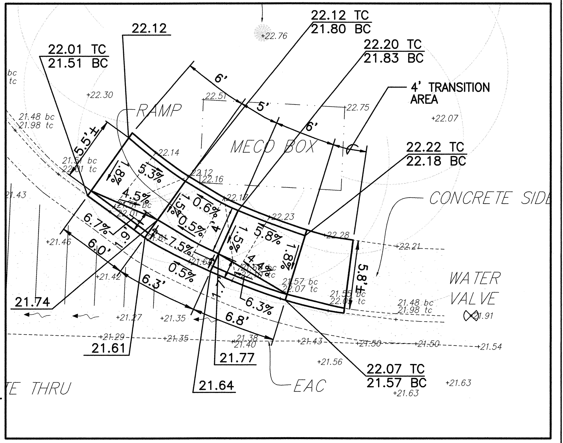
CURB RAMP NO. 20404-2 DETAILS SCALE: 1"= 5'
