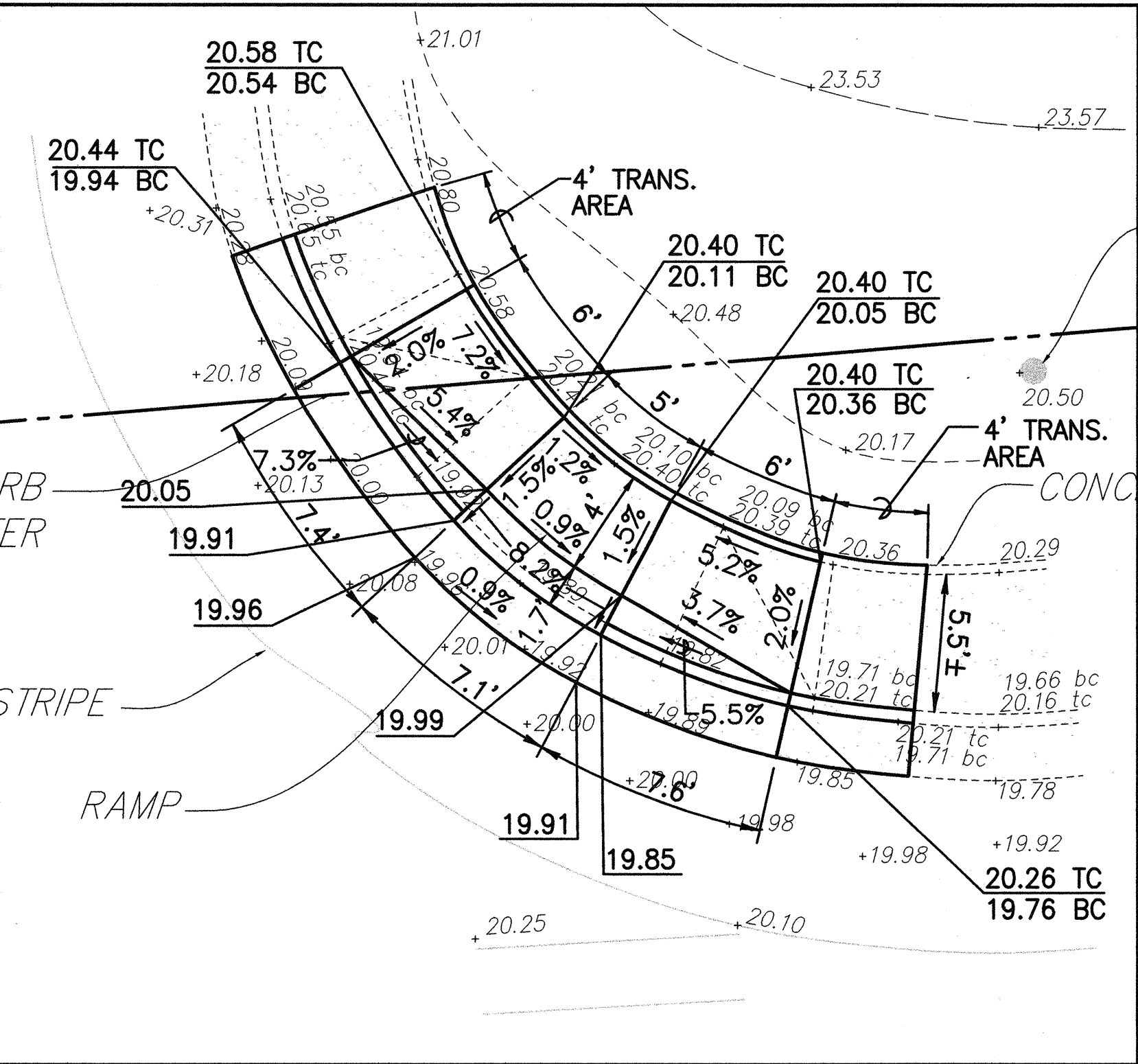
CURB RAMP NO. 40404-1 DETAILS SCALE: 1"= 5'
