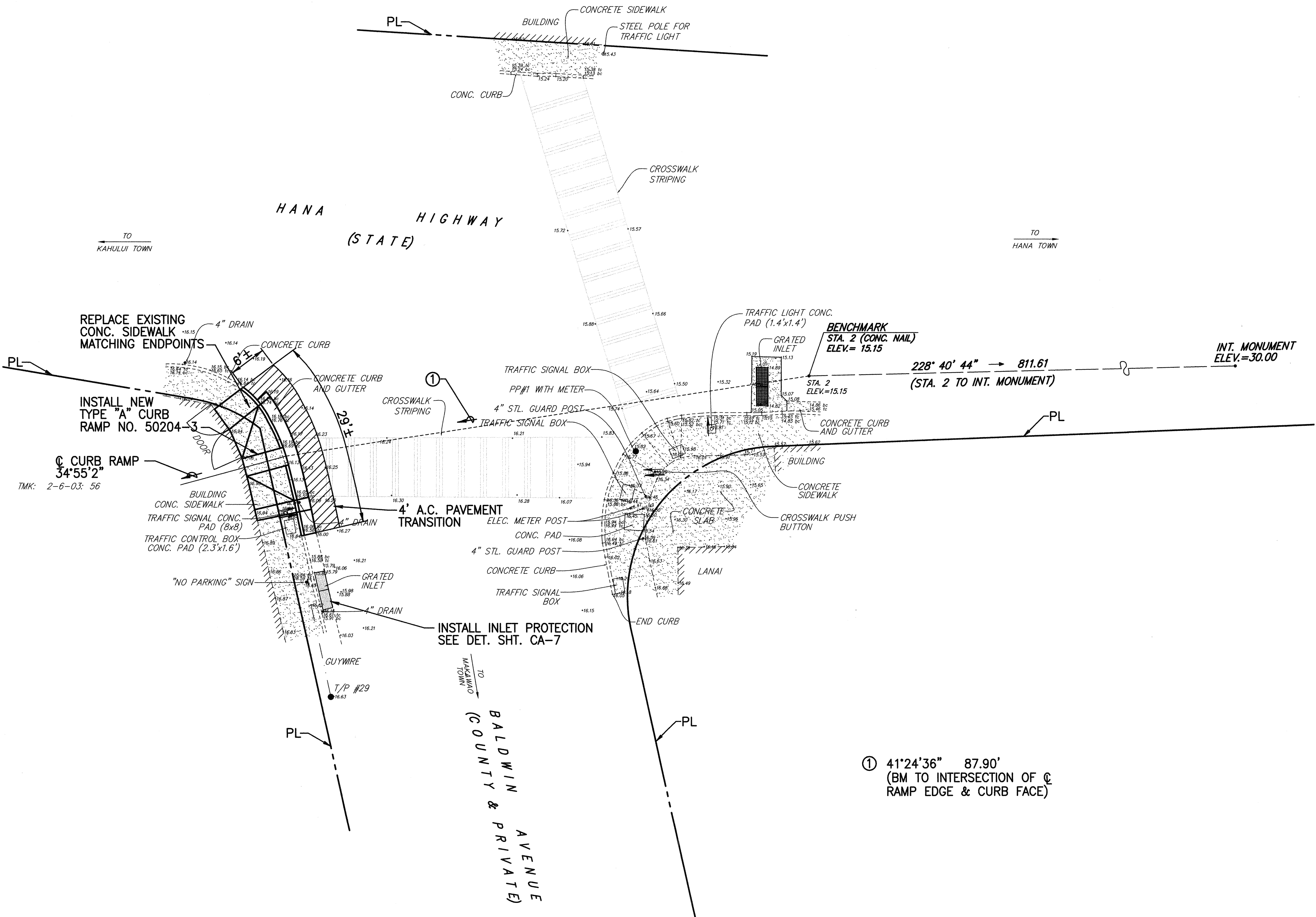
SITE PLAN SCALE: 1"= 10' NORTH
