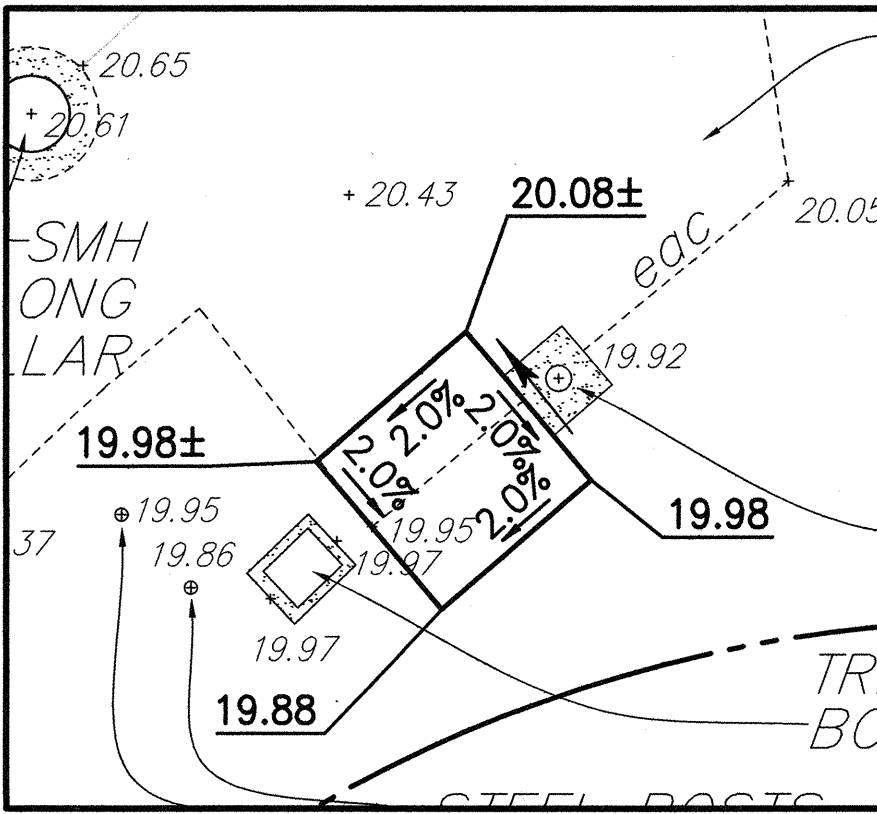
A.C. SIDEWALK NO. 40504-1 DETAILS SCALE: 1"= 5'
