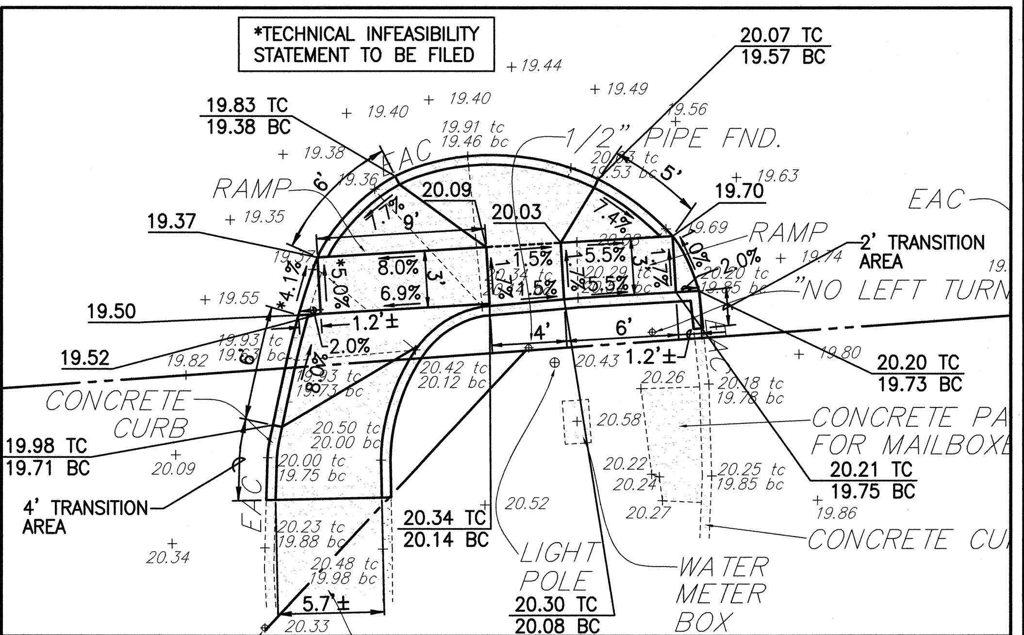
CURB RAMP NO. 61504-2/61604-1 DETAILS SCALE: 1"= 5'
