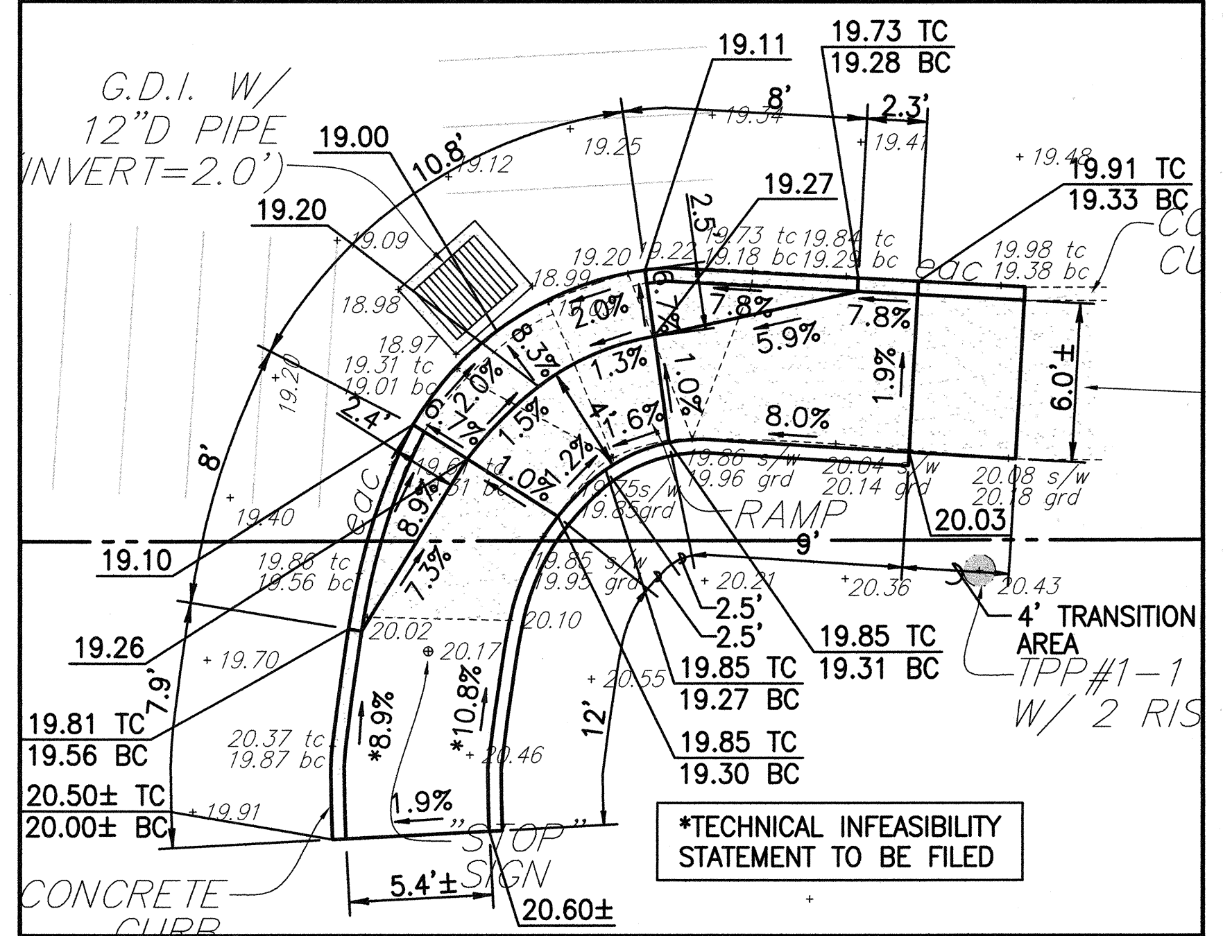
CURB RAMP NO. 62104-3 DETAILS SCALE: 1"= 5'
