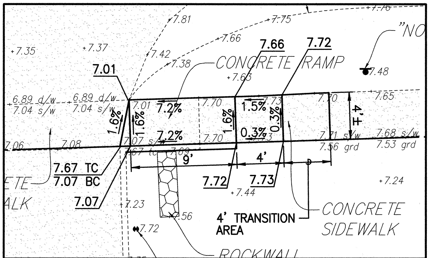
CURB RAMP NO. 30404-2 DETAILS SCALE: 1"= 5'
