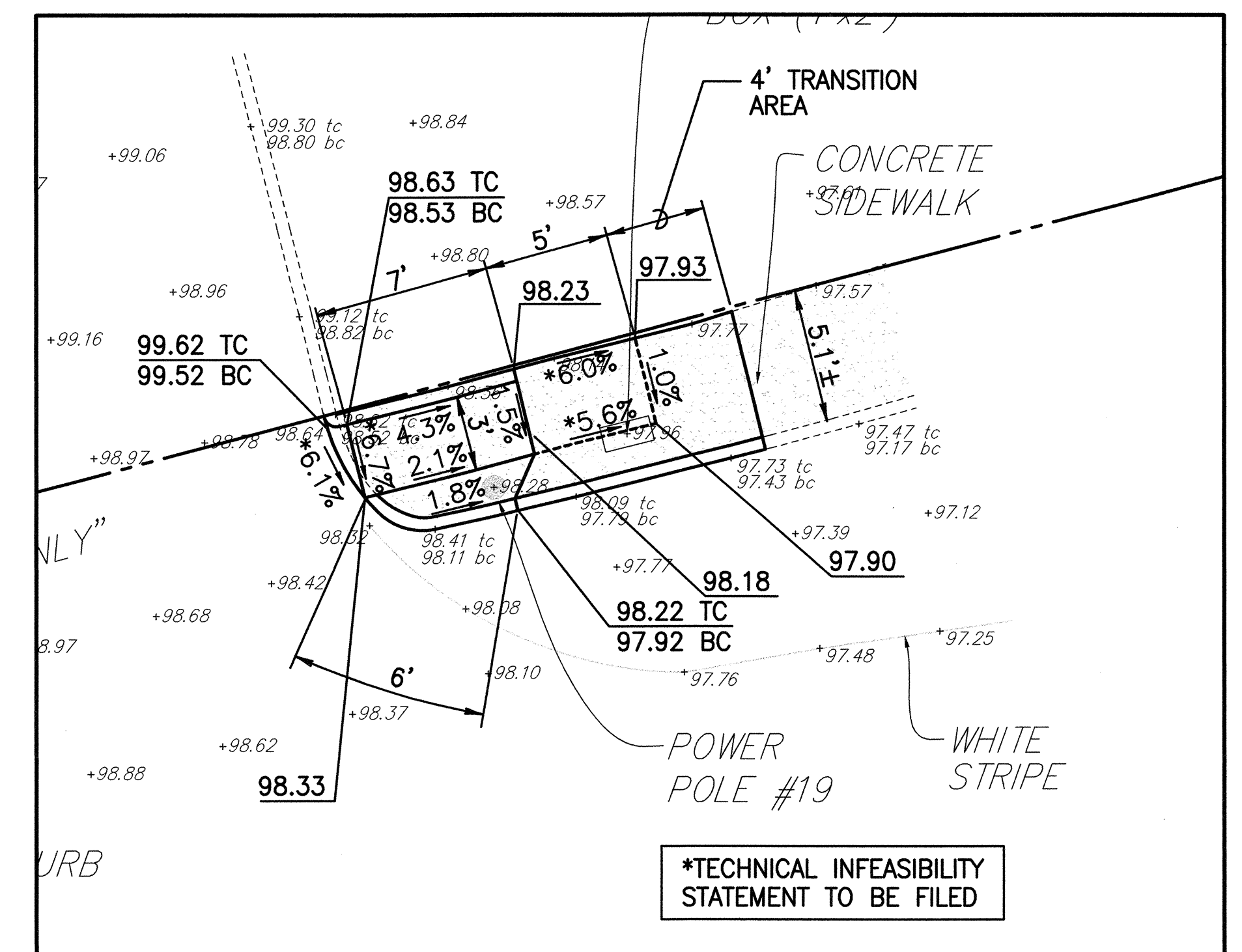
CURB RAMP NO. 10604-2 DETAILS
