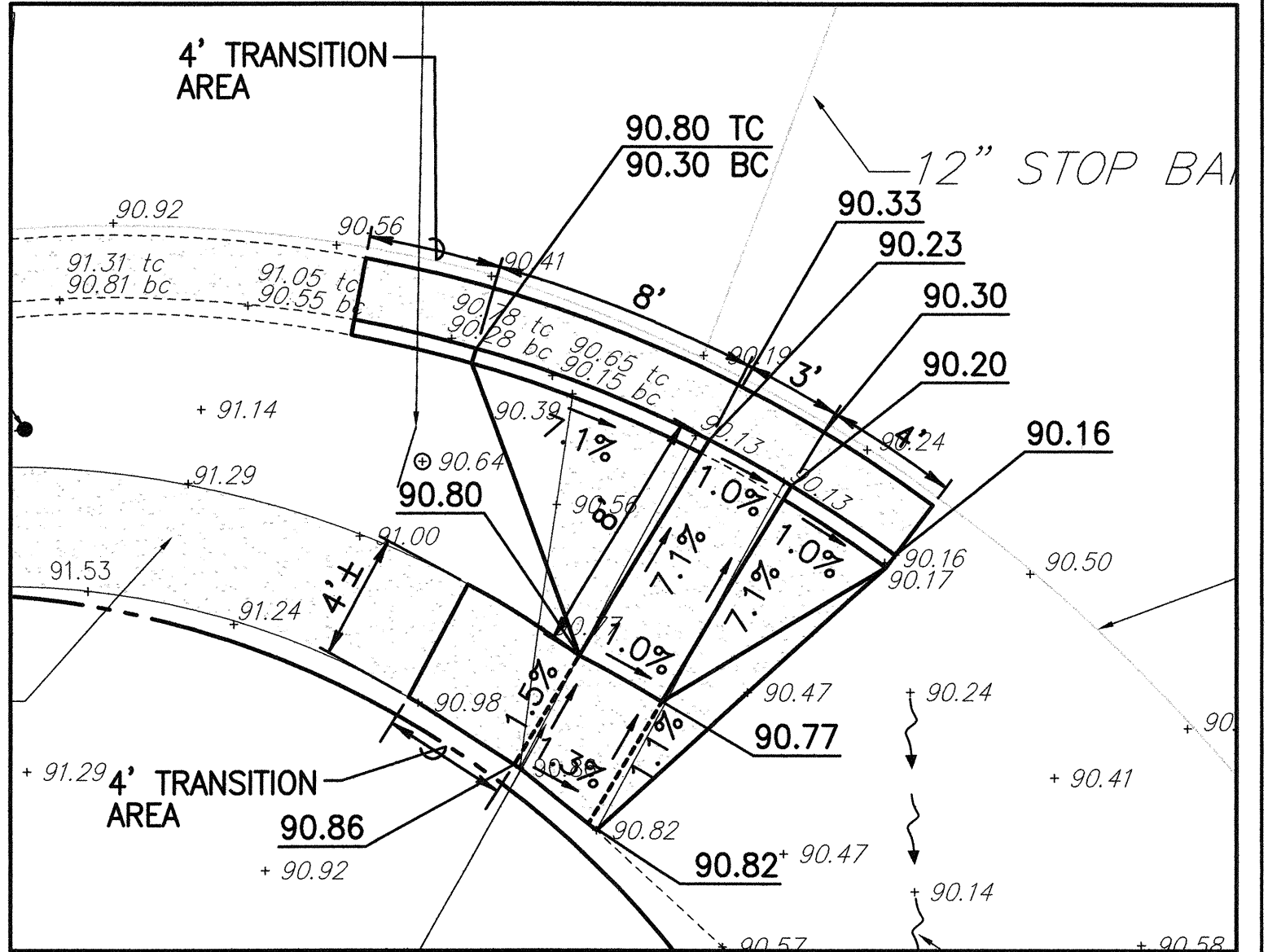
CURB RAMP NO. 22304-1 DETAILS SCALE: 1"= 5'
