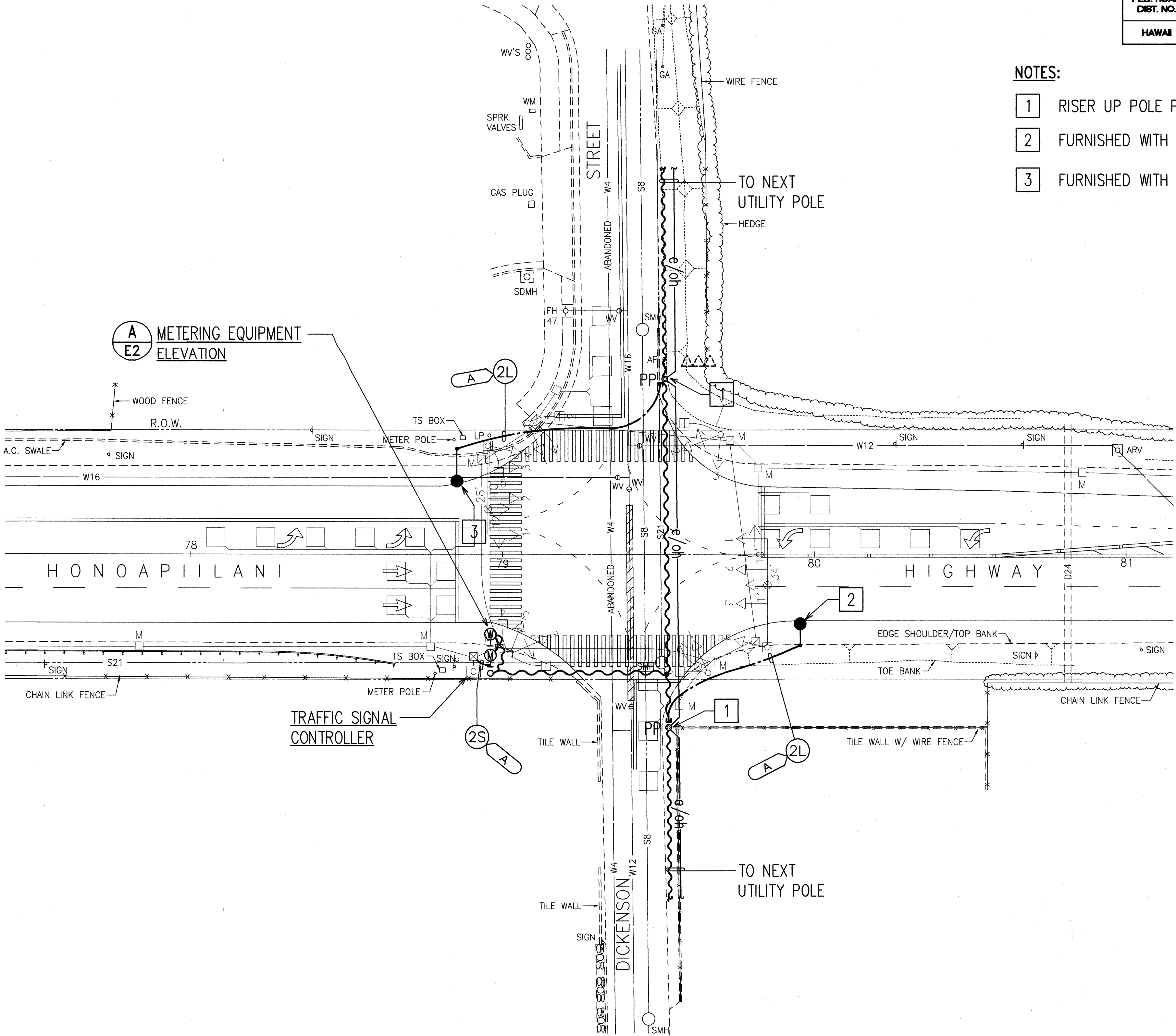
ELECTRICAL SITE PLAN SCALE: 1"=20'
