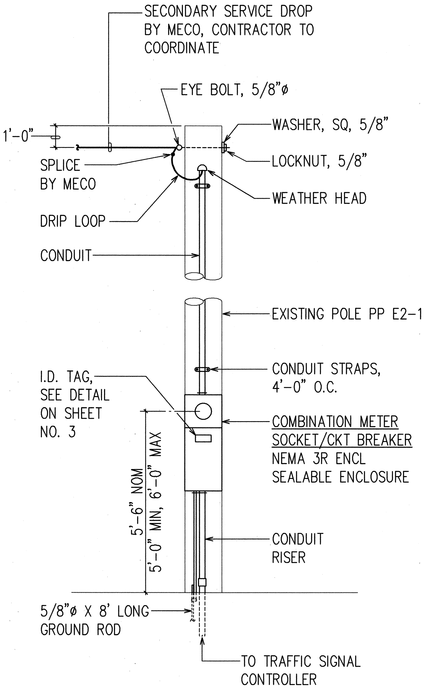
A METER EQUIPMENT ELEVATION E2 NOT TO SCALE
