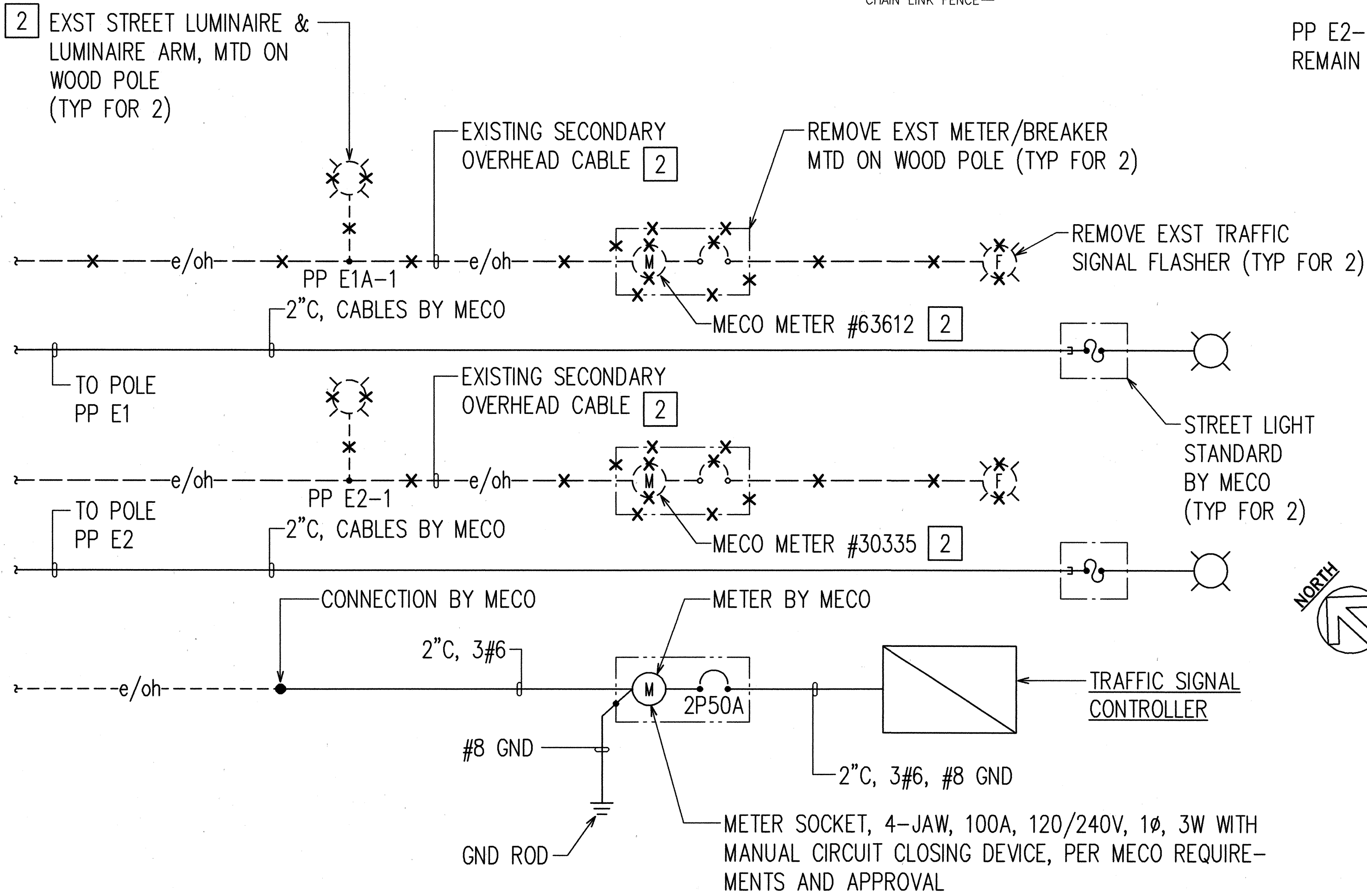
ONE-LINE DIAGRAM
