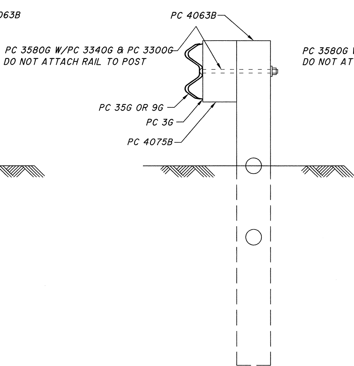
SECTION "C-C" (@ POSTS #4, #6, #8, #9 & #10)
