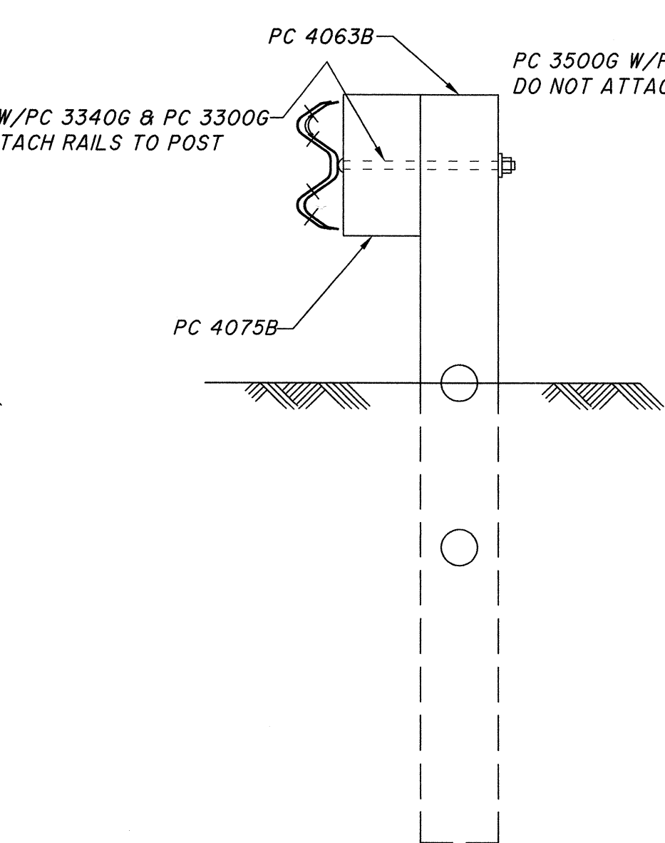
SECTION "B-B" (@ POSTS #3 & #7)
