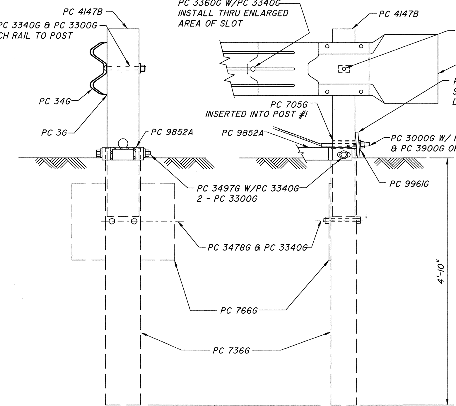
SECTION "A-A" (@ POST #2)
