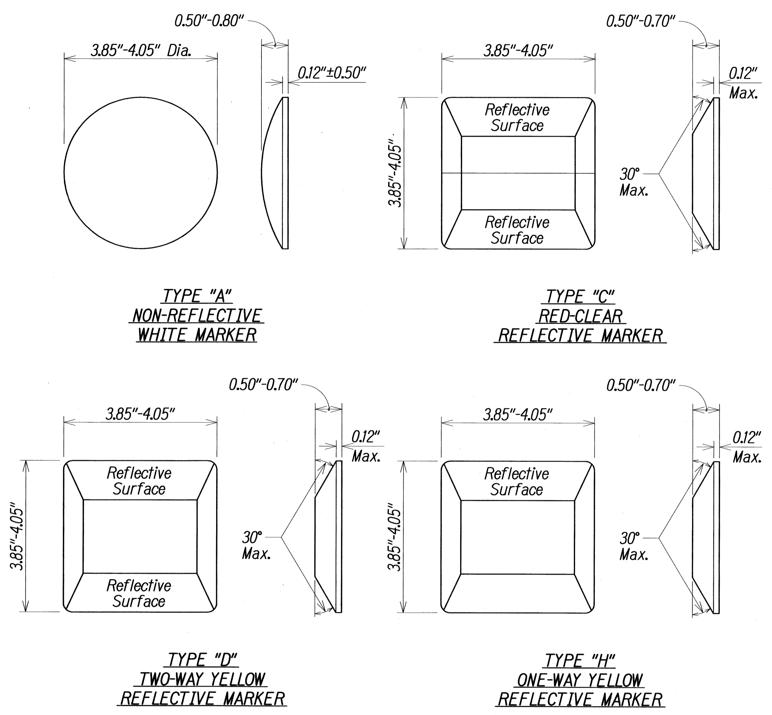
STANDARD RAISED PAVEMENT MARKER DETAILS Not to Scale
