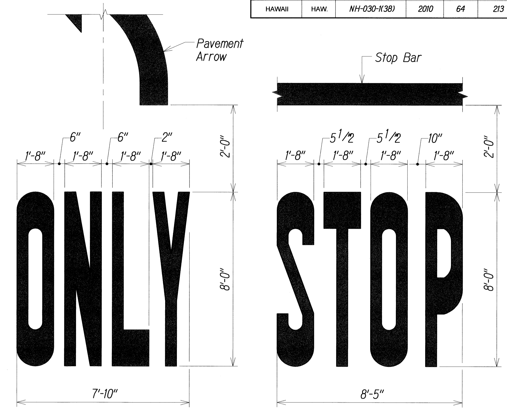
PAVEMENT WORD DETAILS Not to Scale
