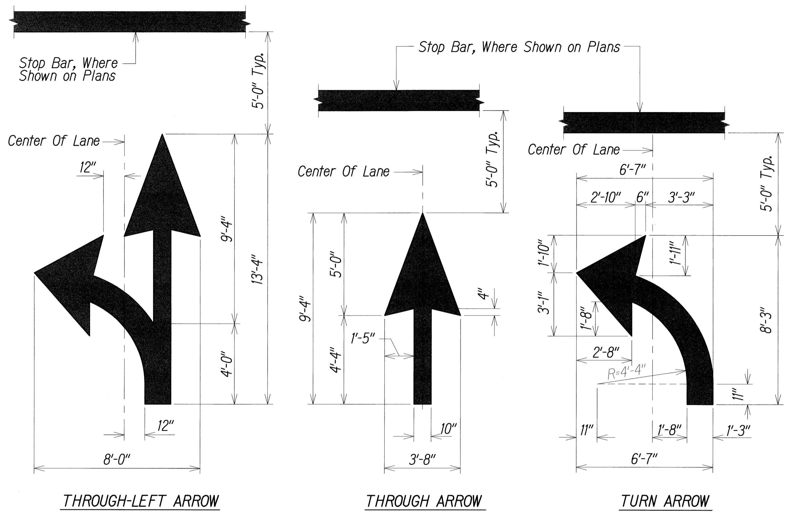
TYPICAL PAVEMENT ARROW DETAILS Not to Scale
