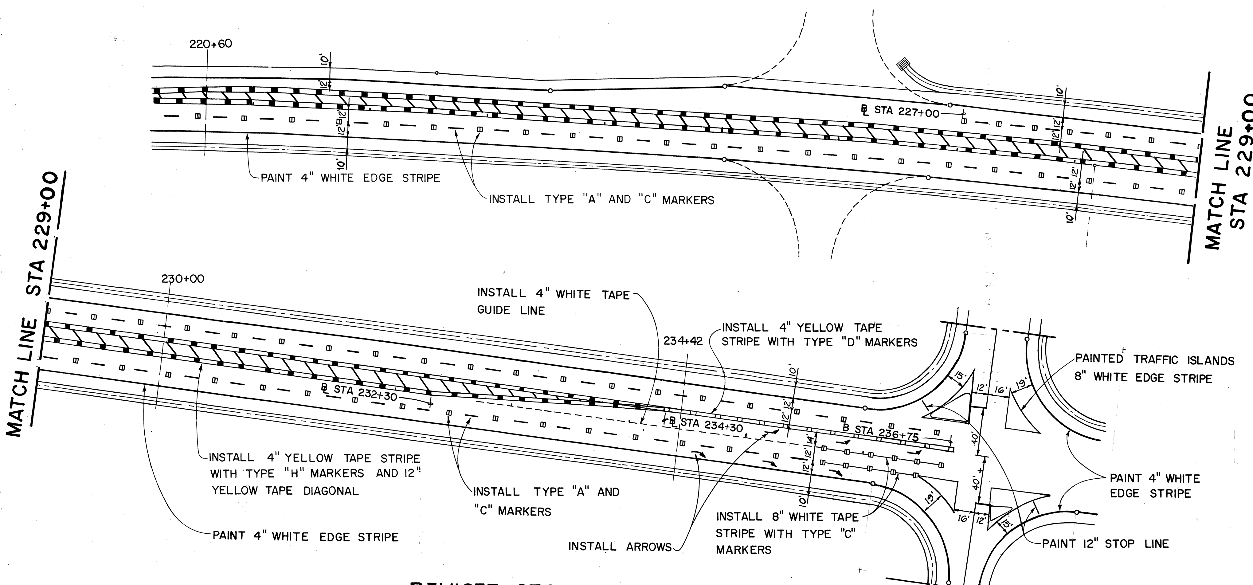
REVISED STRIPING AND PAVEMENT MARKING STA. 220+60 TO 238+00 SCALE: 1" = 50'-0"
