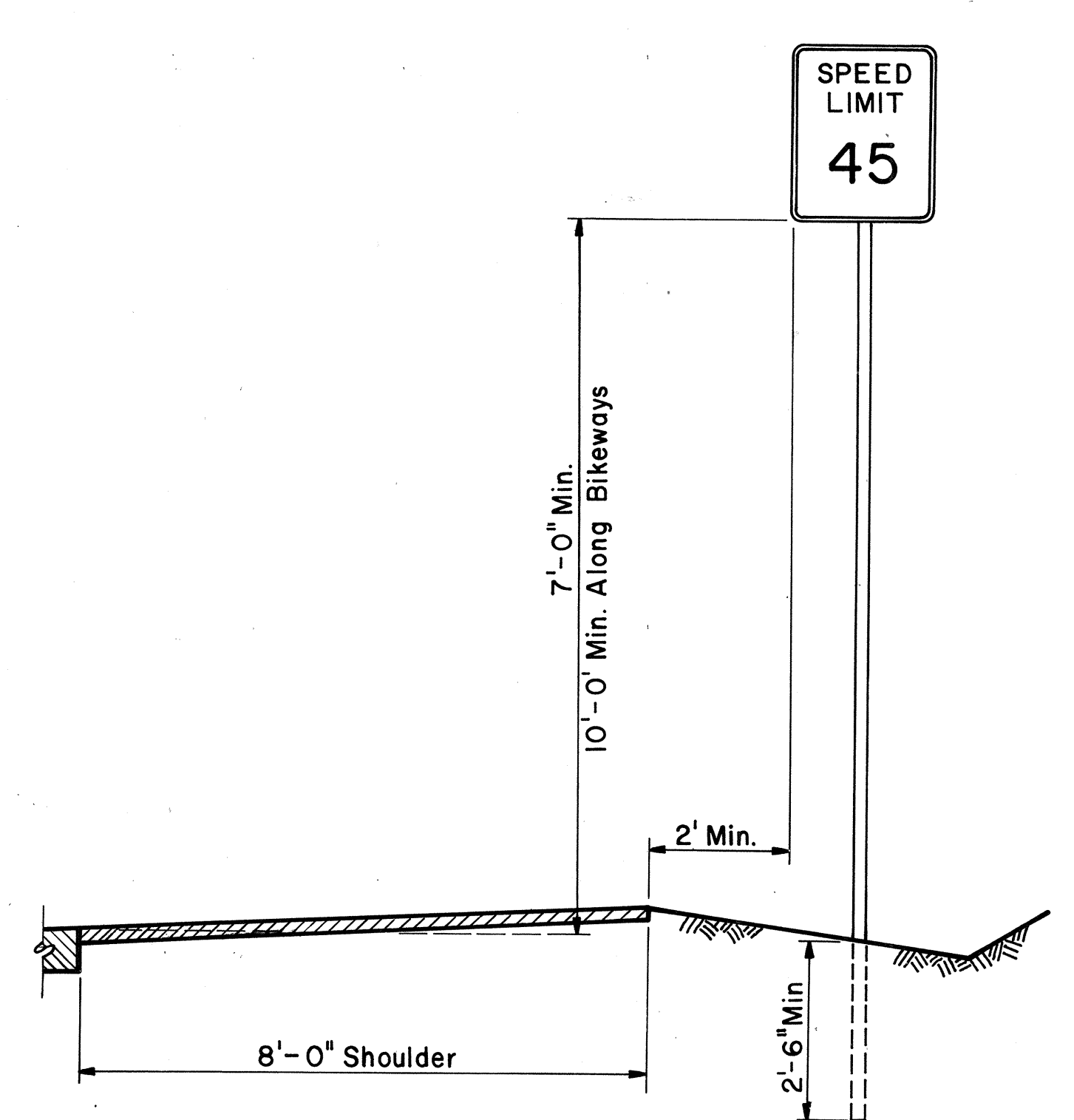
HEIGHT AND LATERAL LOCATIONS OF SIGNS TYPICAL INSTALLATION N.T.S.
