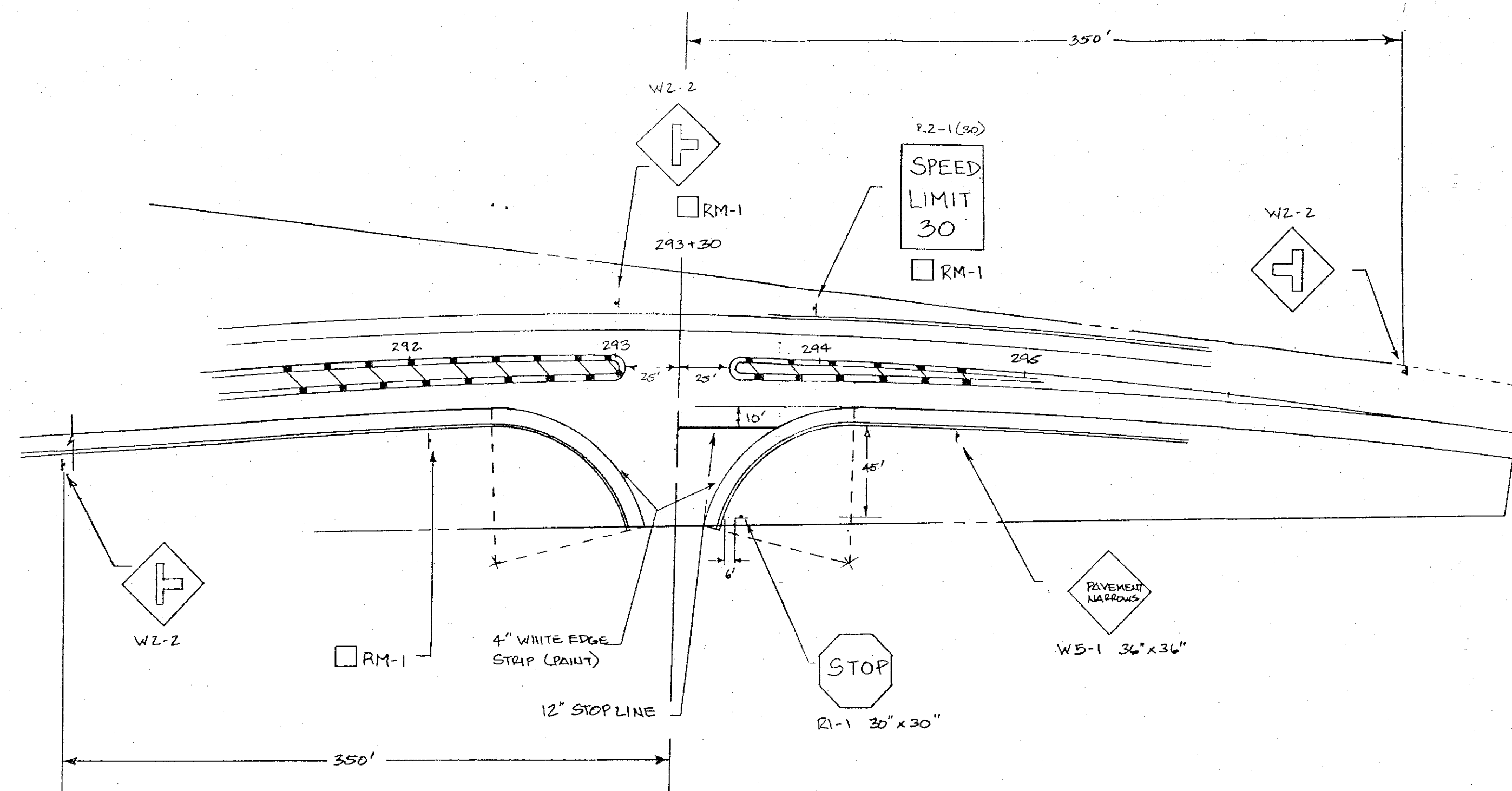
SIGNING and STRIPING PLAN Scale: 1 in. = 50 ft.
