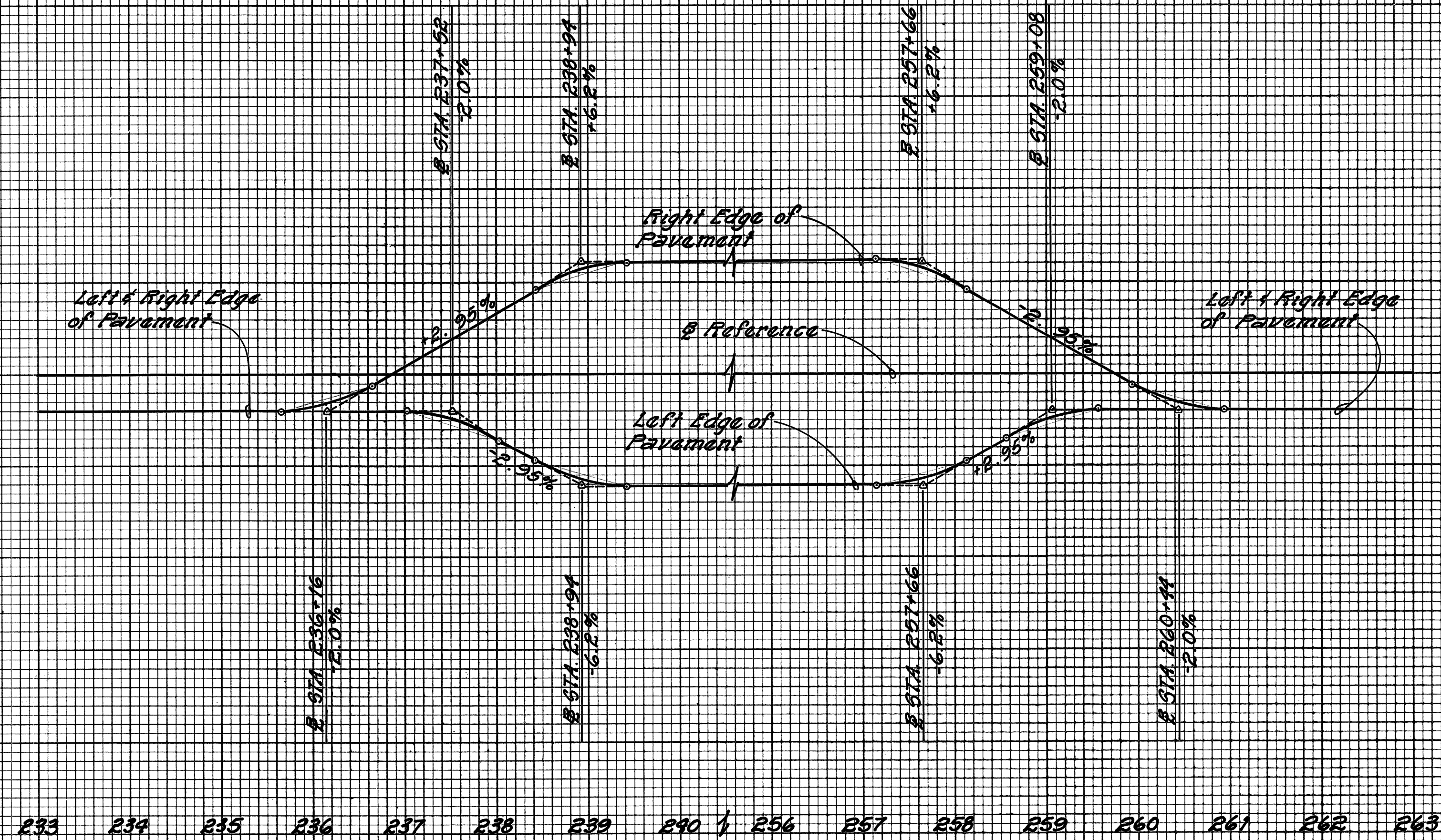
SUPERELEVATION FOR LEFT & RIGHT EDGE OF PAVEMENT
