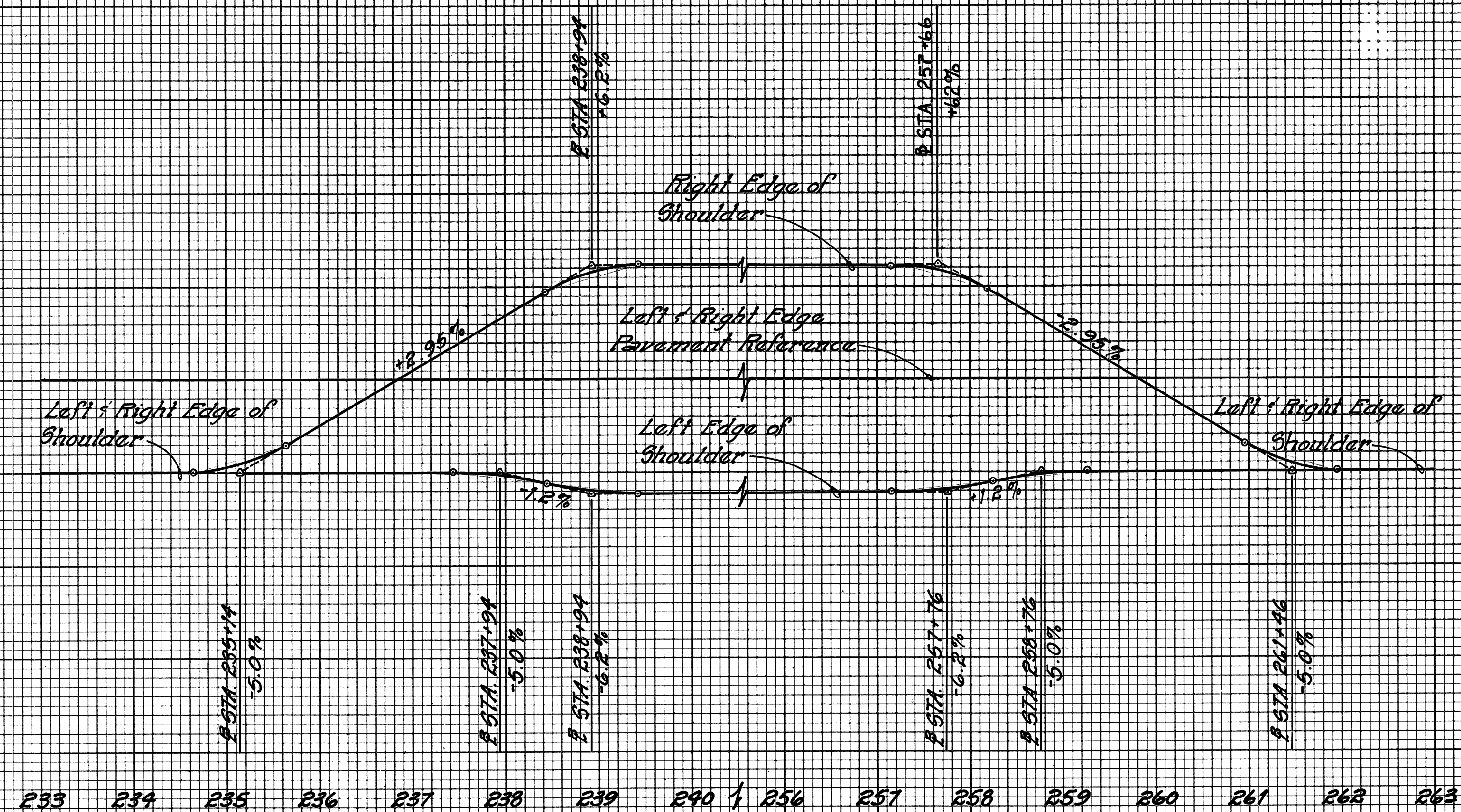
SUPERELEVATION FOR LEFT & RIGHT EDGE OF SHOULDER
