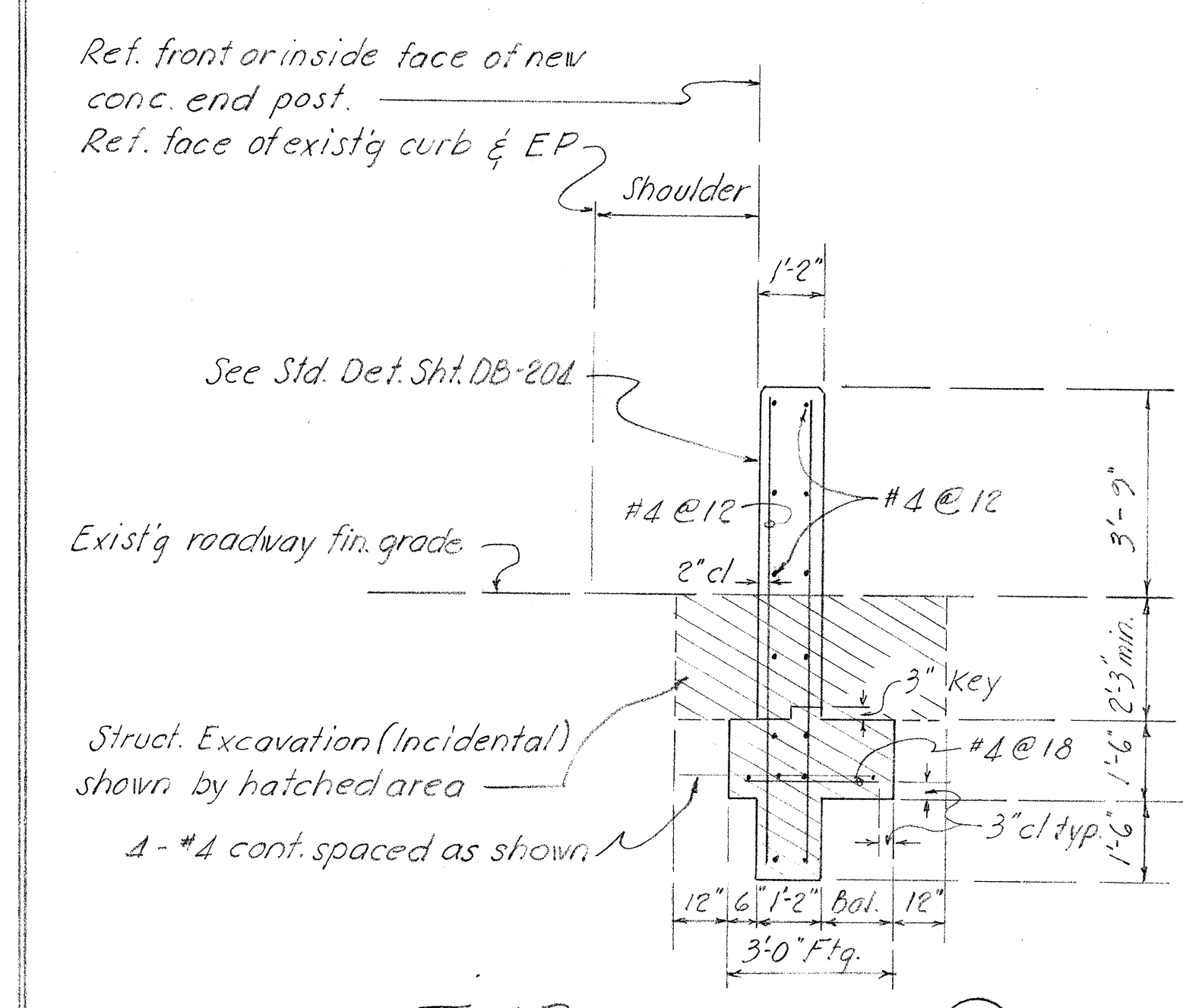
TYP. SECT. Scale: 3/8" = 1'-0"
