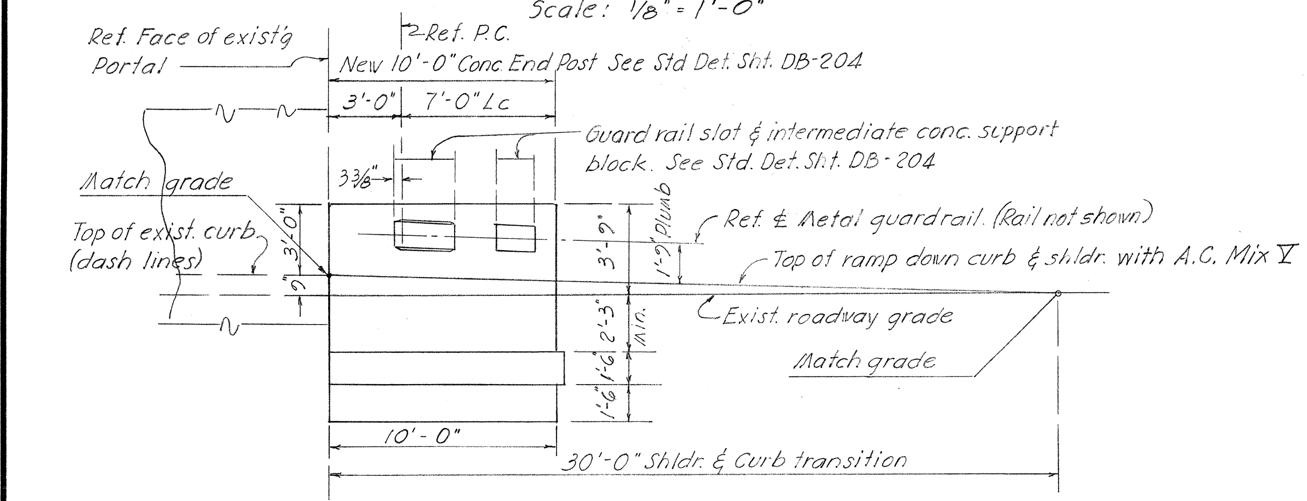
TYP. END POST ELEVATION Scale: 1/4" = 1'-0"
