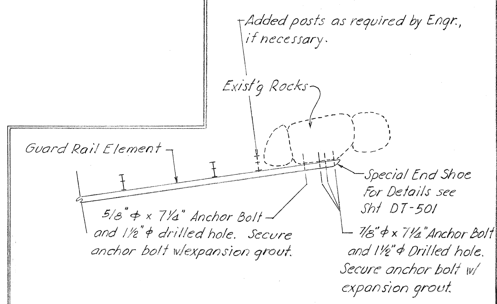
SPECIAL FLARE ANCHOR DETAIL
