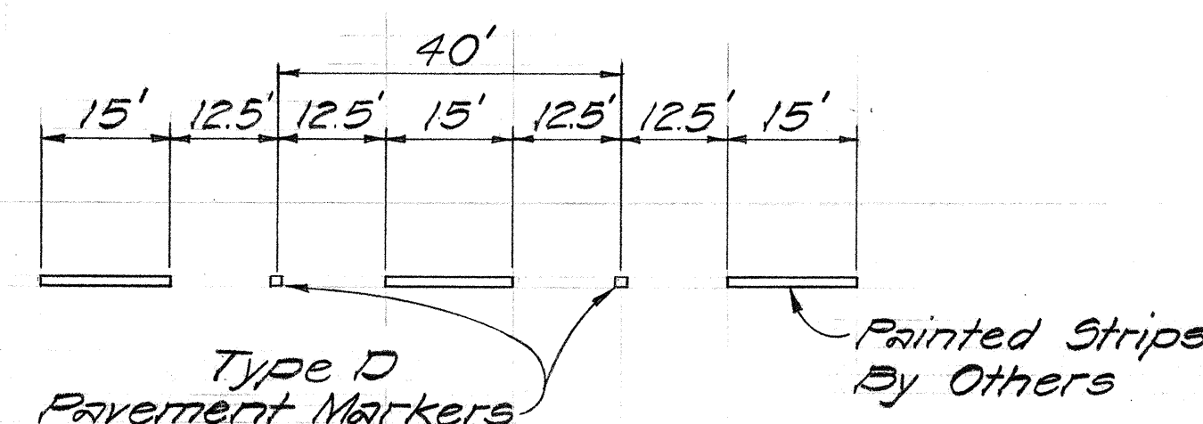
PLAN OF TYPE D PAVEMENT MARKERS Not to Scale
