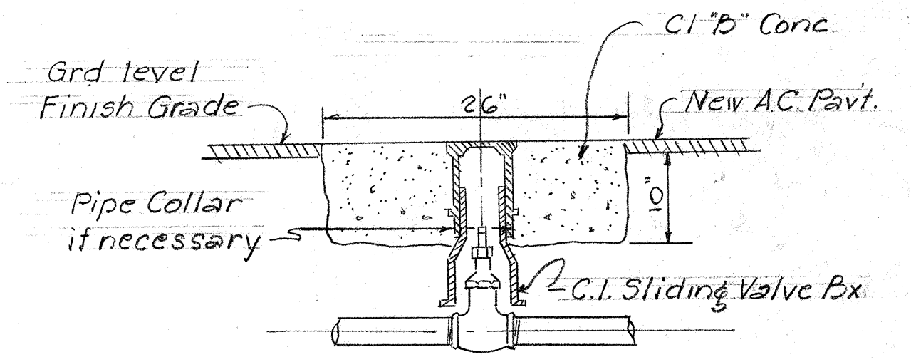
ADJUSTED WATER VALVE BOX
