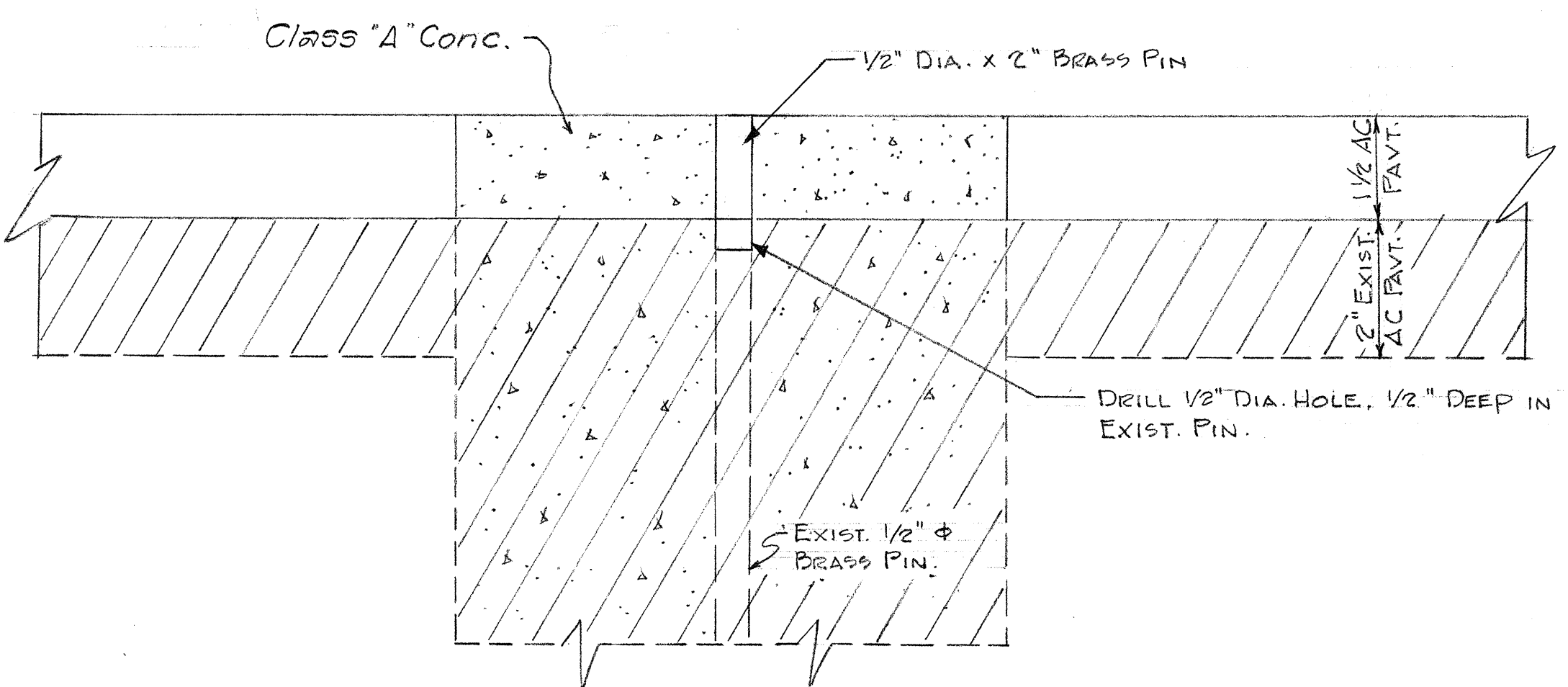
DETAIL OF CENTERLINE MONUMENT SCALE: 1/2" = 1"
