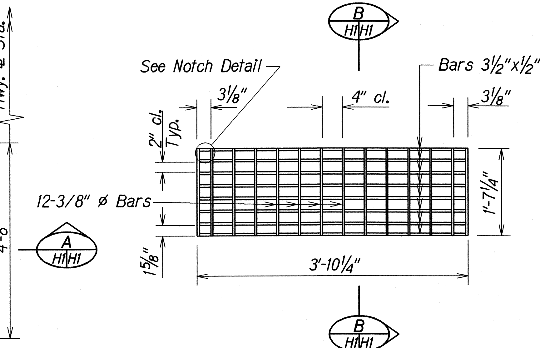
PLAN - GRATE Not to Scale
