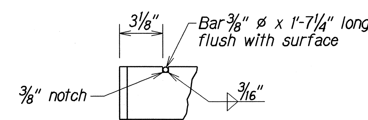
NOTCH DETAIL Not to Scale
