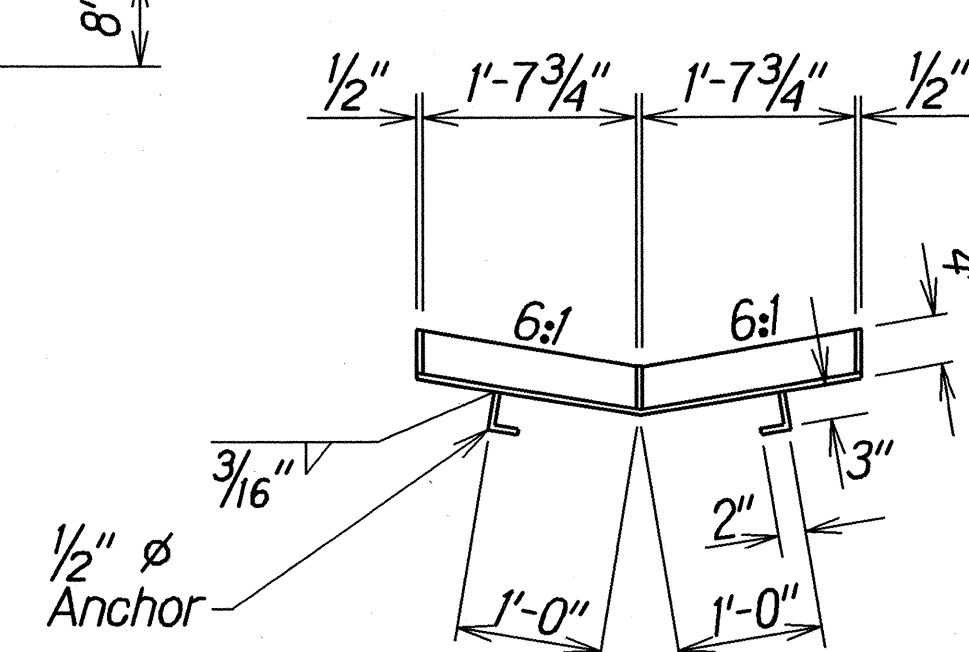
SECTION - FRAME Not to Scale
