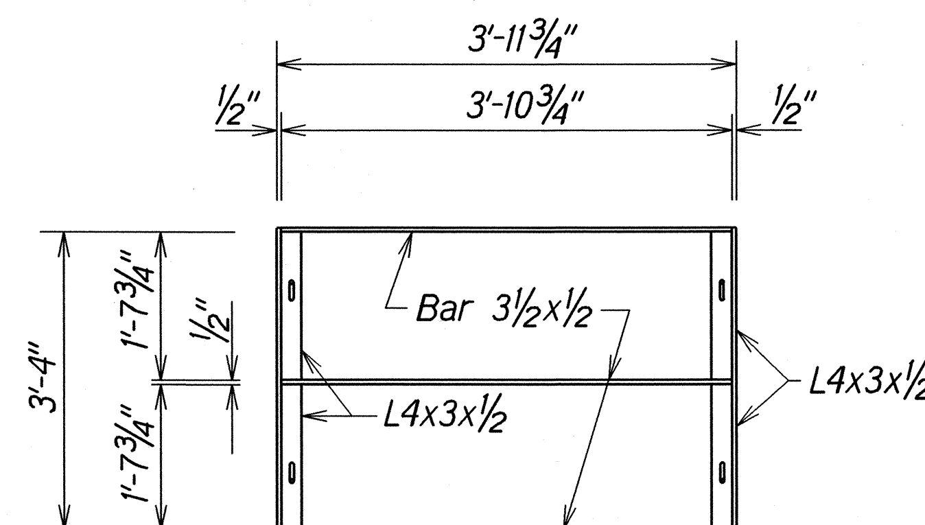
PLAN - FRAME Not to Scale
