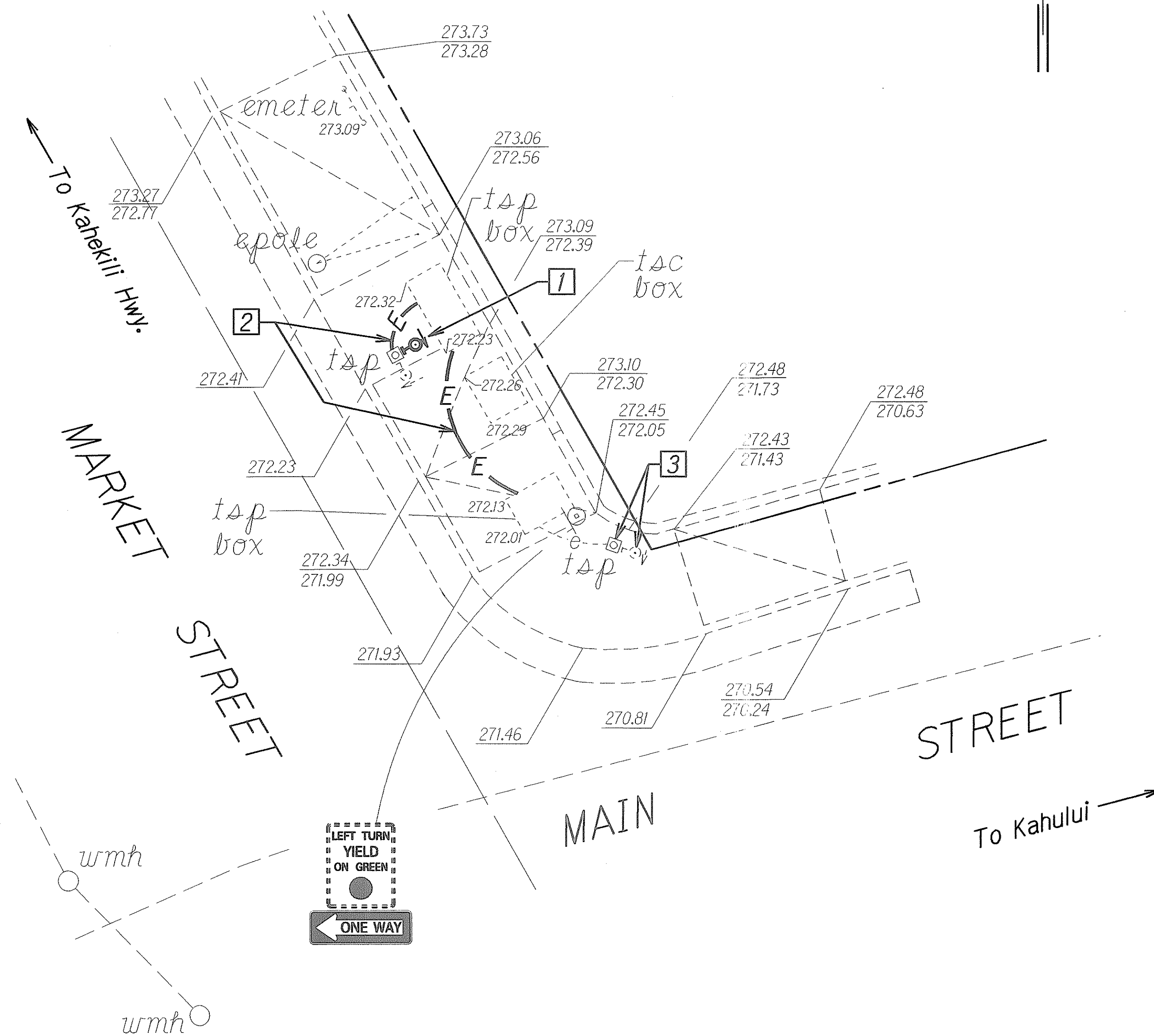
CURB RAMP NO. 10404-3 & -4 DETAILS Scale: 1"= 5'
