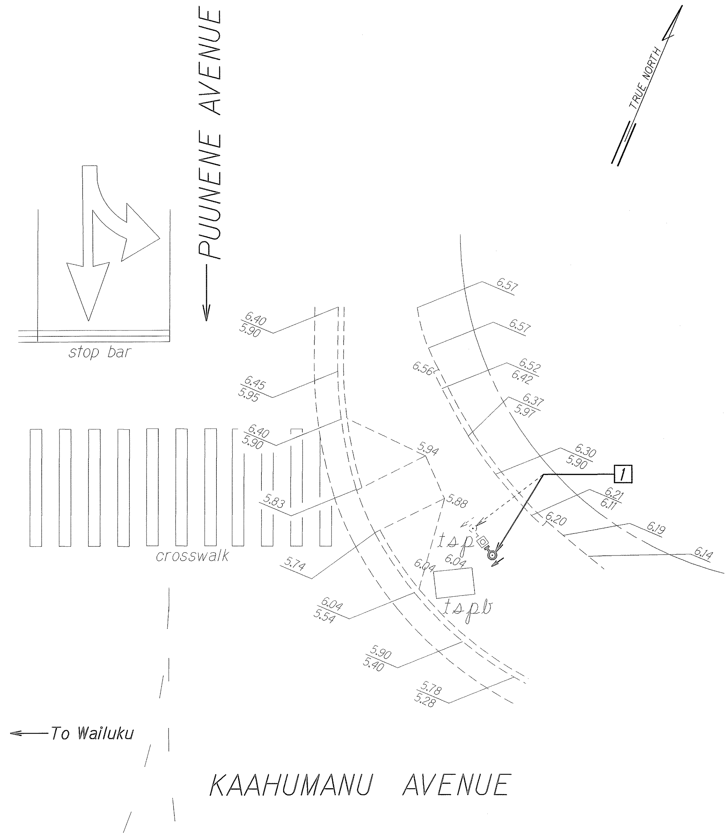
CURB RAMP NO. 12104-2 DETAILS Scale: 1"= 5'
