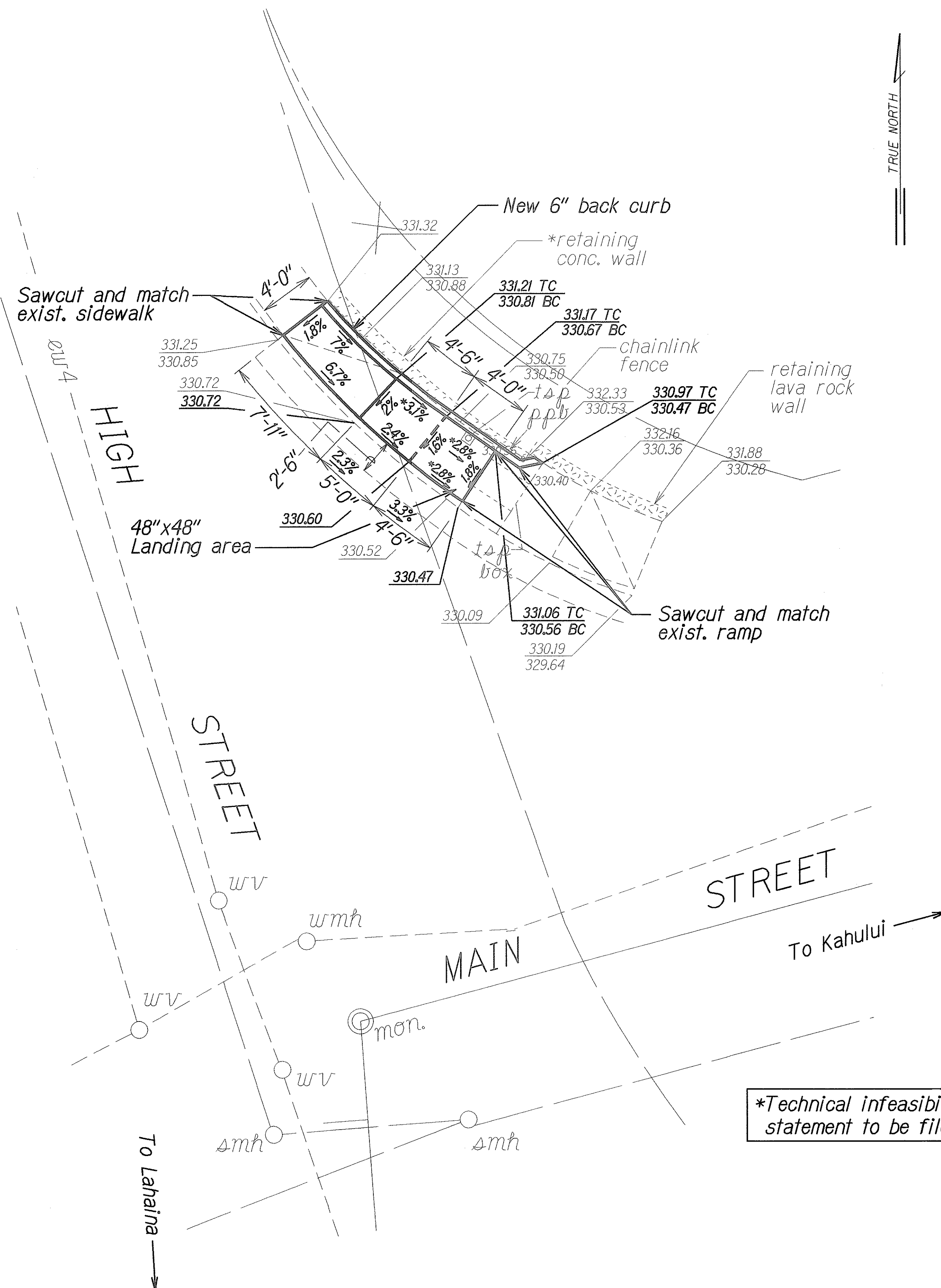
CURB RAMP NO. 10104-4 DETAILS Scale: 1"= 5'
