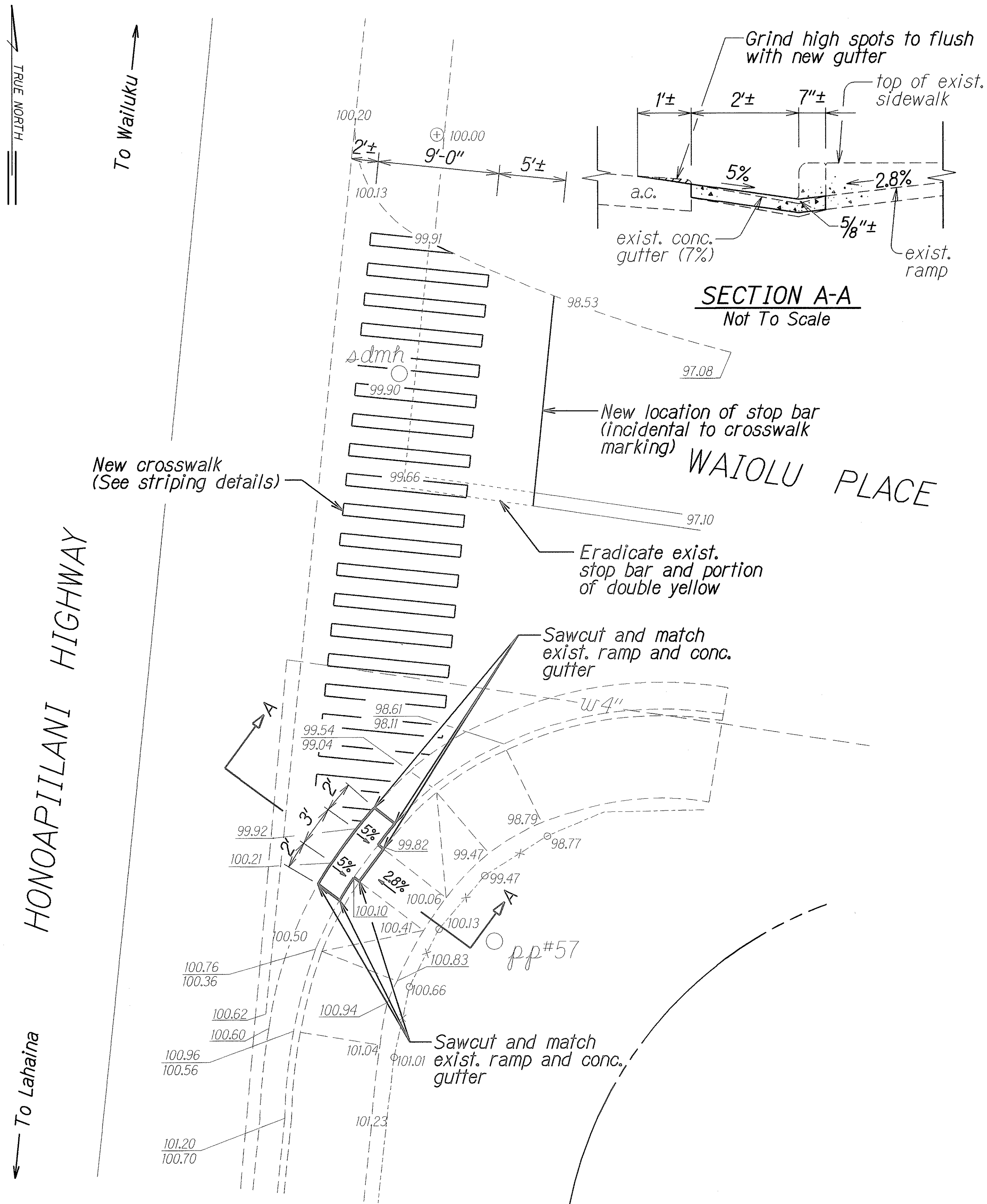
CURB RAMP NO. 31704-1 DETAILS Scale: 1"= 5'
