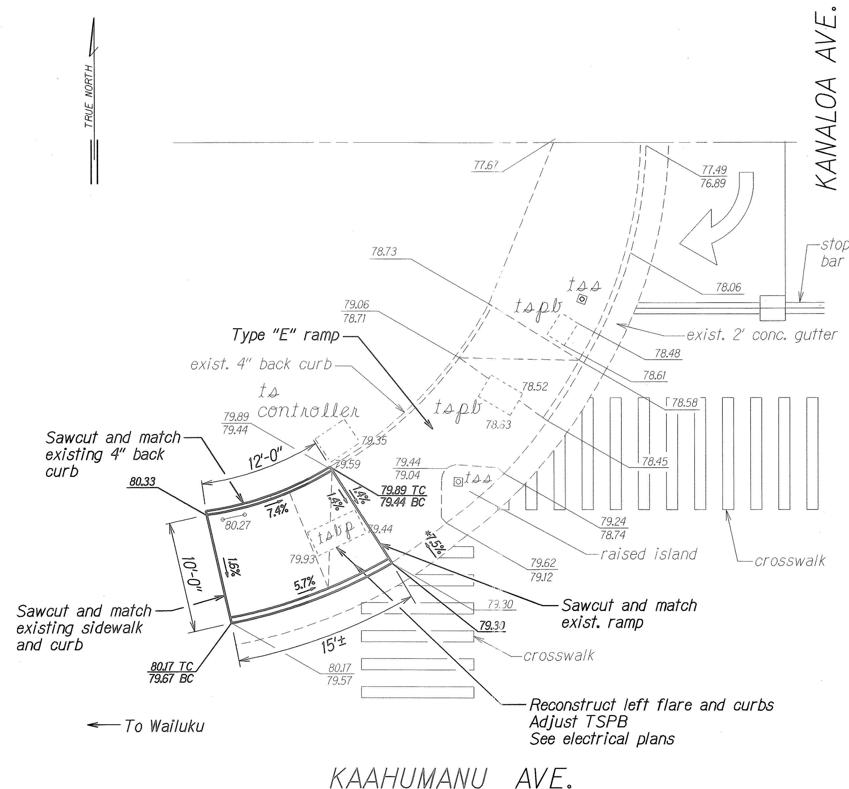
CURB RAMP NO. 11204-1 DETAILS Scale: 1"= 5'
