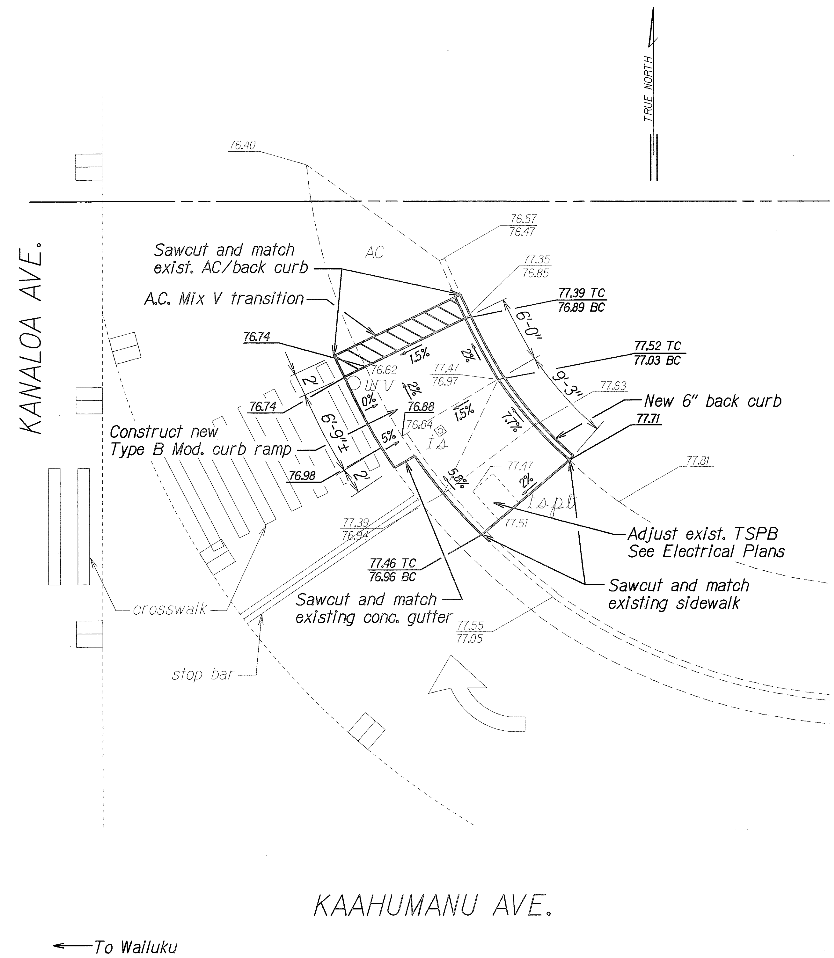
CURB RAMP NO. 11204-5 DETAILS Scale: 1"= 5'
